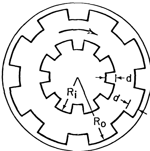
FIG. 1 Schematic of Experimental Magnetron Conducting Boundary Configurations.
