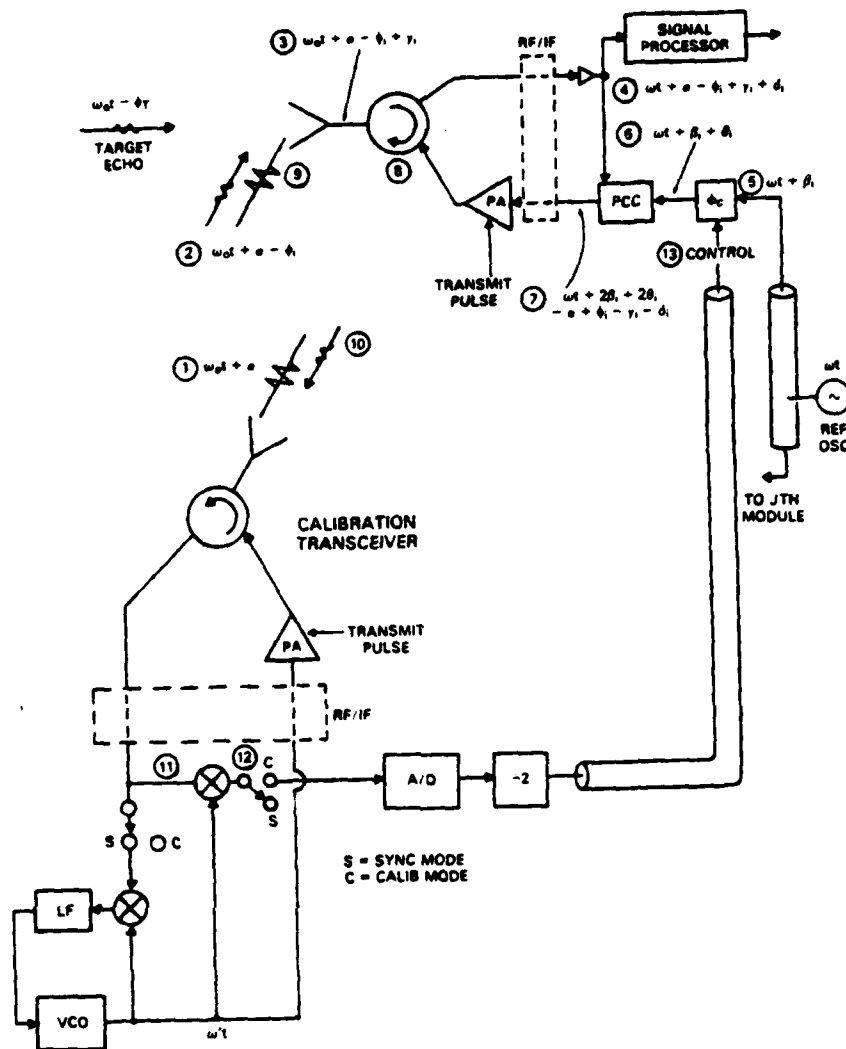
Fig. 10. i th module of distorted array.
