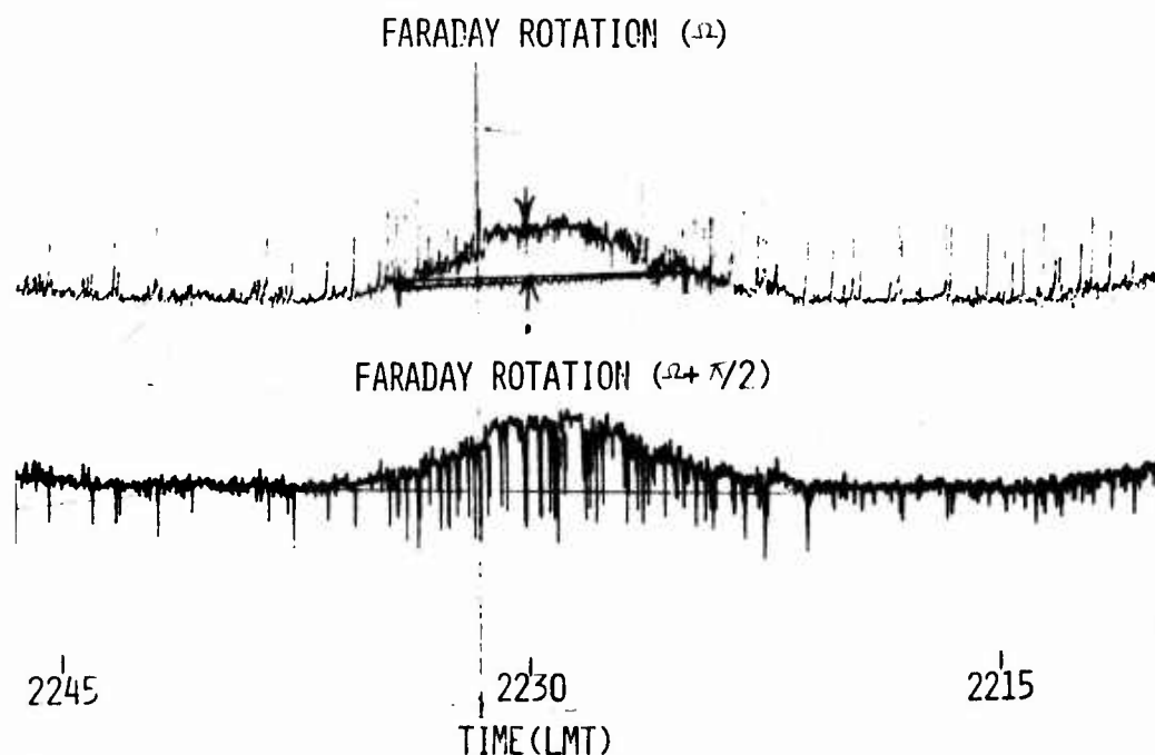
Fig. 6. Original record for September 19, 1978, from Natal using SMS 1 transmissions, showing an isolated enhancement.
