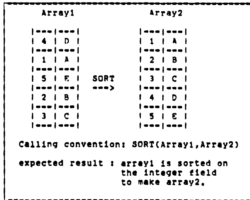
Figure 9. Quicksort
