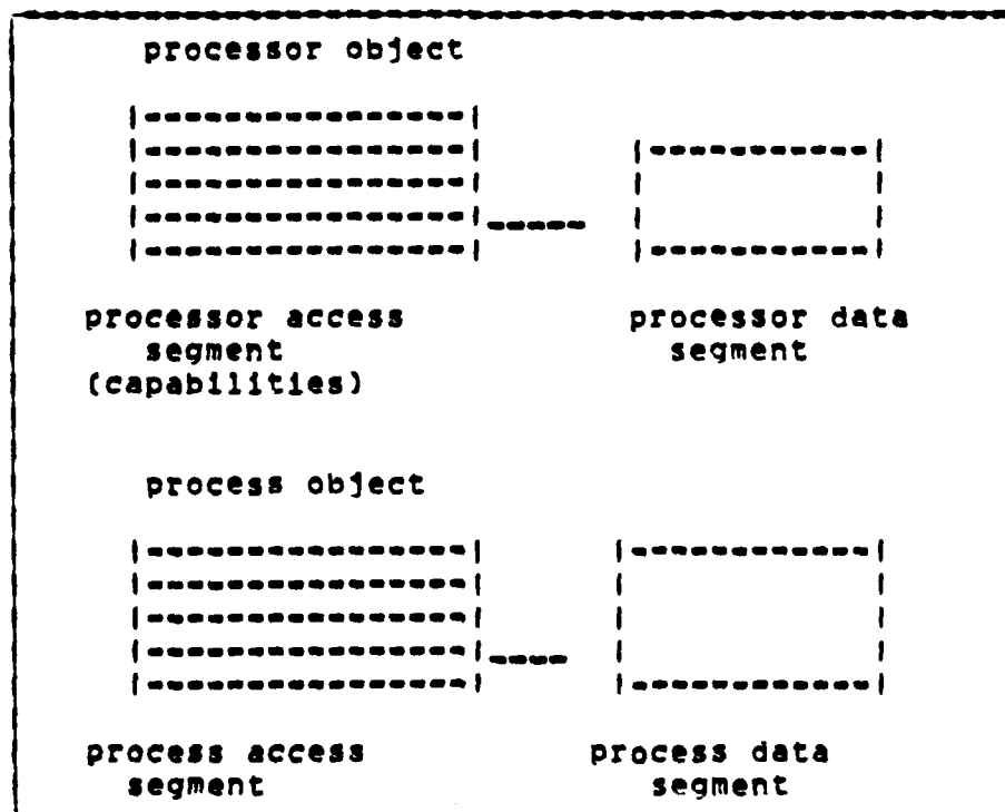
Figure 2. Object Representation
