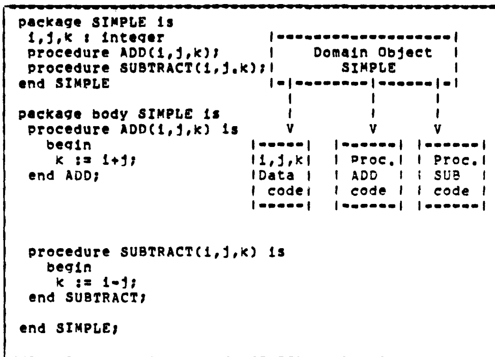
Figure 5. ADA Package and IAPX-432 Object Correspondence
