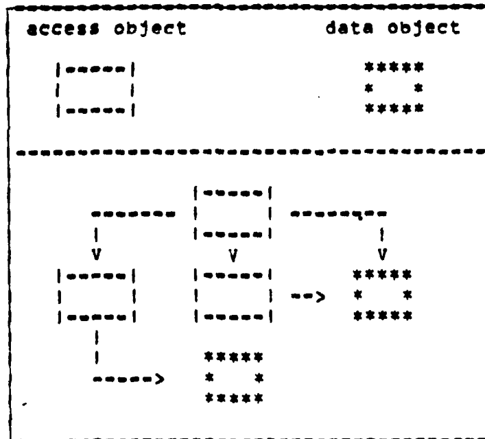
Figure 3. ADA-432 Object Types
