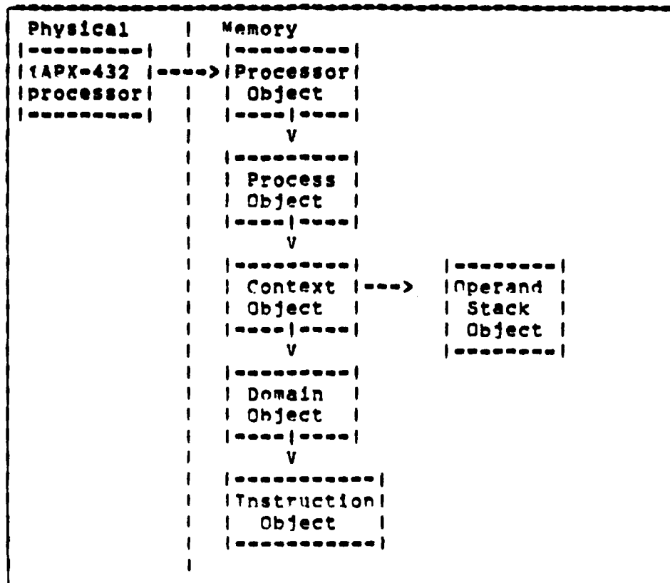
Figure 1. Hardware Recognized Objects
