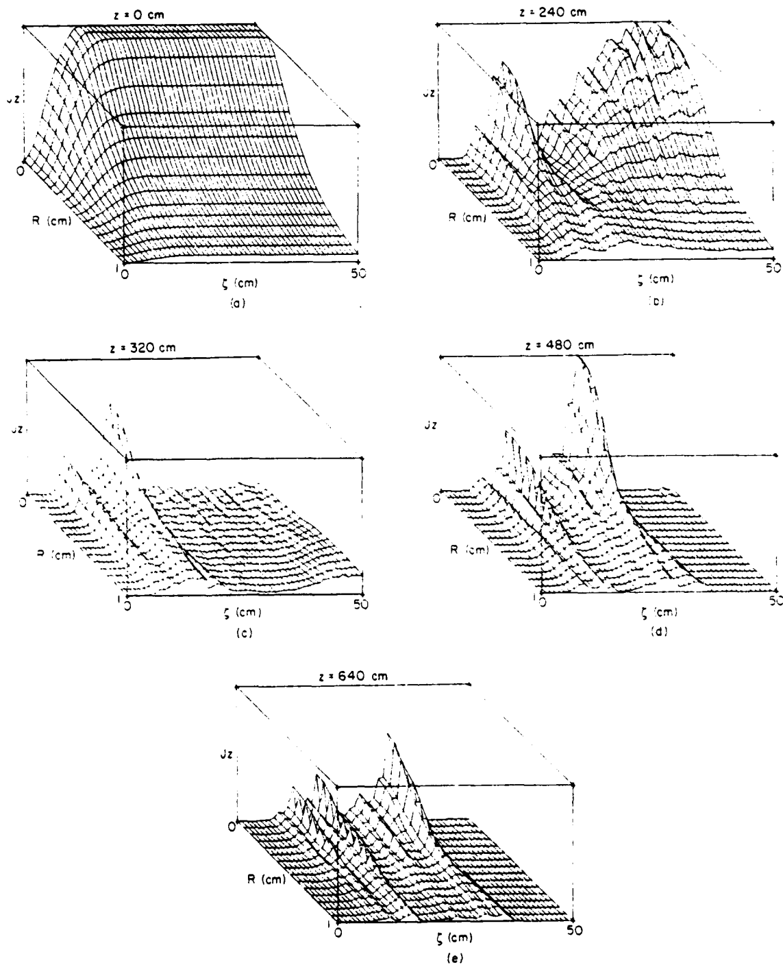
Fig. 5 — Beam current density contours J_b(r, \zeta) for various values of z , for the same case as Fig. 1
