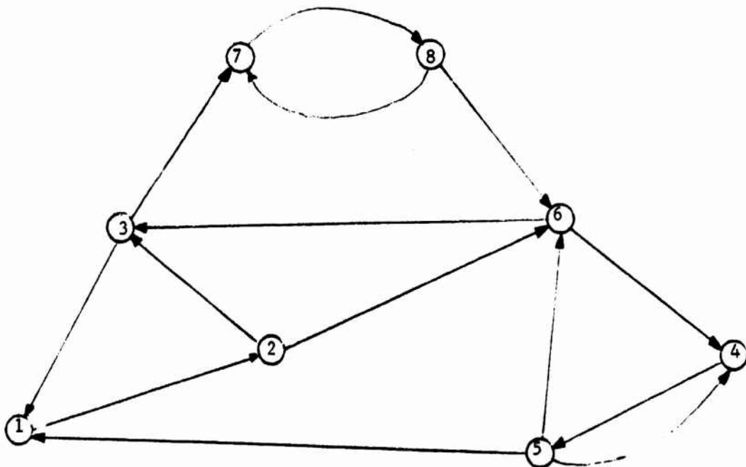
Fig. 6. Graph G_0 after bounding procedure 3
