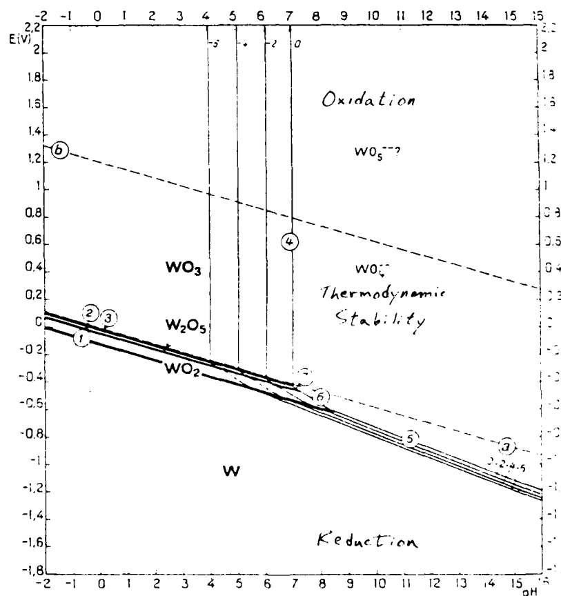
Figure 1. Potential-pH equilibrium diagram for the system tungsten-water at 25°C.
