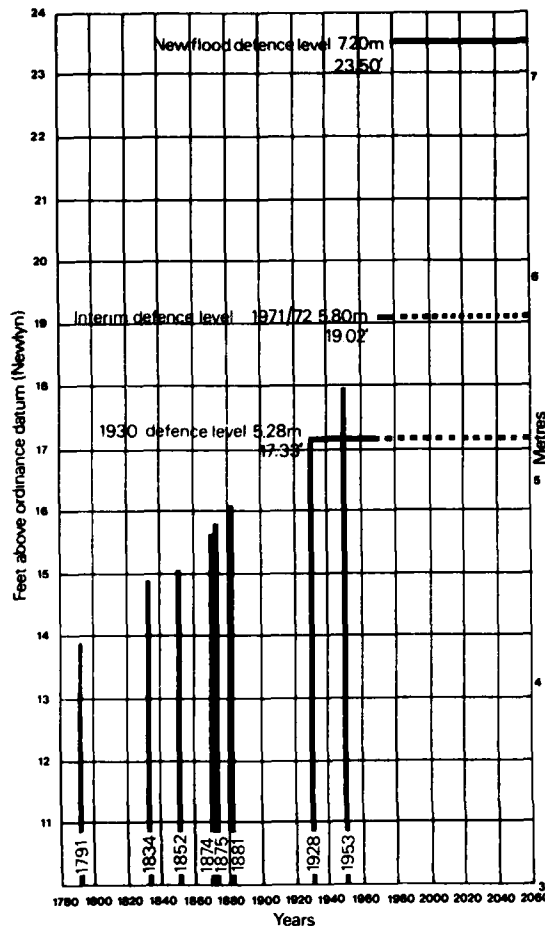
Figure 2. Increasing high tide levels and defense levels at London Bridge.
