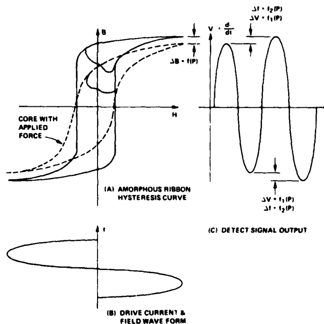
FIGURE 4 SIGNAL PROCESSING SIN MAGNETOELASTIC RIBBONS
