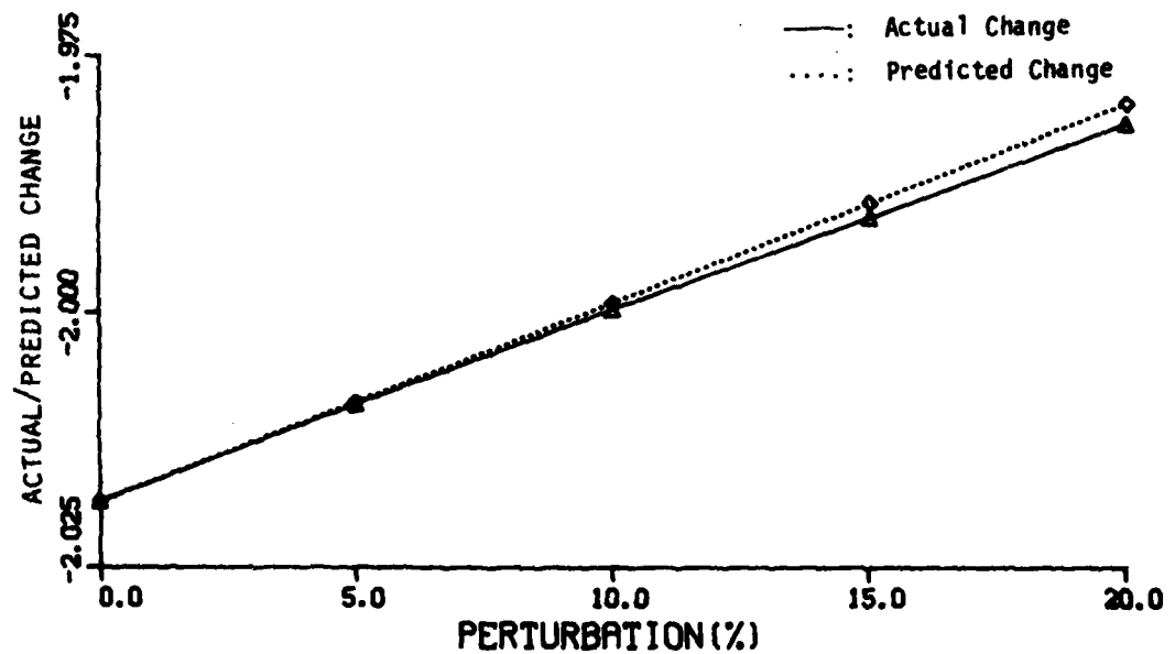
Figure 13. Accuracy test of design sensitivity of rear wheel penetration constraint on bump road ( \psi_{10} )
