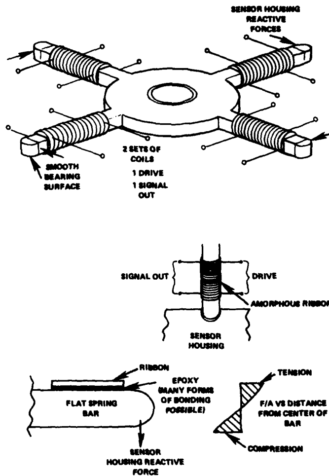
FIGURE 6 TORQUE SENSOR
