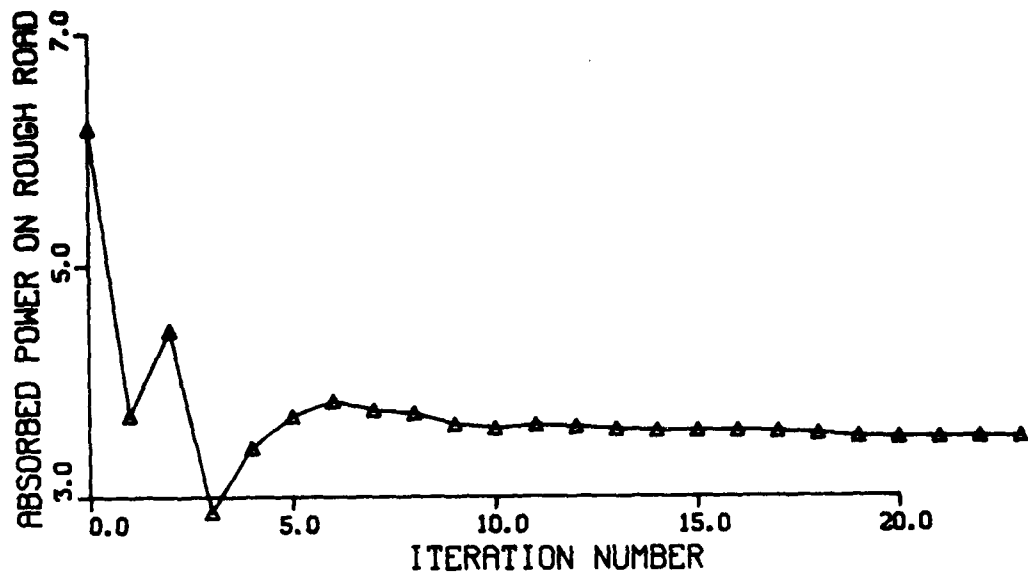
Figure 14. History of absorbed power constraint ( \psi_1 )
