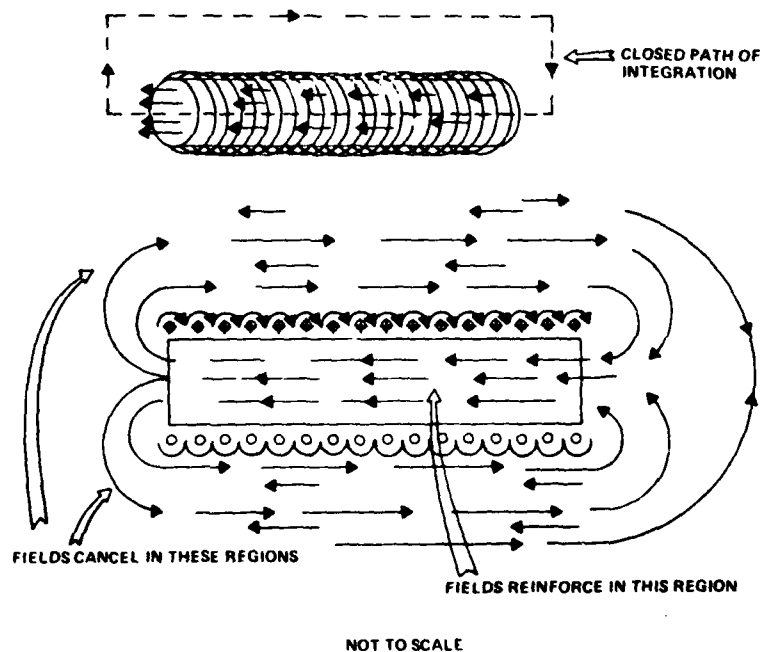
FIGURE 3 H&B FIELDS IN THE MAGNETOSTRICTIVE ROD
