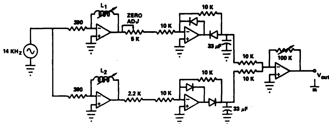
FIGURE 5 THE SEPARATELY EXCITED OSCILLATOR
