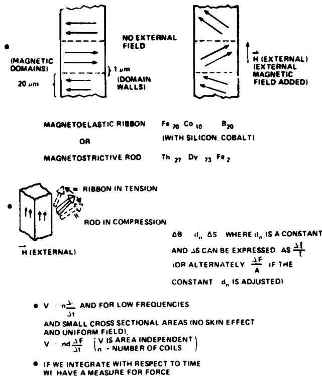
FIGURE 2 HOW THE MATERIALS ACT AS FORCE SENSORS
