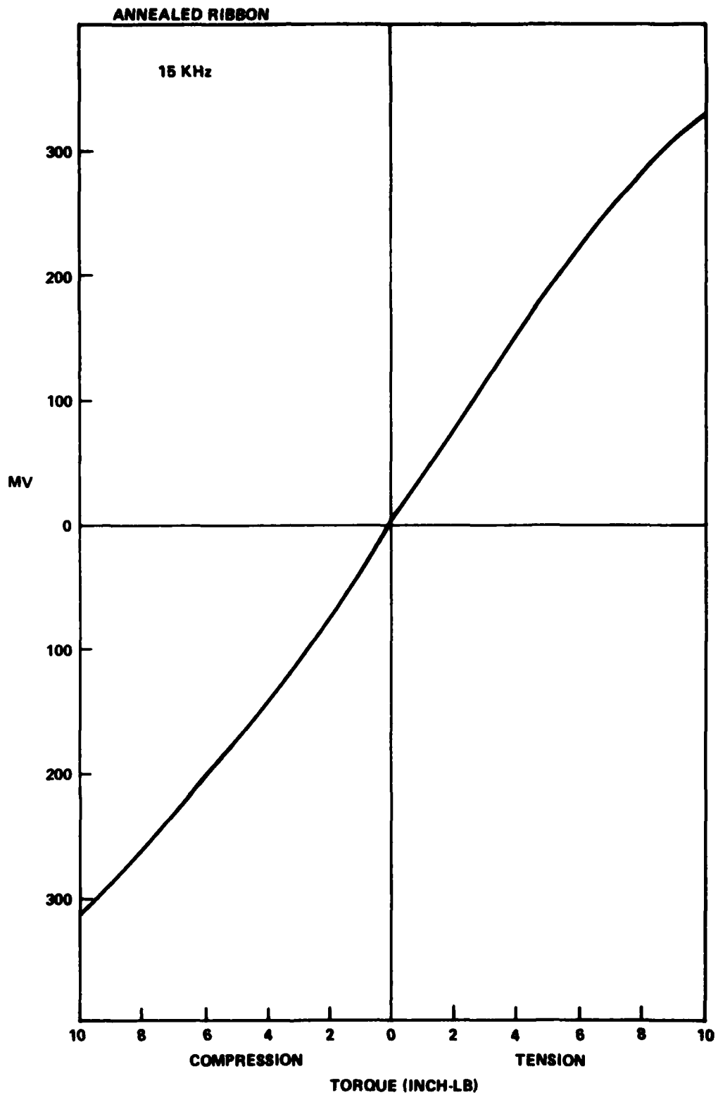
FIGURE 7 LINEARITY RESULTS
