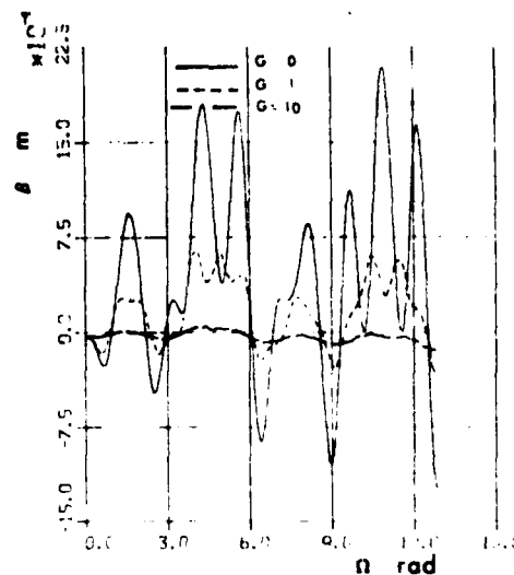
Figure 10. Four-Mode Solu- tion for Different Gain Factors
