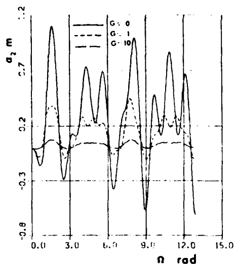
Figure 7. Effect of the Gain on the Second Mode of Link BP
