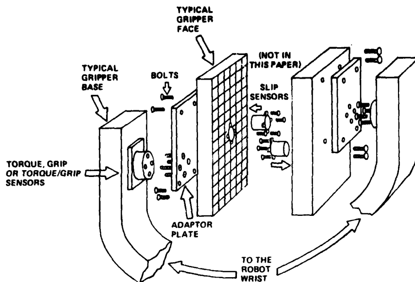
FIGURE 1 RETROFIT TECHNIQUE
