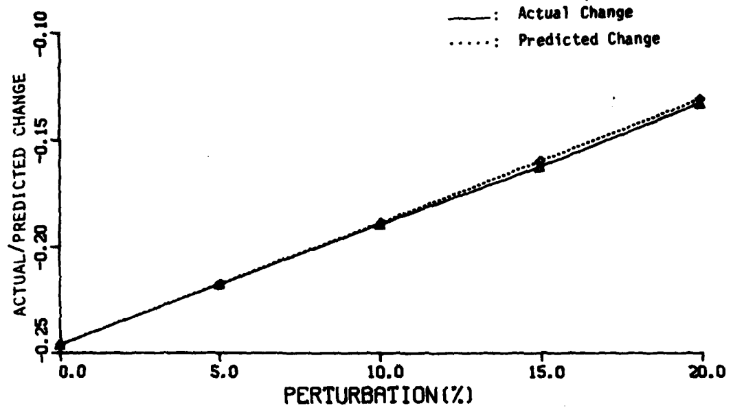
Figure 12. Accuracy test of design sensitivity of rear wheel hop constraint on bump road ( \psi_9 )
