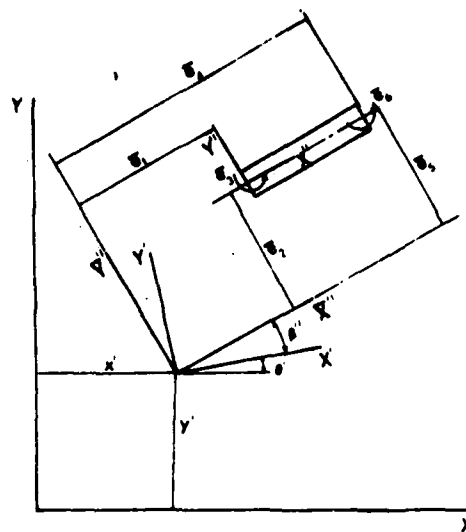
Figure 2. Two Dimensional Beam Element
