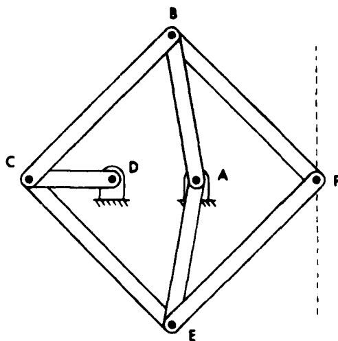
Figure 3. Peaucillier Lipkin Mechanism
