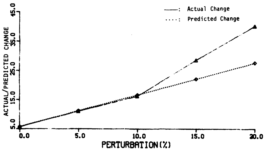
Figure 7. Accuracy test of design sensitivity of peak acceleration constraint on bump road ( \psi_4 )
