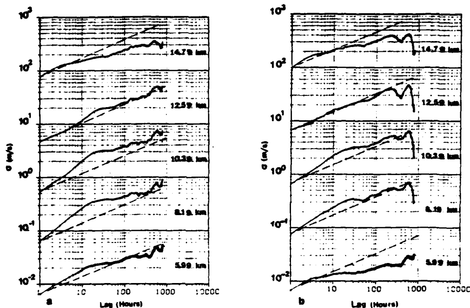
FIG. 3. (a) The variability of the zonal wind as a function of the time lag. The variability is defined in the text. Curves at successive altitudes have been multiplied by a factor of 10 to separate them on the graph. The vertical axis labeling is correct for the variance at 10.39-km altitude. (b) As in (a) but for the meridional wind component.
