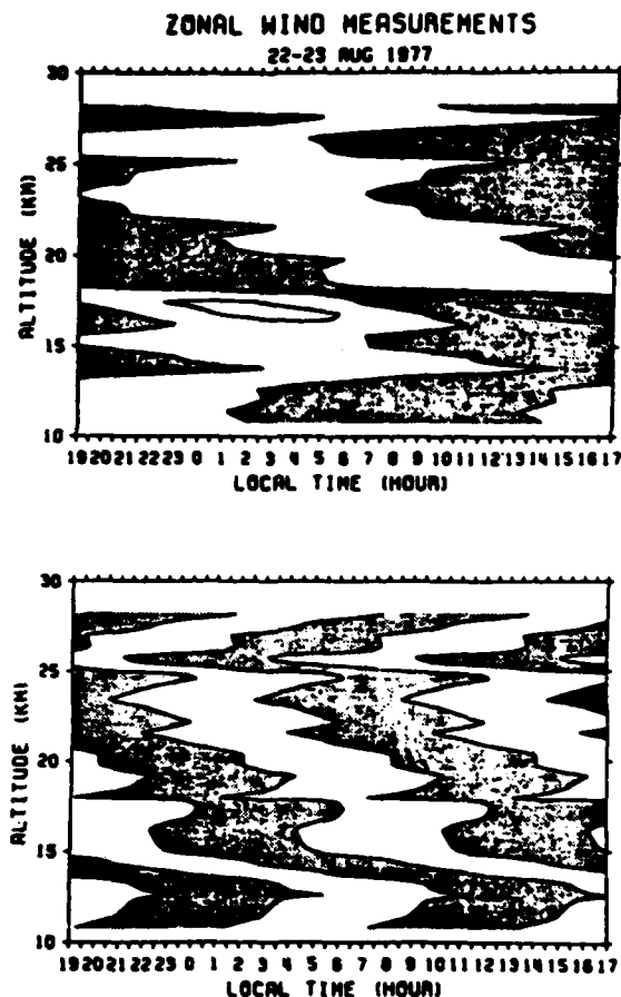
FIG. 10. Diurnal and semi-diurnal tidal components measured by Fukao et al. (1980) at Arecibo, Puerto Rico. The velocity time series were filtered to exclude everything but the particular frequency component of interest. The tidal components show downward phase progression and upward energy propagation in the lower stratosphere.
