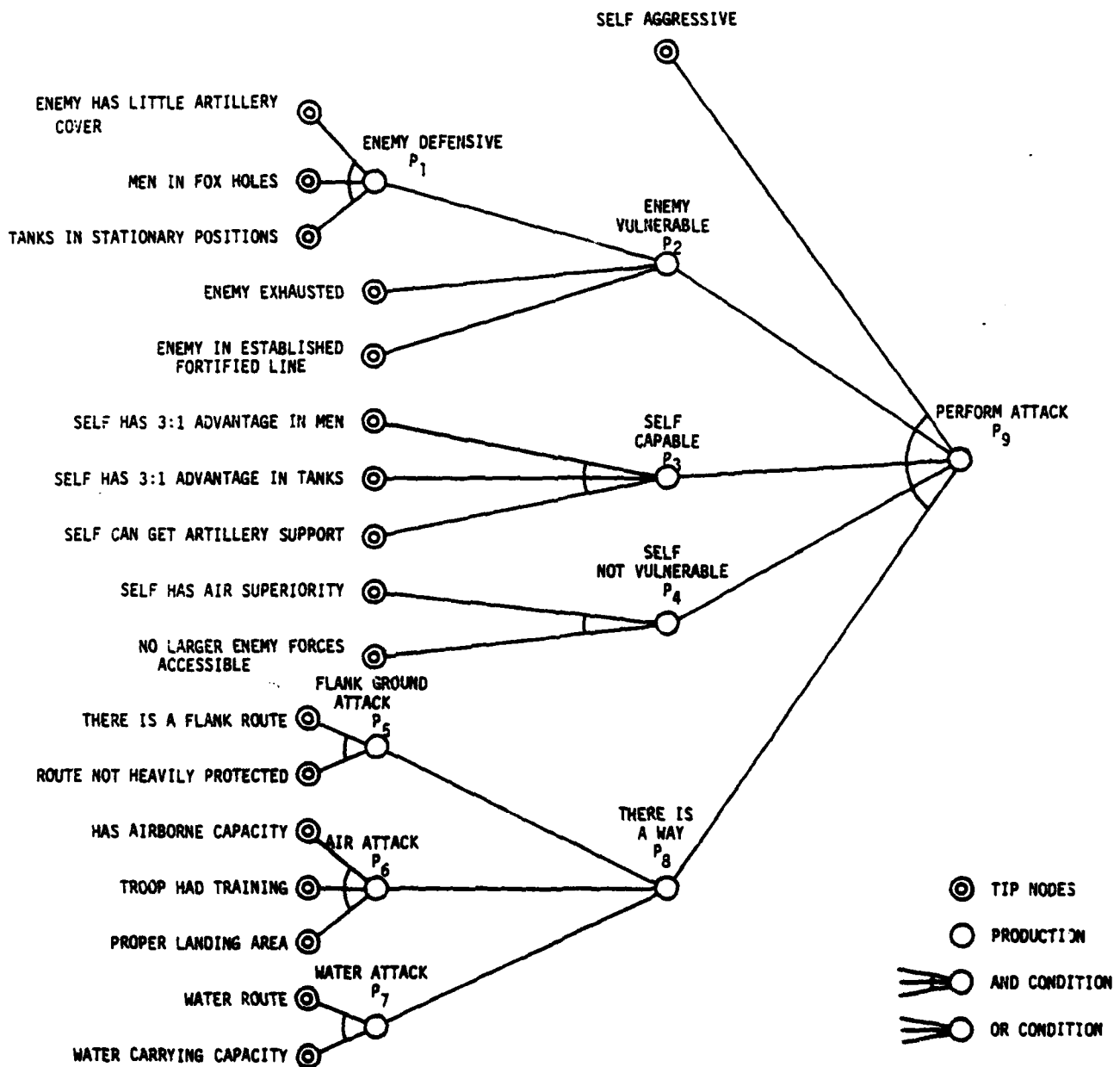
FIGURE 3-1. AND/OR GRAPH
