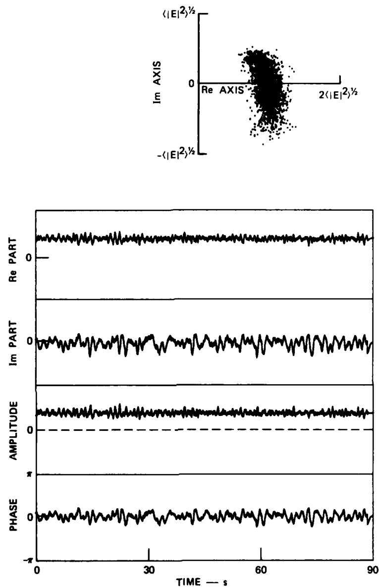
FIGURE 3 THE SCATTER COMPONENT (containing intensity and phase fluctuations with Fourier periods shorter than 2.5 s) OF THE COMPLEX-SIGNAL SCINTILLATION PRESENTED IN FIGURE 1
