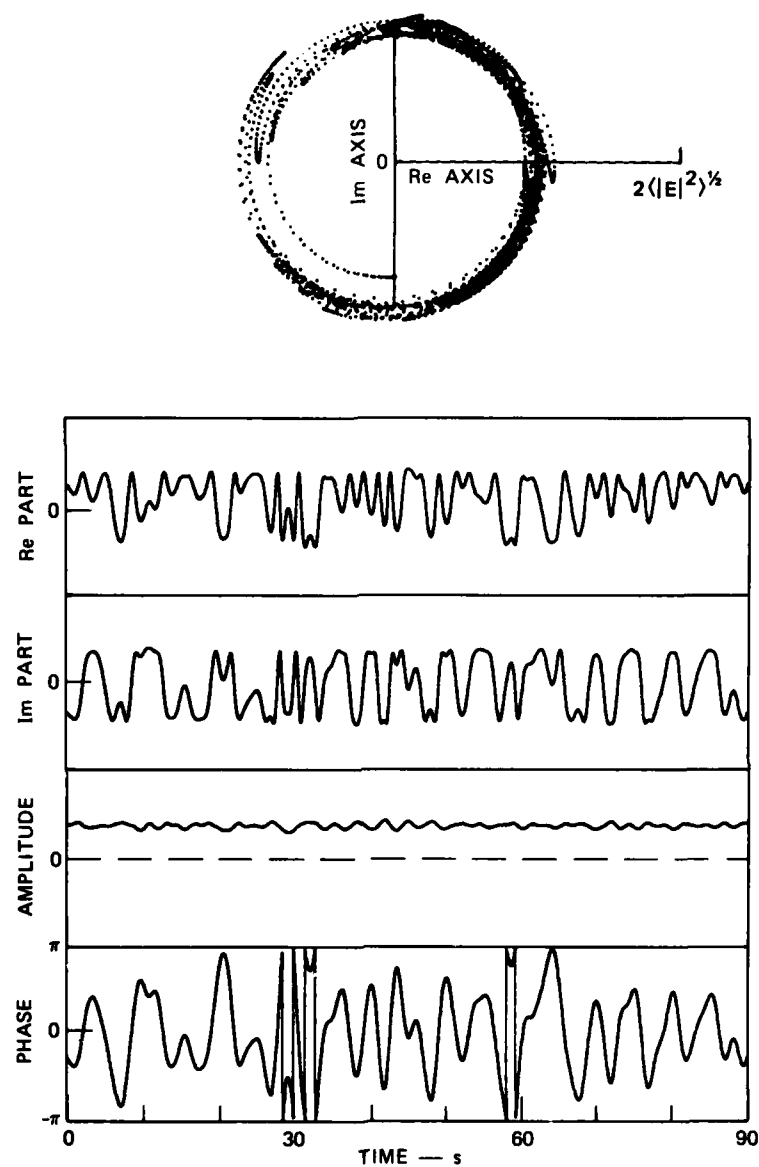
FIGURE 2 THE FOCUS COMPONENT (containing intensity and phase fluctuations with Fourier periods shorter than 2.5 s) OF THE COMPLEX-SIGNAL SCINTILLATION PRESENTED IN FIGURE 1
