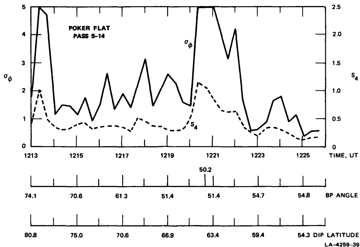
FIGURE 6 STANDARD SUMMARY DISPLAY OF VHF (138 MHz) INTENSITY AND PHASE SCINTILLATION INDICES ( S_4 and \sigma_{\phi} , respectively) OBSERVED IN ALASKA ON A PARTICULAR SATELLITE PASS UNDER CONDITIONS APPROXIMATED BY THE INPUT CONDITIONS FOR THE CALCULATION ILLUSTRATED IN FIGURE 5
