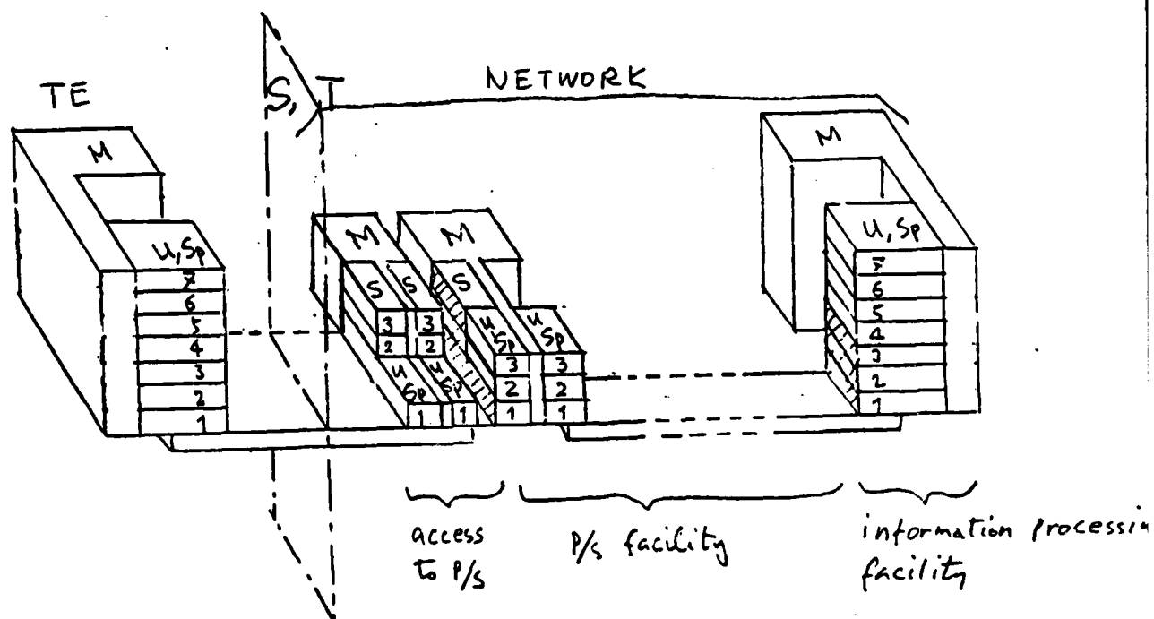
Fig. 6B ISDN Protocol Reference Configuration (Access to HLF - P/S via B-channel)
