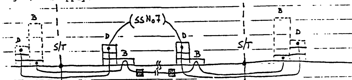
Fig. 7 Protocol model for 64 kbit/s circuit-switched Bearer Service
