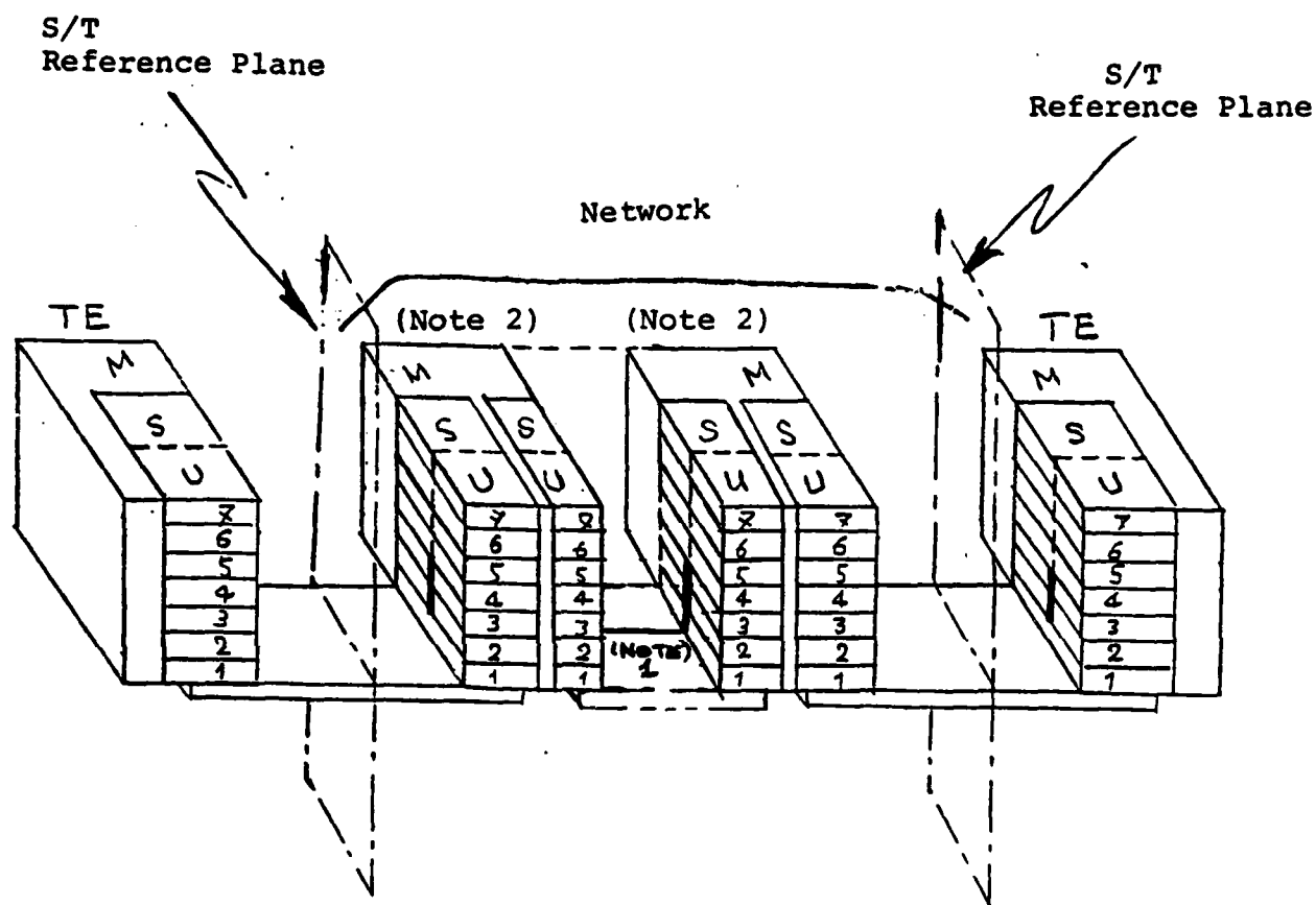
Fig. 4 ISDN PROTOCOL REFERENCE MODEL
