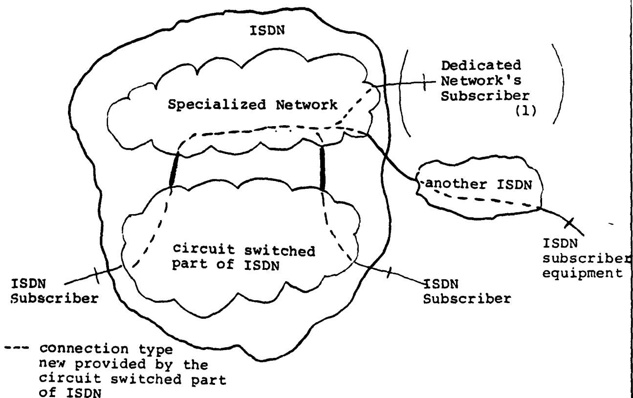
- Fig. 8 / I0210 - Interworking with a specialized network
