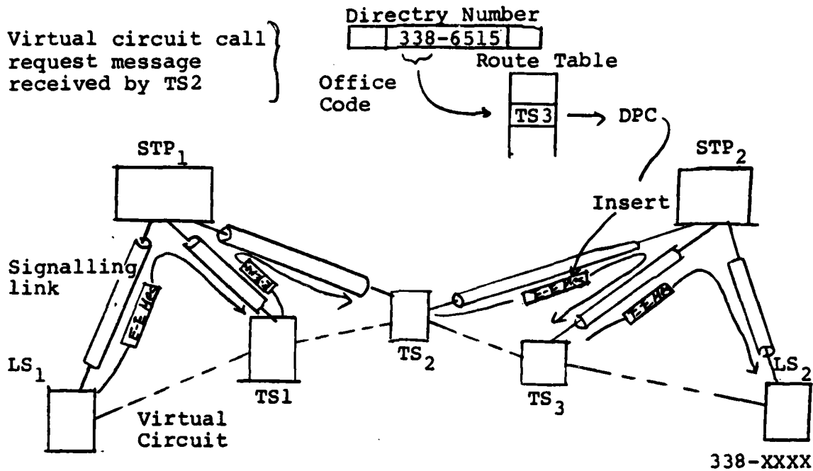
Figure 1. Virtual circuit via transit exchanges
