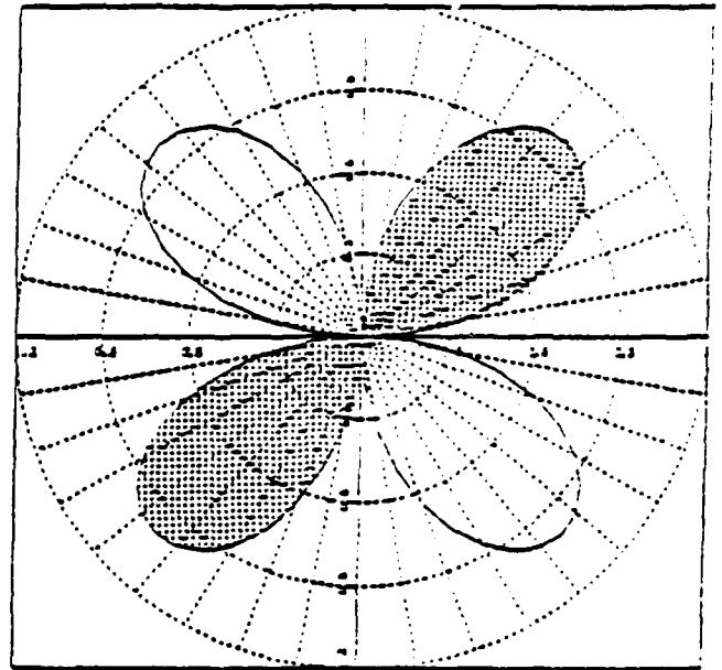
BODY WAVE
