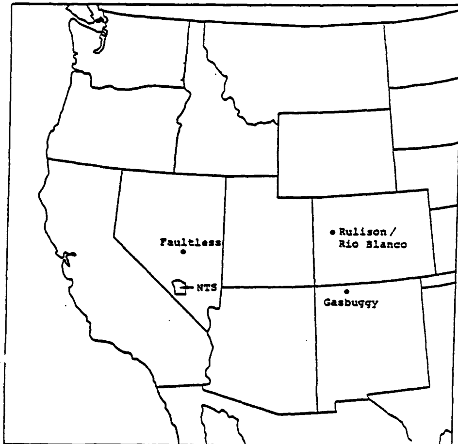
Figure 1. Event location map.
