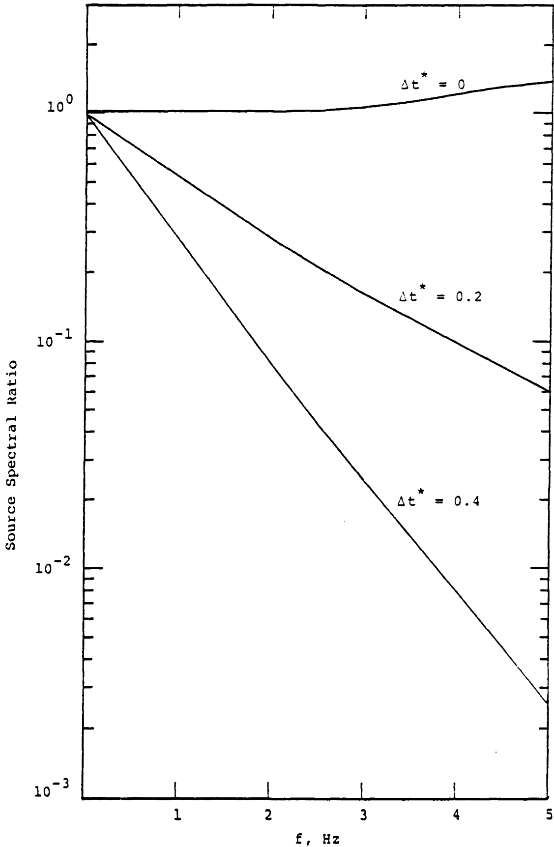
Figure 16. Theoretical Rulison/Gasbuggy P wave spectral ratios computed assuming a range of \Delta t^* values.
