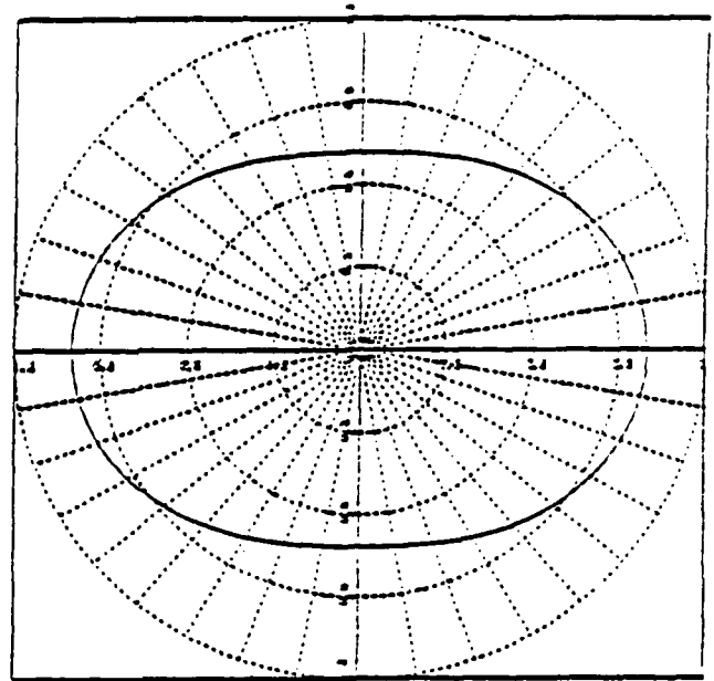
BODY WAVE
