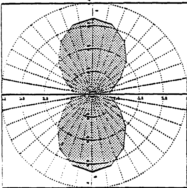
RAYLEIGH WAVE
