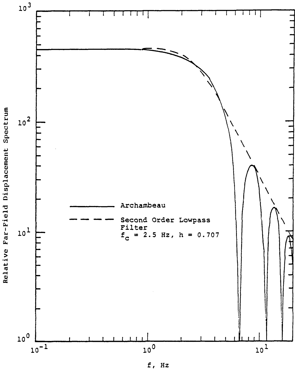
Figure 24. Comparison of Archambeau and lowpass filter approximations to the Rulison tectonic release far-field S wave spectrum.
