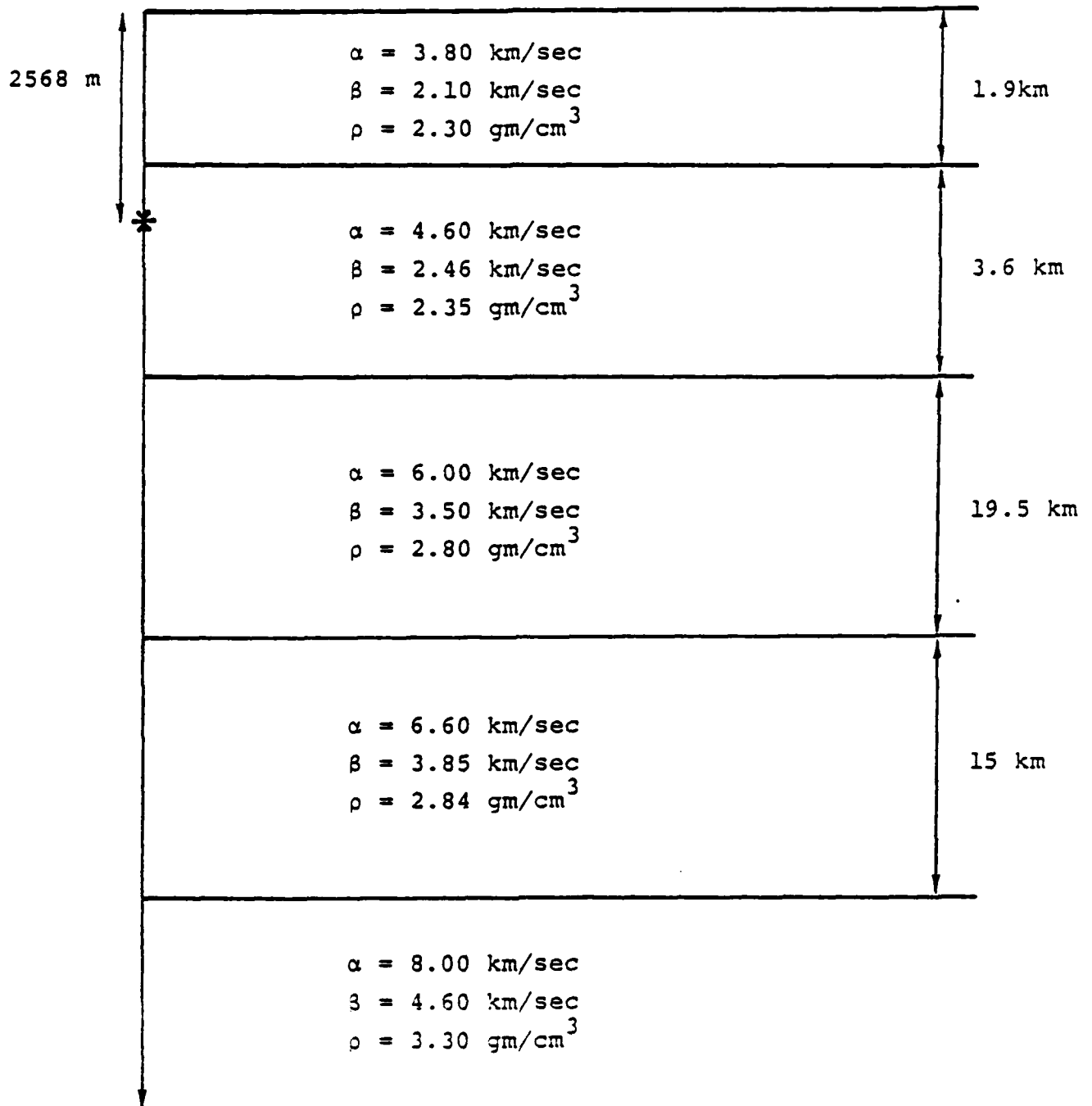
Figure 9. Rulison crustal model.
