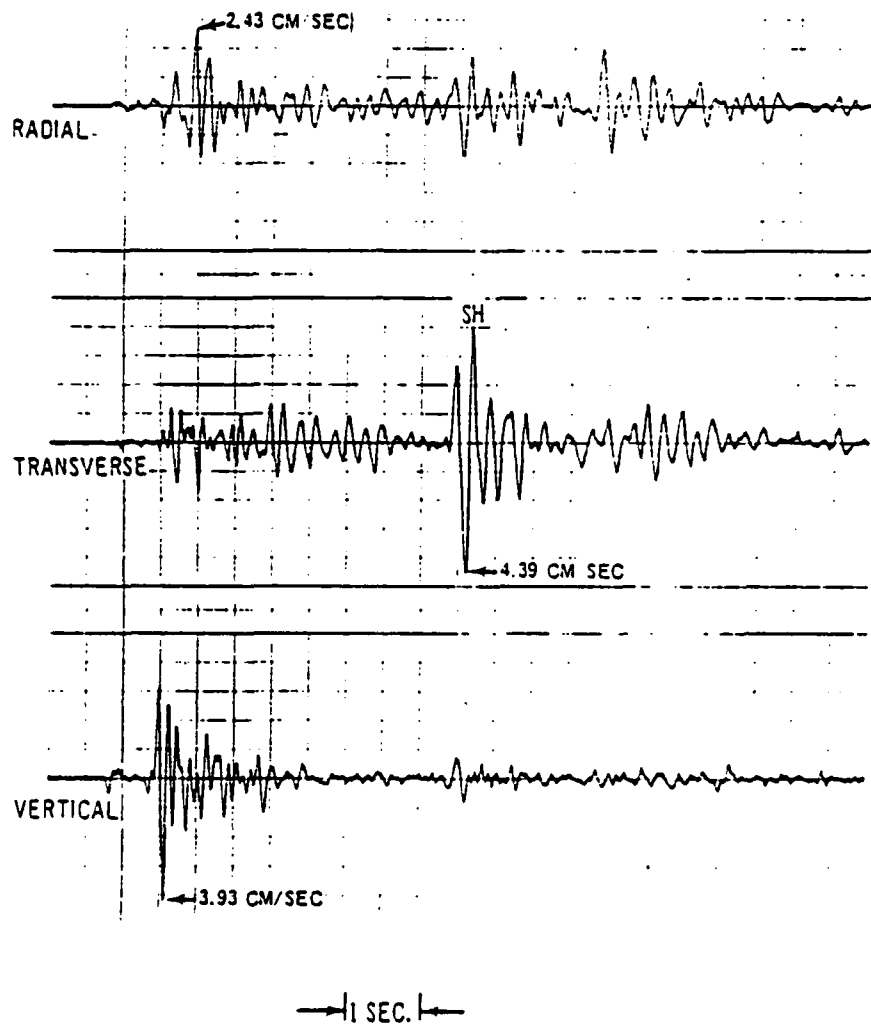
Figure 19. Broadband particle velocity seismograms measured from Rulison at Debeque, Colorado, \Delta = 23 km.
