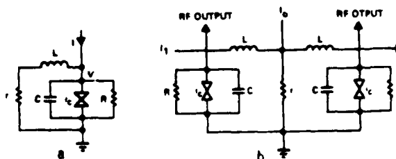
Figure 1. Equivalent circuit of SQUID VCO. (a) Resistive SQUID; (b) Voltage-clamped dc SQUID.
