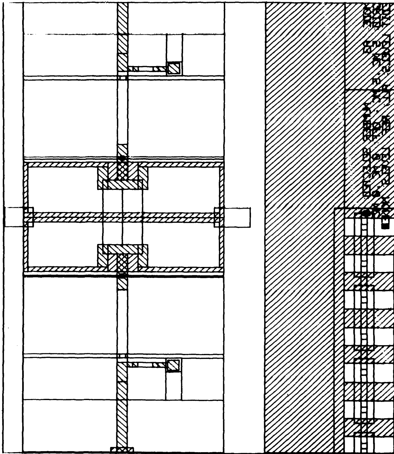
Figure 11c. Composite of mask artwork for the central section of VCO #3.
