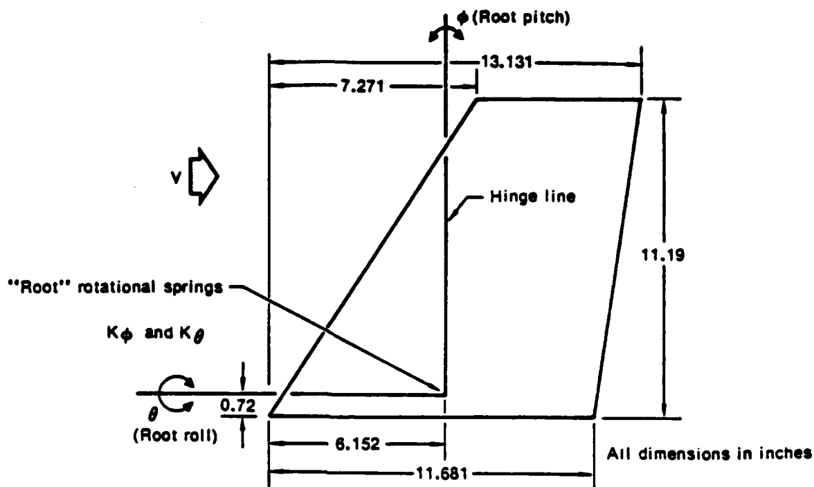
Figure A-1 Control surface geometry
