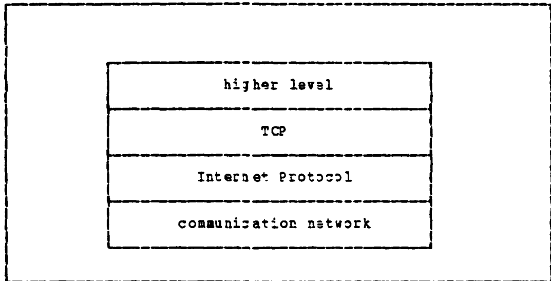
Figure C.1 Protocol Layering.
