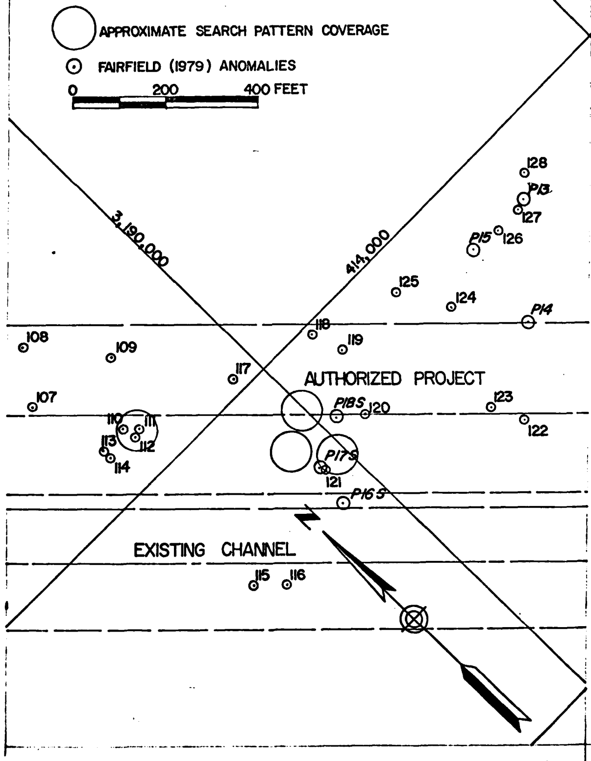
FIGURE 4 POINT 17 (AND 17 S) AREA
