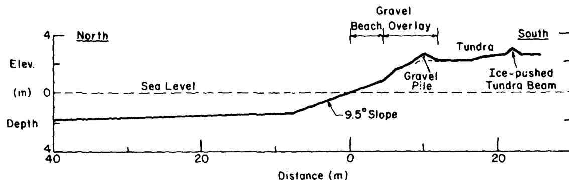
Figure 51. Profile across coast at old ice ride-up tundra scar near left arm of position 17b bracket in Figure B2.
