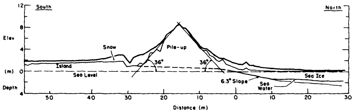
Figure 47. Cross section of 1982 Spy Island sea ice pile-up.
