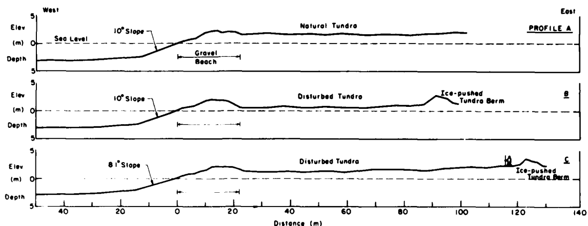
Figure 32. Profiles across coast of undisturbed tundra (A) and ice scars B and C shown in Figure 30.
