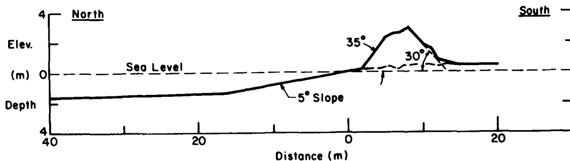
Figure 42. Profile across coast and old pile-up feature (position 6b, Fig. B1).
