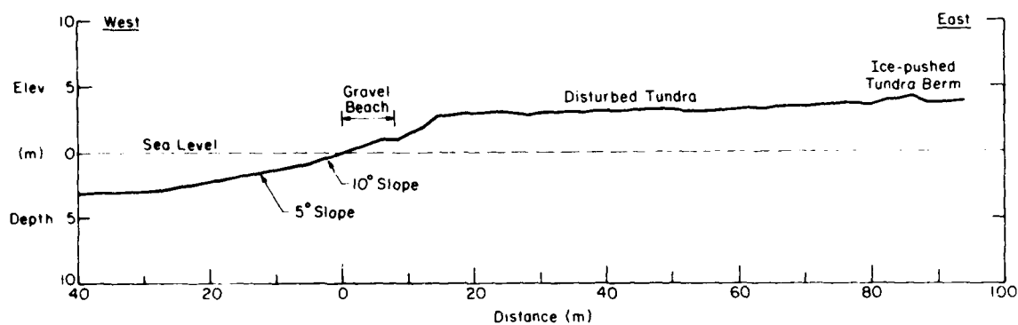
Figure 55. Profile across ice-scarred coast at position C in Figure 33.
