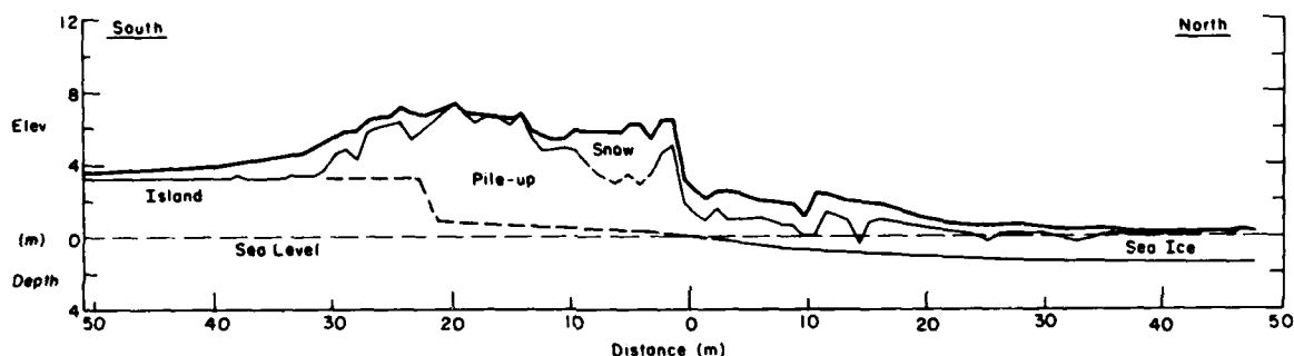
Figure 49. Cross section of Pingok Island sea ice pile-up.
