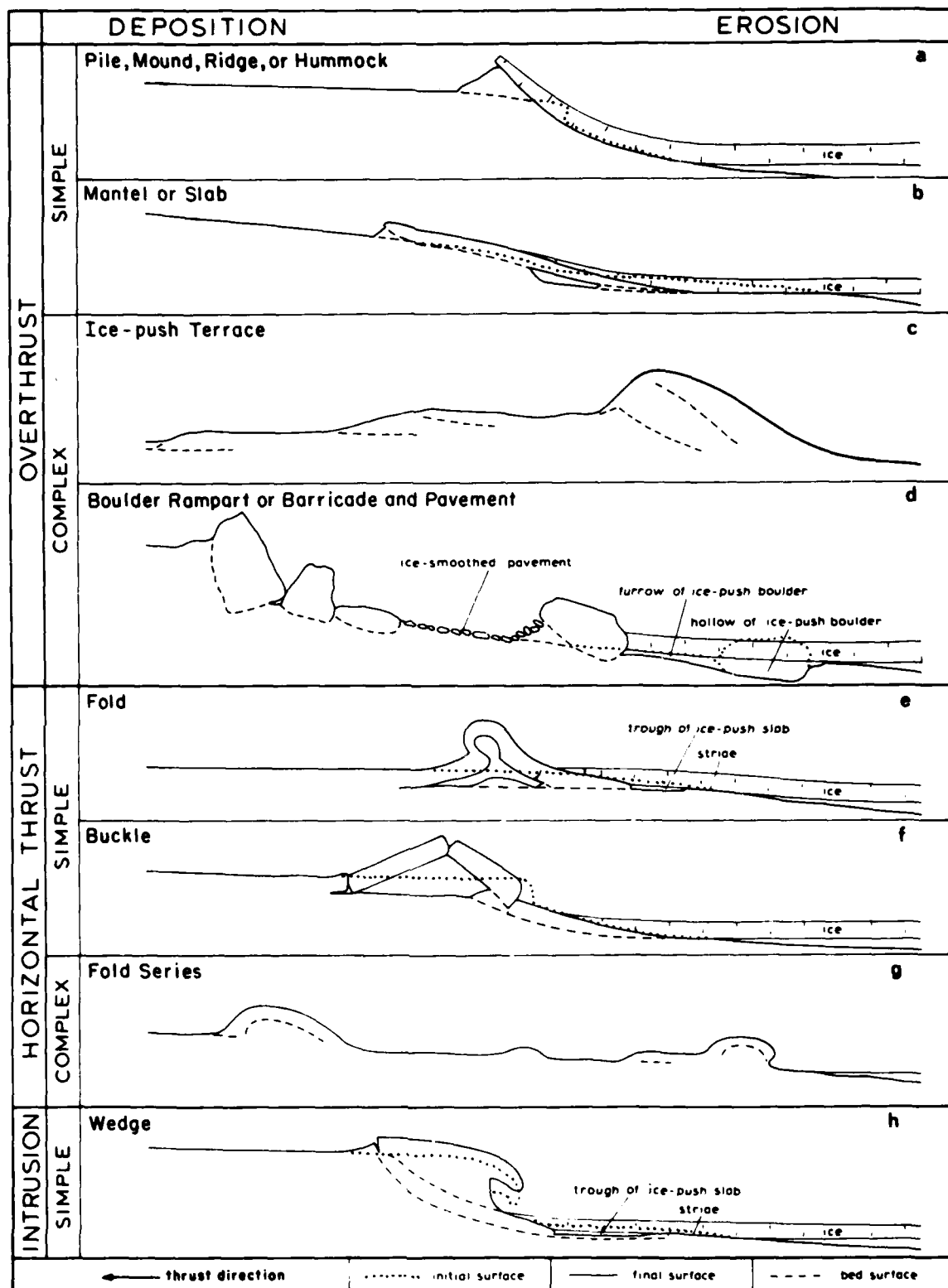
Figure 1. Ice-thrust shore morphology. (After Alestalo and Häikiö 1979.)
