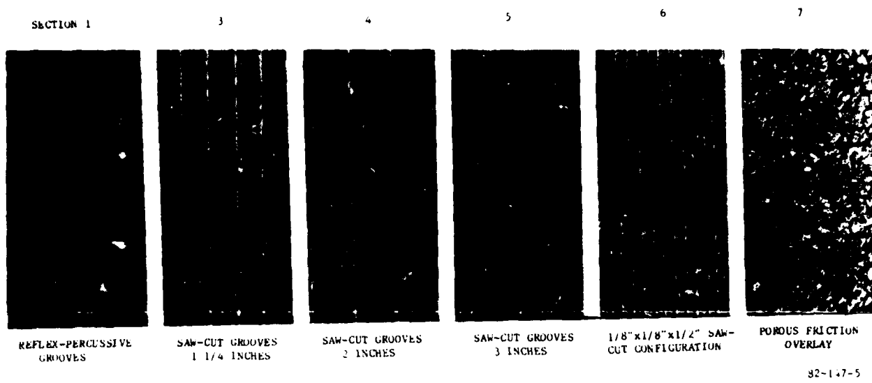
FIGURE 5. VARIOUS TEST SECTIONS OF THE 300-FOOT ASPHALTIC CONCRETE TEST BED (EACH SECTION IS 40 FEET LONG)
