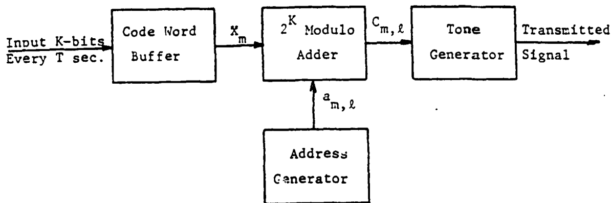
Figure 5-1 Simplified Block diagram of FH-MFSK Transmitter
