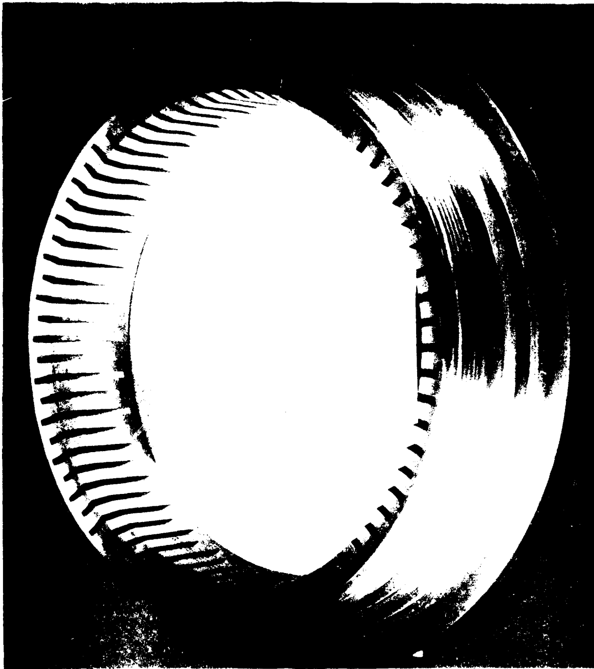
Figure 8. Fuel Injection Ring
