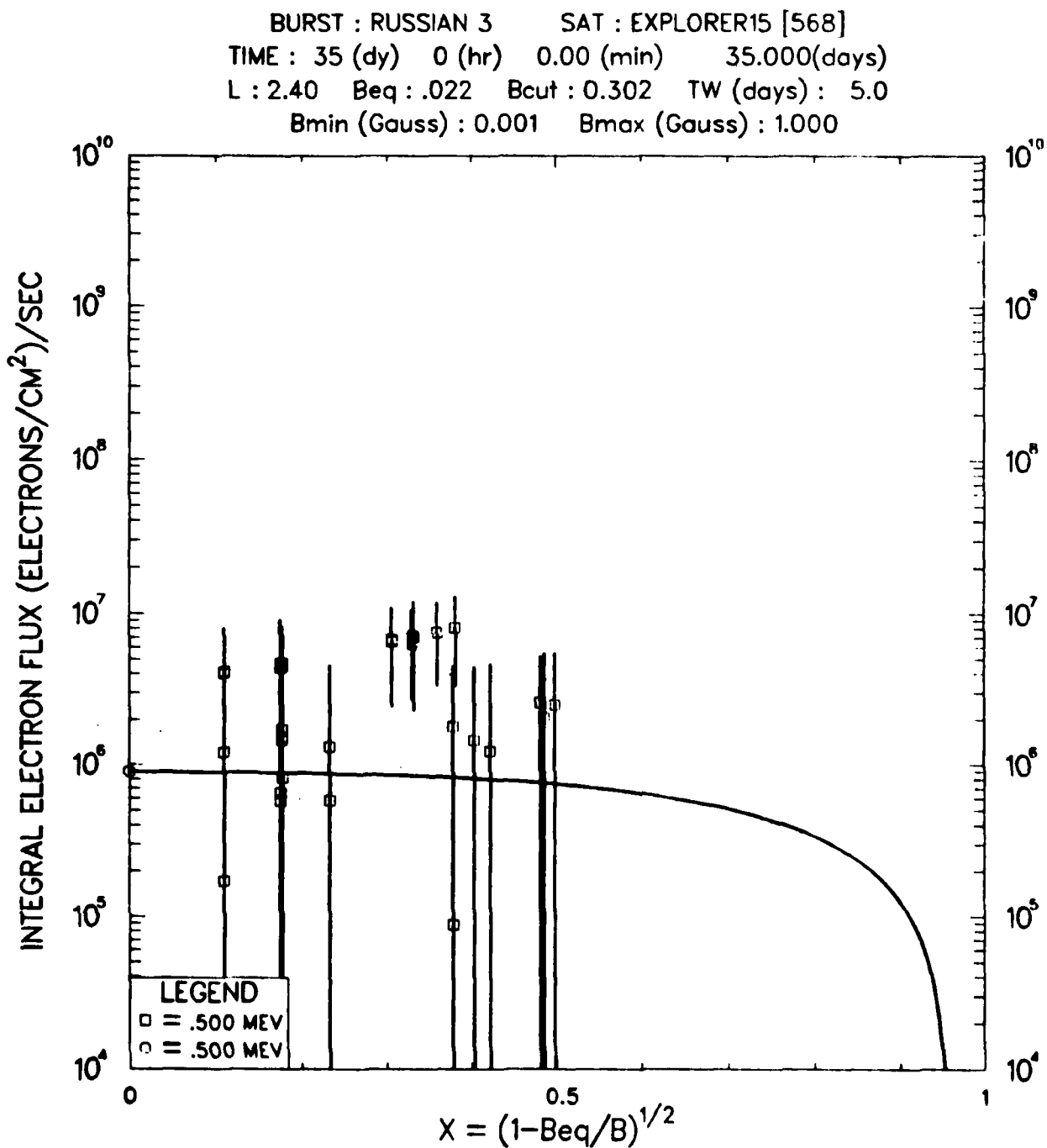
Figure 15(k). Temporal Progression of Raw Data and Fitted Flux Curves at L = 2.4 for Russian 3 Burst ( \tau_n freely varying with physical constraints).
