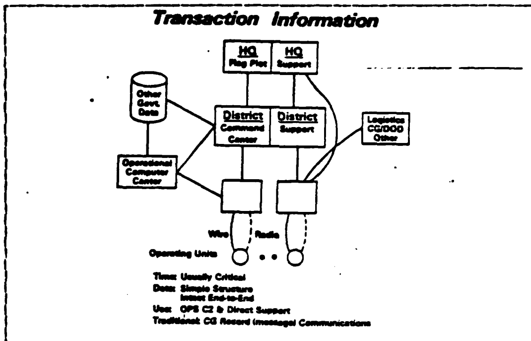
Figure 2.2 Transactional Information.
