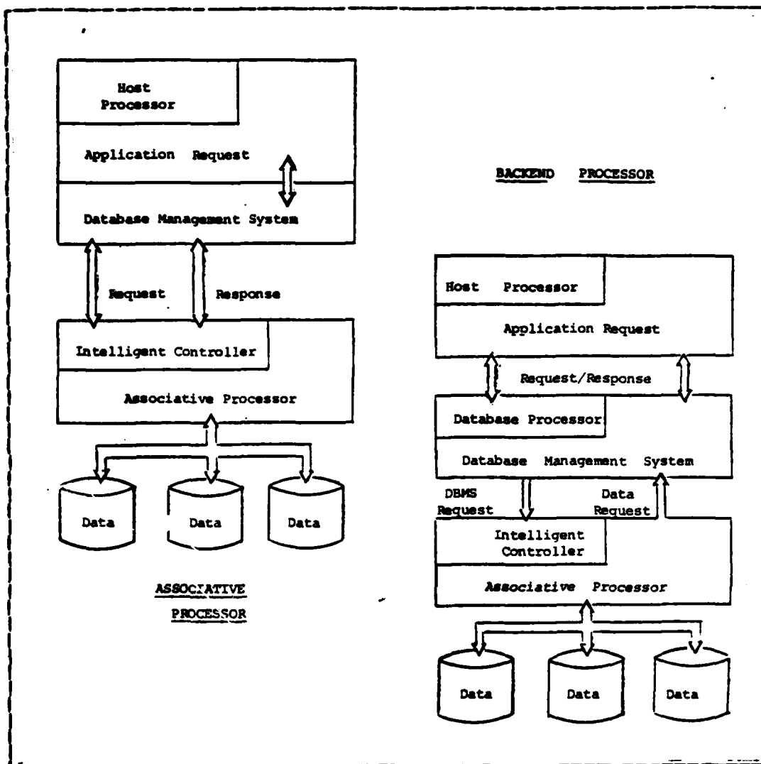
Figure 4.4 Future DBMS Architectures.
