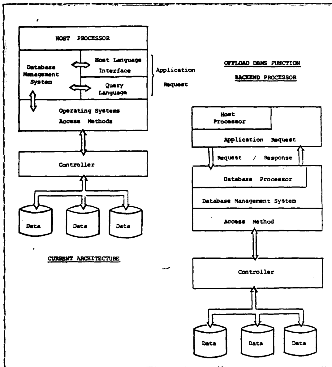
Figure 4.3 Current DBMS Architectures.
