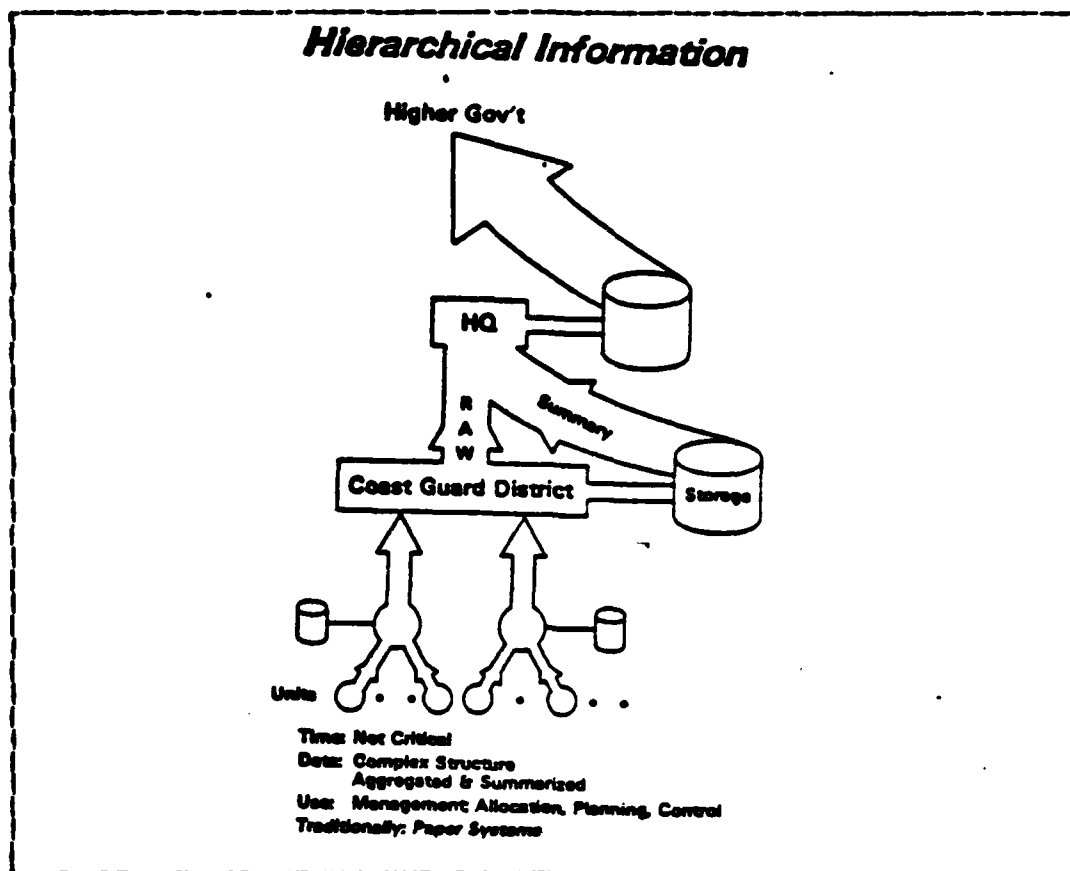
Figure 2.1 Hierarchical Information.
