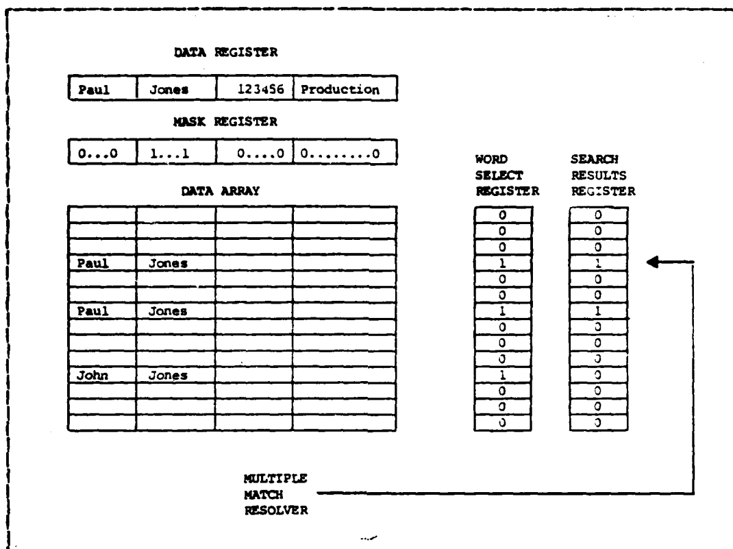
Figure 4.1 Associative System.
