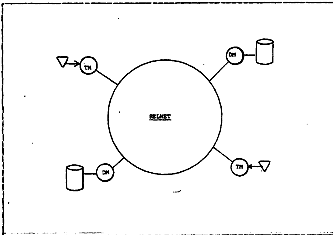
Figure B.1 SDD-1 Architecture.
