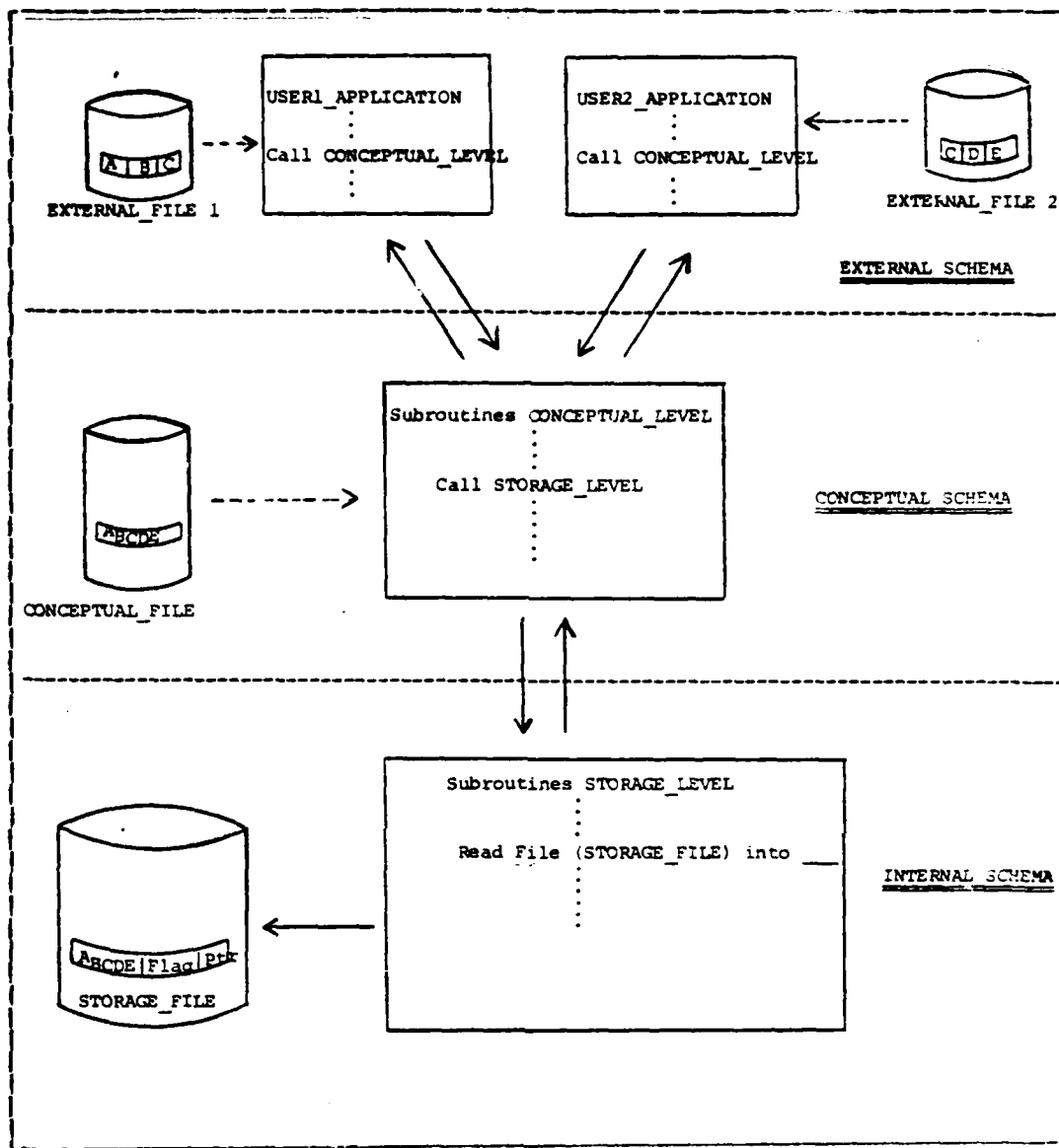
Figure 5.1 Three-Level Hierarchy of a DBMS.
