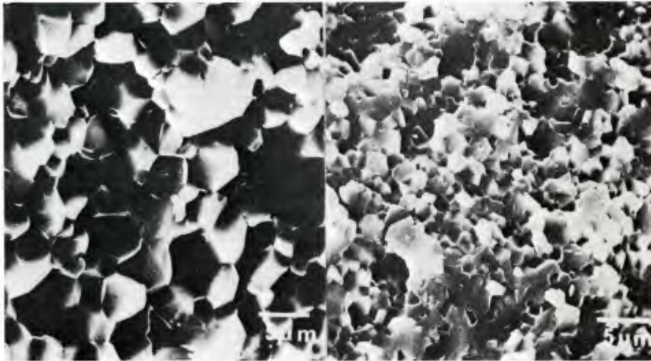
FIGURE 28 Microstructures in sintered alumina as functions of densification path (CTS, RCS), achieving same density ( D = 0.99 ) over same total densification time ( t = 3 \pm 0.1 hr): (a) CTS, 1530^{\circ}\text{C} , 2 hr soak; (b) RCS, peak temperature \sim 1560^{\circ}\text{C} , no soak. Note: typical grain size ranges: CTS 1.8\text{--}5.2\text{ }\mu\text{m} ; RCS 1.2\text{--}2.8\text{ }\mu\text{m} (Palmour, Huckabee, and Hare 1977)
