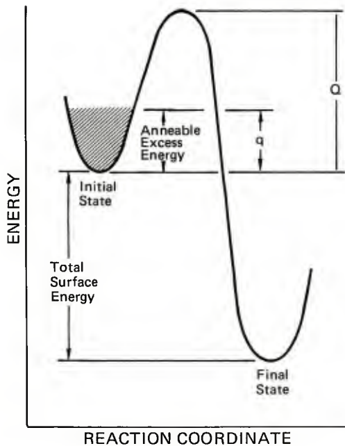
FIGURE 26 Schematic representation of energy relationships influencing densification kinetics at any given porosity and stress (Palmour, Bradley, and Johnson 1969)
