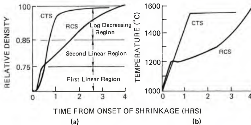
FIGURE 27 Schematic comparisons between conventional temperature sintering (CTS) and three-stage rate controlled sintering (RCS) profiles: (a) Density-time, (b) temperature-time plots (Palmour, Huckabee, and Hare 1977)
