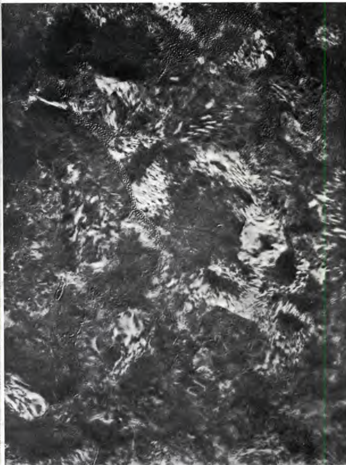
FIGURE 30 TEM mid-radius of explosively compacted AlN (Hoenig and Yust 1981)
