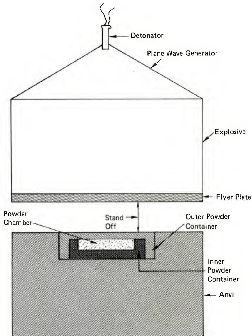
FIGURE 8 Arrangement for powder compaction using an explosively driven flyer plate
