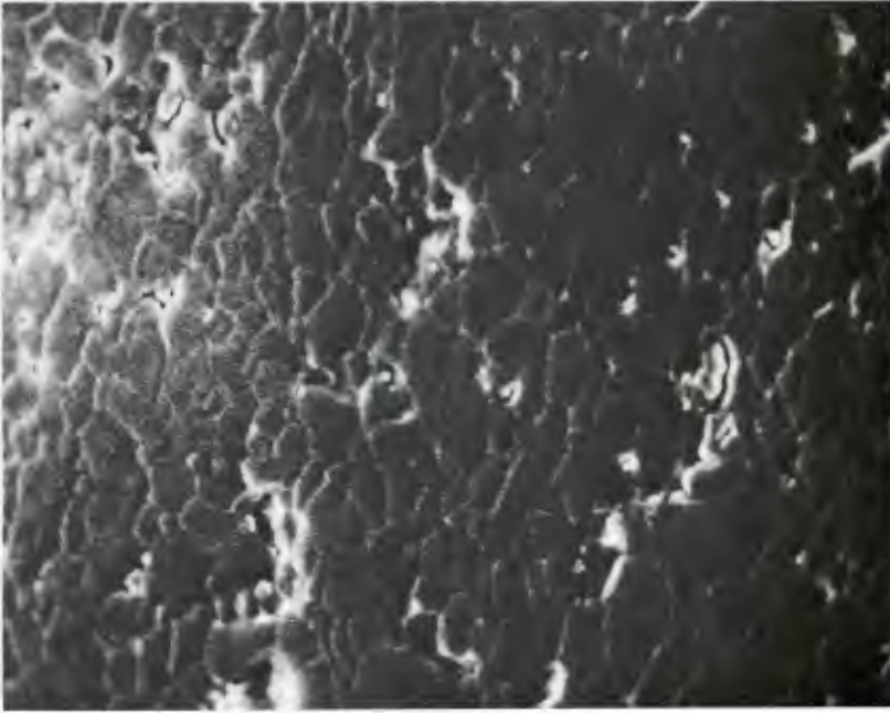
(f) Microstructural details in zone region surface, Zone D, polished and thermally etched surface, SEM, X17,500. Note patches of cluster porosity interspersed in a field of otherwise well compacted fine grains.
