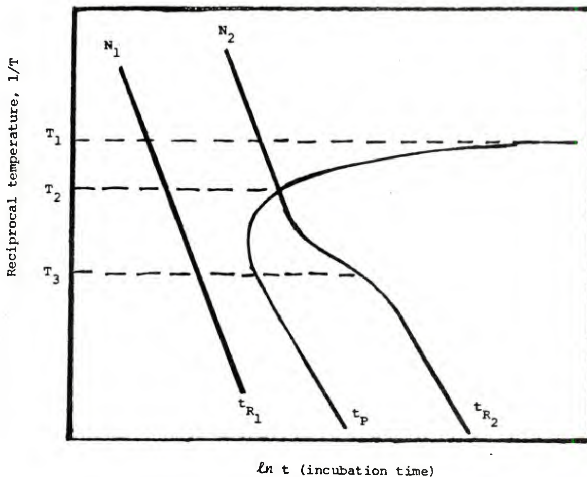
FIGURE 12 Schematic time-temperature-transformation diagram for recrystallization and precipitation processes (Kreye and Hornbogen 1970)
