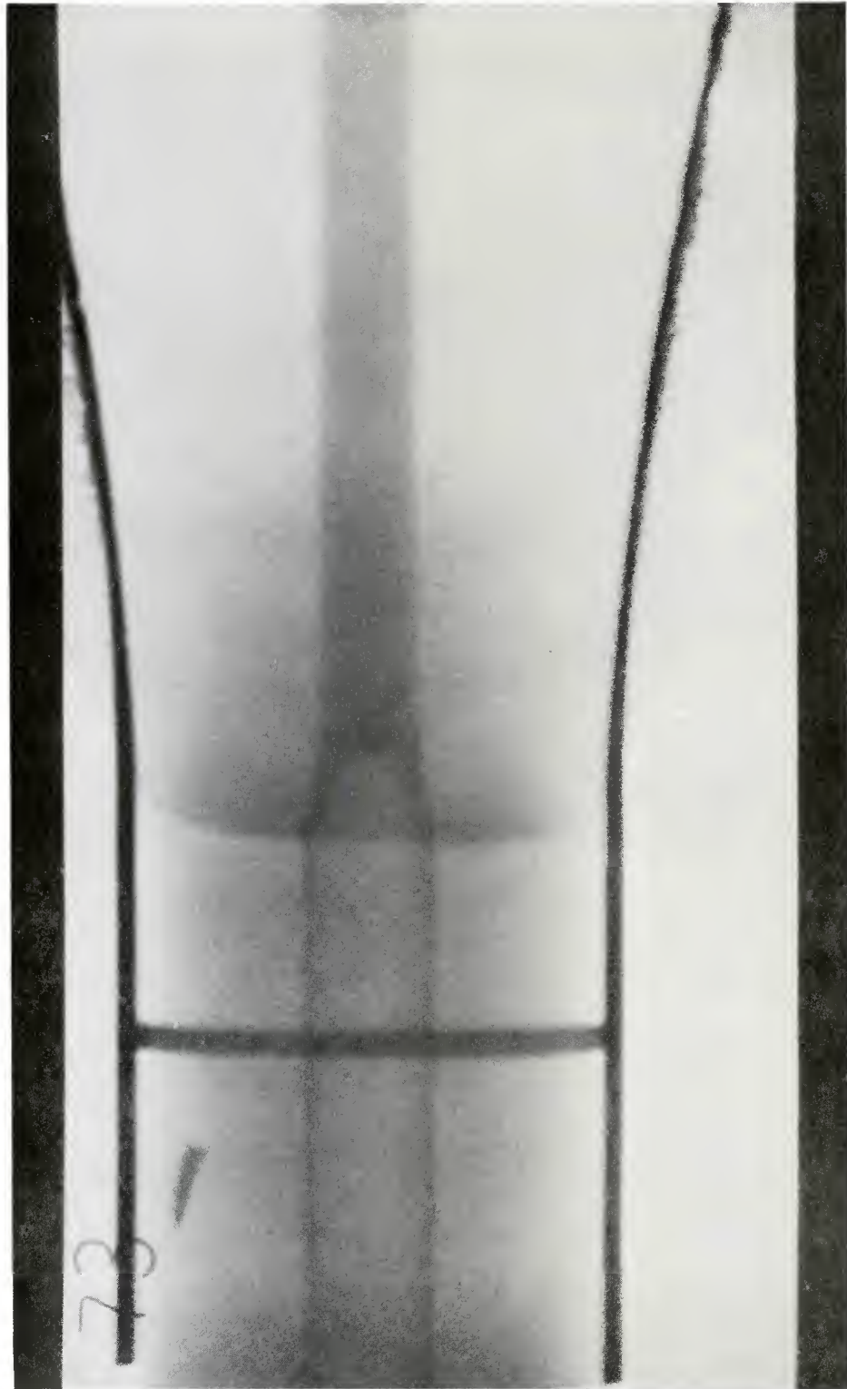
FIGURE 9 Flash X-ray photograph of collapsing cylinder during explosive powder compaction (Linse 1980)
