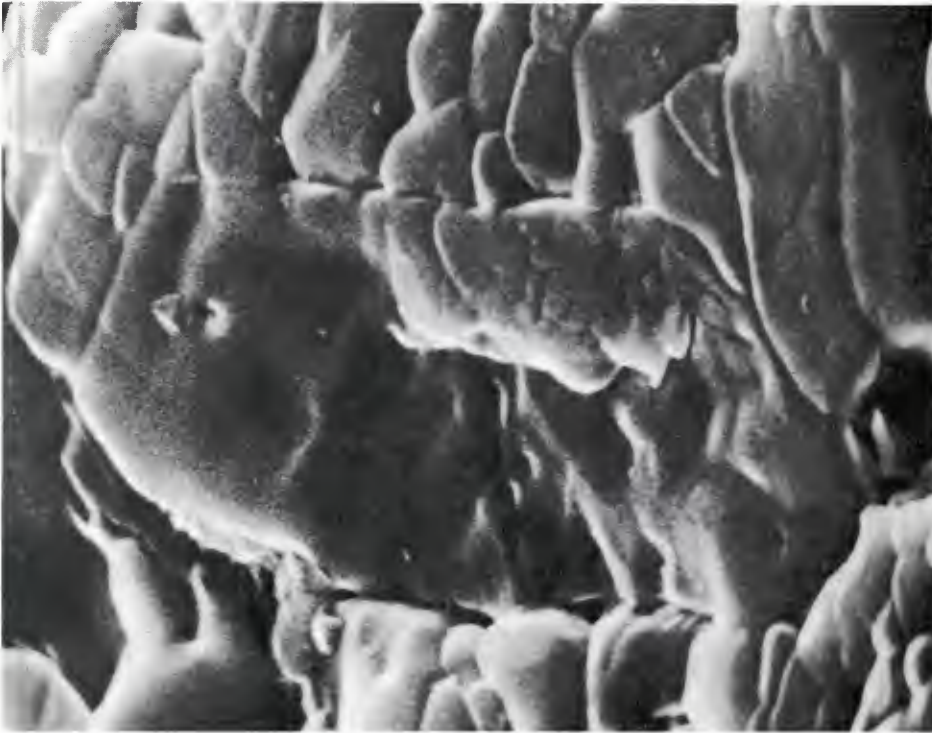
(d) Microstructural details in Zone polished, C on polished, thermally etched surface, SEM, X17,500. Note definite bimodal character of grain sizes, sizes, and local evidences of sub-grain boundaries. This local region seems dense, but the overall zone contains much cluster porosity.
