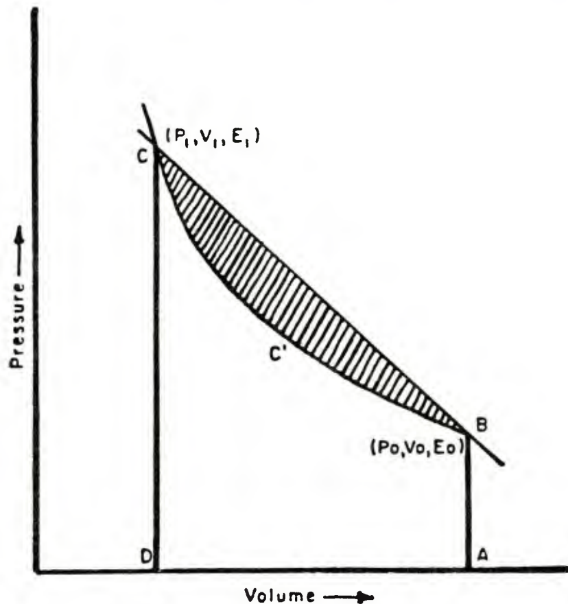
FIGURE 2 Rankine-Hugoniot curve
