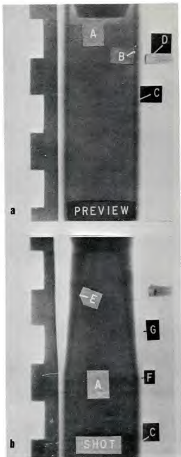
FIGURE 13 Flash X-ray radiographs showing mechanism of explosive shock treatment of powders. Assembly before detonation of explosive (a) and assembly immediately after initiation of explosion (b). A. ceramic powder; B. tube wall; C. explosive; D. target trigger to actuate X-ray tubes; E. shock front advancing into powder; F. detonation front; G. detonation products. (Bergmann and Barrington 1966)
