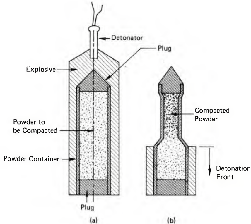
FIGURE 7 Assembly for explosive compaction of powders: (a) prior to compaction and (b) during compaction (Prümmer 1973)
