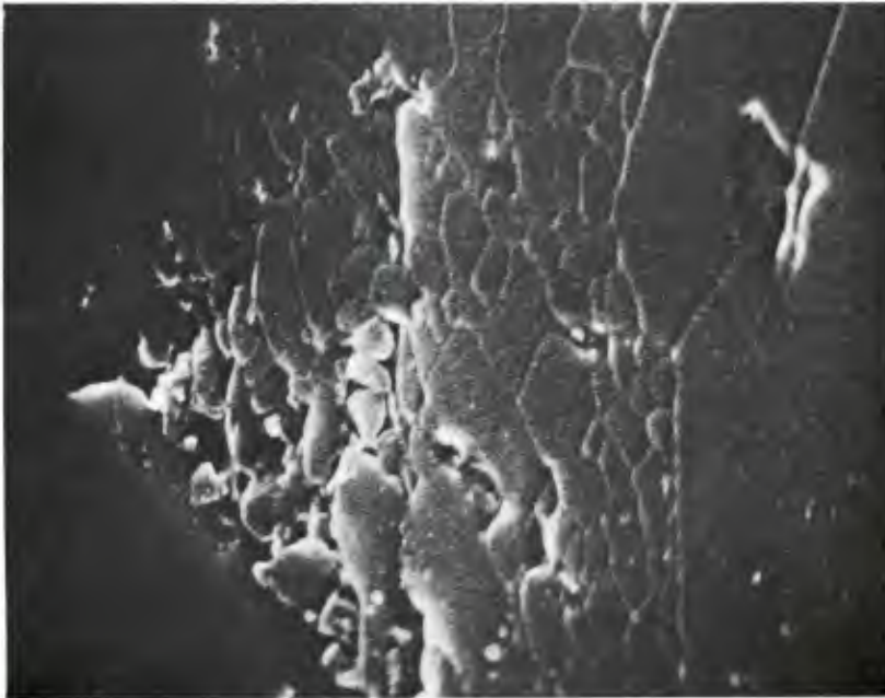
(e) Microstructural details in transition between Zones C and D, polished and thermally etched surface, SEM, X17,500. Note substantial region of cluster porosity at upper left, and sharp interface between the fine midfield grains and the large recrystallized foreground grain.
