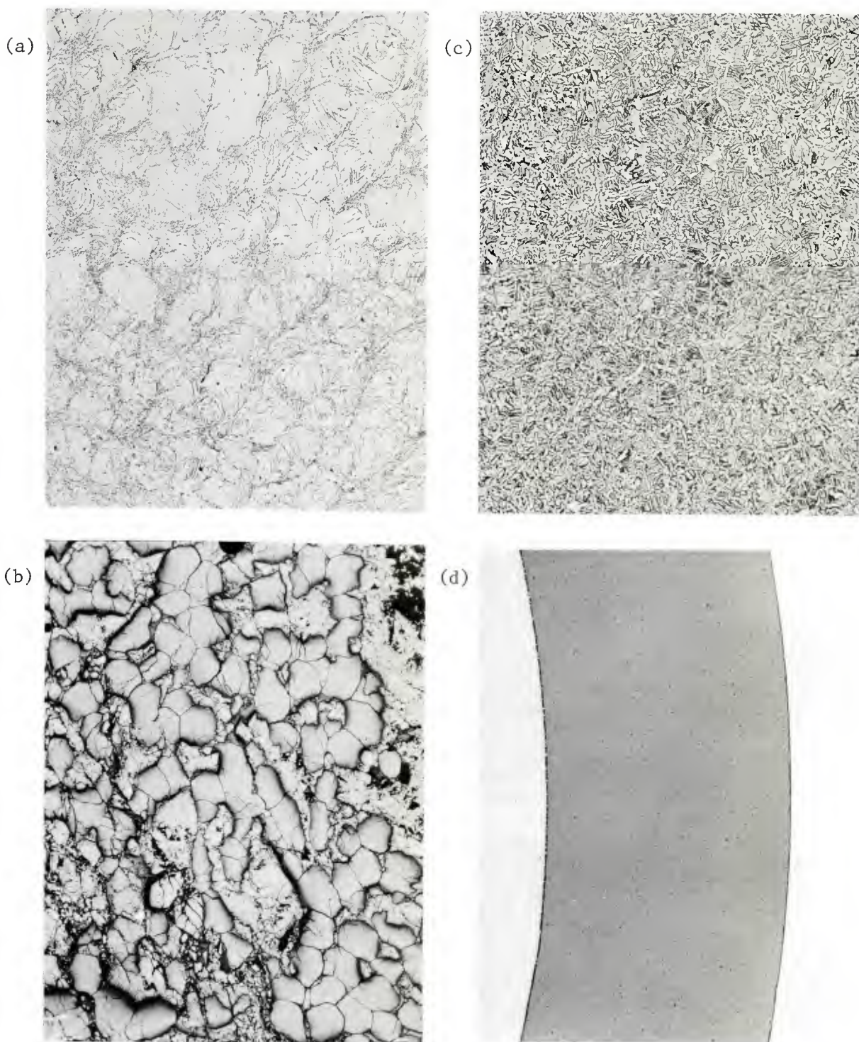
FIGURE 23 Examples of successful applications of direct dynamic compaction hot compacted technology to a variety of metal and ceramic powders: (a) tungsten, (b) B_4C-UO_2 , (c) Ti-6Al-4V alloy, hot compacted; and (d) SiAlON (Linse 1981)
