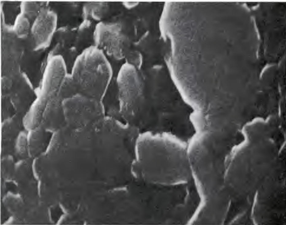
(c) Microstructural details in Zone B on thermally etched surface, SEM, X10,500. Note pores and evidences of sub-grain boundaries.
