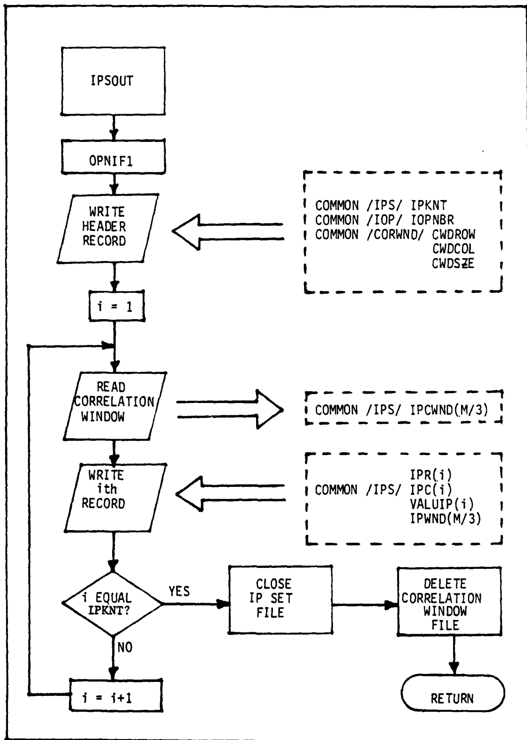
Figure 14. Interesting Point Set Storage Flow Diagram
