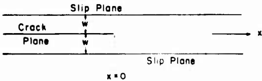
Fig. 1. Double slip plane model. The crack is assumed to be an atomically sharp slip crack on the negative x -axis with the tip at the origin. Two planes parallel to the crack plane are permitted for dislocation generation and slip. The planes are assumed to be a distance w from the crack plane. Mode III or II will be assumed throughout for purposes of analysis.
