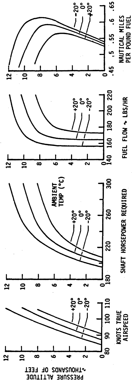
FIGURE B. SAMPLE LEVEL FLIGHT CRUISE PERFORMANCE
