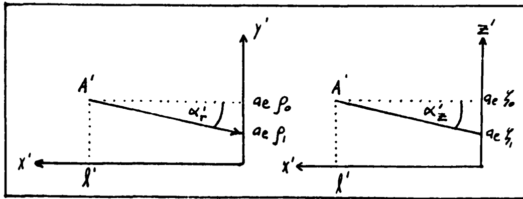
Figure 5 - Entrance Angles
