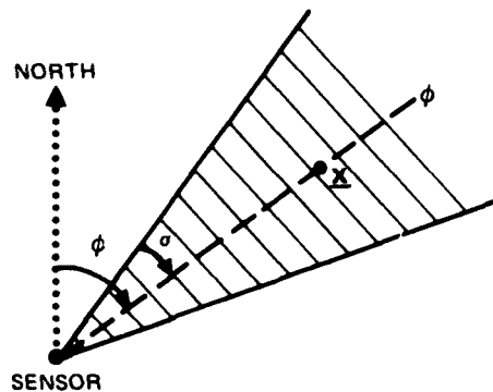
Figure 16. Example of support for bearing measurement probability density described by equation (33).
