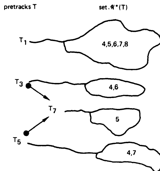
Figure 7. Illustration of sets of hypotheses \mathcal{H}^*(T) attached to pretracks T corresponding to Table 1. Thus, the integers 4 through 8 label hypotheses h_4 to h_8 , and we can deduce from the above set structure that, for example, h_6 = [T_1, T_3] or that T_3 appears in hypotheses h_4 and h_6 .
