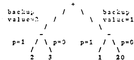
Figure 3: Pure Max chooses the left branch.
