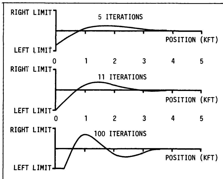
FIGURE 4-12. CONTROL HISTORIES
