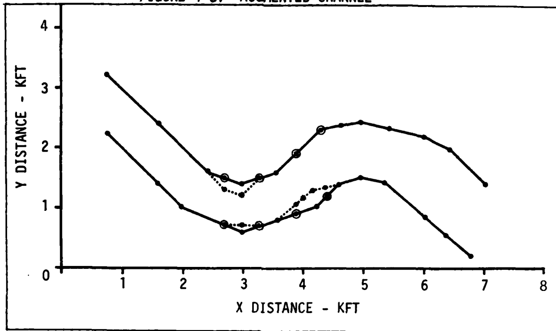
FIGURE 4-3. AUGMENTED CHANNEL
