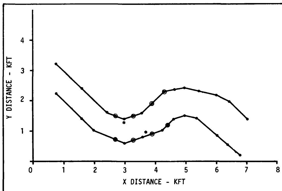
FIGURE 4-2. ORIGINAL CHANNEL
