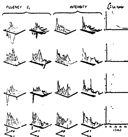
FIG. 4. Transverse energy current J_T and intensity are plotted isometrically for four shots in a statistical ensemble. In some of the shots the phase curvature is such that the associated energy flux flows inwardly; i.e., the transverse energy current is negative, which could lead to self-focusing. Inward energy flow never occurred for simulations using a homogeneous initial tipping angle (without quantum initiation) for any value of the Fresnel number. Here, n_0^0 = 9.5 \times 10^{10} \text{ cm}^{-3} , F = 1.49 , and 10^4 \langle \theta_0^2 \rangle^{1/2} = 2.15, 1.63, 1.79 , and 1.16 rad, respectively, from top to bottom. Note the fluctuations in peak maximum and its associated delay in the output integrated over \rho (last column).
