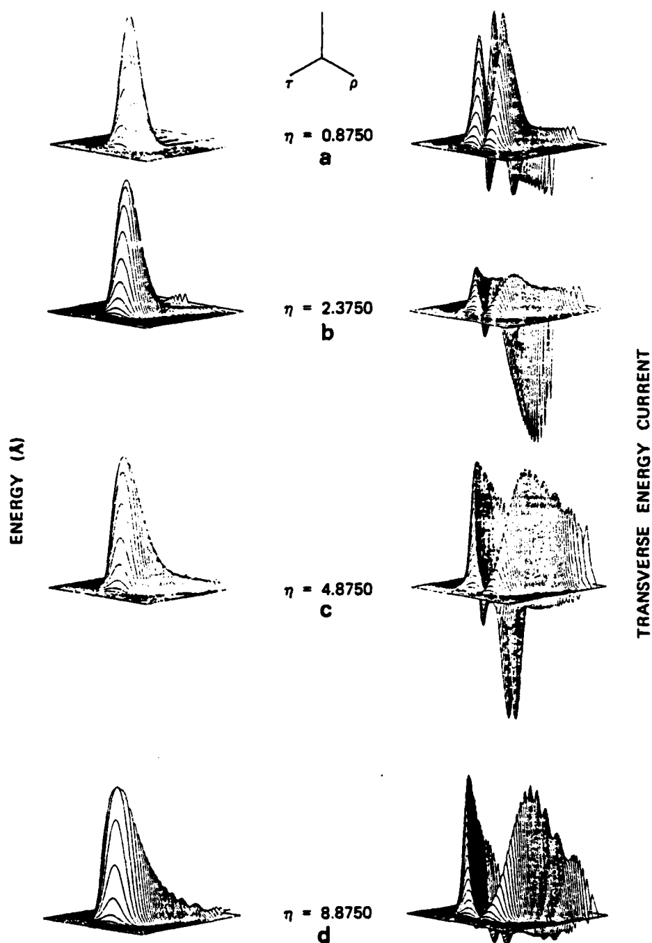
Fig. 19. Isometric plots of the amplifier field energy and transverse energy flow profile for various time slices at the four regions of interest, with stretched radial coordinate for proper accounting of the transverse boundary condition. No severe reflection or abrupt variation in the field energy, at the wall boundary, is observed.
