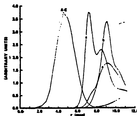
FIG. 12. Radially integrated normalized intensity profiles for the SF and injected pulses at z=5.3 -cm penetration depth for three different values for the SF transition effective gain g_s . The on-axis initial area \theta_i for the injected pulse is \theta_i=3\pi . All other parameters are the same as for Fig. 10.
