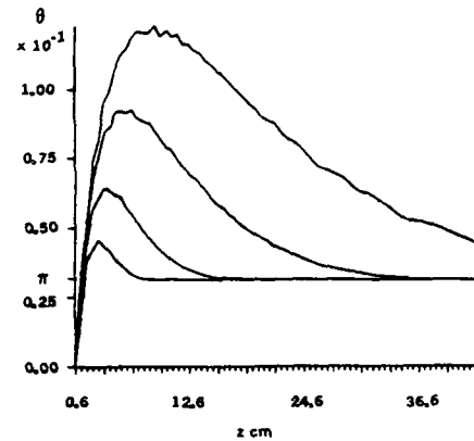
Figure 2. Pulse area \theta = \int_0^\infty |\epsilon| d\tau vs. propagation distance z for numerical integration of Eqs. (2-1) - (2-3). Values of the parameters used are those of Figure 1 except for \kappa : 1) \kappa = 5.2 \text{ cm}^{-1} , g/\kappa = 56.08 ; 2) \kappa = 10.4 \text{ cm}^{-1} , g/\kappa = 28.04 ; 3) \kappa = 20.8 , g/\kappa = 14.02 ; 4) \kappa = 41.6 \text{ cm}^{-1} , g/\kappa = 7.01 .
