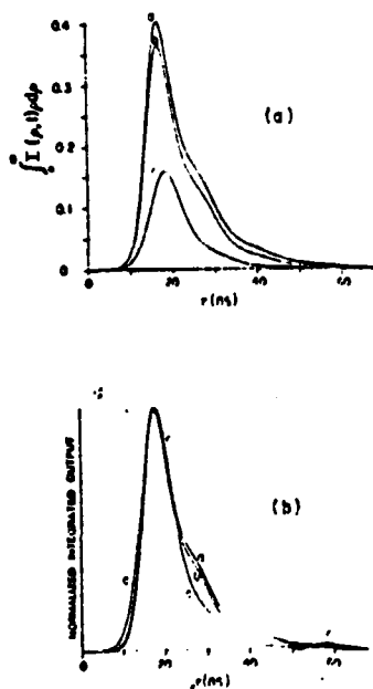
FIG. 12. Transverse effects and inhomogeneous broadening. Parameters: Same as Fig. 10 except that transverse effects ( F=0.27 ) are now considered. Including T_2^* in the Cs simulation is seen to be a small refinement which does suppress the tail slightly. (a) Relative integrated outputs. (b) Normalized integrated outputs with peaks shifted to coincide with each other to simplify pulse-shape comparisons.
