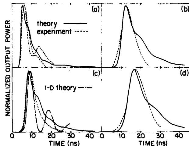
FIG. 3. Theoretical fits to Cs data of Ref. 3. The two dashed-line curves in (a) indicate typical experimental shot-to-shot variations. F = 1 , L = 2 cm, T_1 = 70 ns, T_2 = 80 ns, \lambda = 2.931 \mu m, \tau_0 = 551 ns, \theta_0 is uniform or Gaussian, and n_0(r) is Gaussian. The following give \theta_0^0(\text{fit}) , n_0^0(\text{fit}) , n_0^0(\text{exp}) , with \theta_0^0 in units of 10^{-1}/\text{cm}^2 and n_0^0 in units of 10^{10}/\text{cm}^3 : (a) 1.07, 31, 19; (b) 1.37, 18, 7.6; (c) 1.69, 11.9, 3.8; (d) 1.96, 8.85, 3.1. The broken-line curve in (b) is the one-dimensional fit of Ref. 3b, with \theta_0^0 = 1.69 and n_0^0 = 12 .
