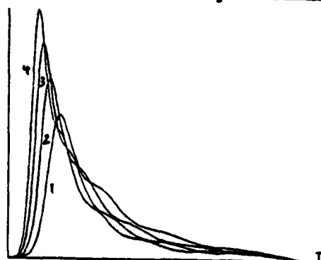
Fig. 30. Contrast of the total energy per unit atom (versus time) for different radiation damping time \tau_R for a chosen \mathcal{F} = 0.7 , and a fixed tipping angle \theta_R = 3 \times 10^{-3} . g_R = 100 , 125, 150, 175.
