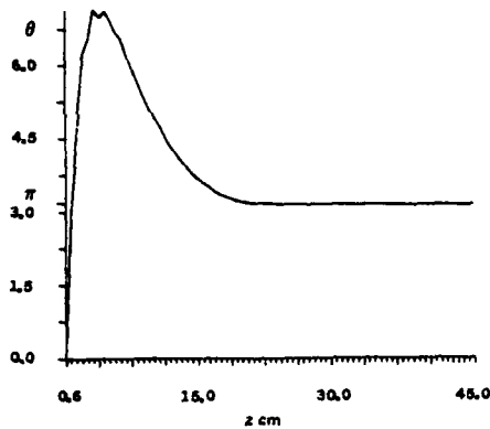
Figure 1. Pulse area \theta = \int_0^\infty |\epsilon| d\tau vs. propagation distance z for numerical integration of Eqs. (2-1) - (2-3). Values for the parameters used in the calculation are: g = 291.6 \text{ cm}^{-1} , \kappa = 2.60 \text{ cm}^{-1} , g/\kappa = 112.15 , T_1 = T_2 = 70 \text{ nsec} , \phi_0 = 9.42 \times 10^{-4} , \tau_c = 89.4 \text{ psec} .
