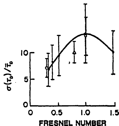
FIG. 6. Fresnel-number dependence of the uncertainty in delay time normalized to the average delay. Points are as follows: \bullet , seven trajectories with n_0^0 = 9.5 \times 10^{10} \text{ cm}^{-3} and \langle \theta_0^2 \rangle^{1/2} = 1.89 \times 10^{-4} rad; \square , n_0^0 = 18 \times 10^{10} \text{ cm}^{-3} and \langle \theta_0^2 \rangle^{1/2} = 1.37 \times 10^{-4} rad, for 13 trajectories for F=1 , and for 16 trajectories for F=\pi^{-1} ; \Delta , experimental value for 468 trajectories. A peak close to F=1 can be argued as follows: For small F , strong diffractive coupling reduces fluctuations in the overall output. For large F , so many transverse modes compete that a good average is obtained on every shot. For F=1 , competition of a few modes is maximal, resulting in large fluctuations. Meaningful calculations for large F require an increasing number of transverse steps, and so we avoid the large- F region.
