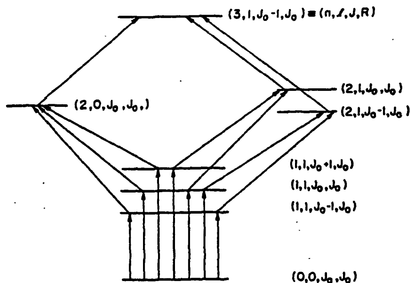
Figure 1: Schematic diagram of dipole-allowed transitions (indicated by arrows) that begin on a given effective state [4(c)] (n, l, J, R) = (0, 0, J_0, J_0) and end on (3, 1, J_0 - 1, J_0) .
