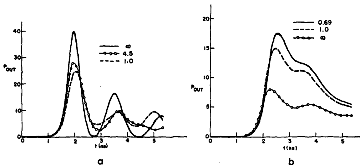
Figure 2. Total energy coherently emitted per unit atom in arbitrary units, as a function of time with Fresnel number as the labelling parameter. \theta_0 = 10^{-4} for all radii, \tau_R = 8\pi\tau_0/3n_0^0 \lambda^2 L = 0.046 ns, and L = 5.23 cm. (a) Uniformly inverted cylinder: inversion constant out to \rho_0 and zero beyond with F = \pi\rho_0^2/\lambda L . The output is accepted only out to \rho_0 . (b) Gaussian inversion cylinder with F and n_0(r) defined as in Fig. 1.
