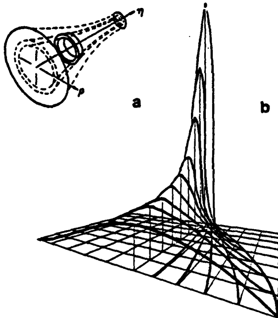
Fig. 2. (a) Isometric representation of the beam cross-section as it experiences self-focusing: The cross-section decreases as a function of the propagation distance; (b) An isometric display of the time integrated field energy as a function of \rho and \eta to illustrate the resolution limitation associated with uniform mesh.
