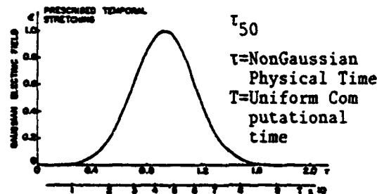
Fig. 3. Non-uniform prescribed temporal stretching.
