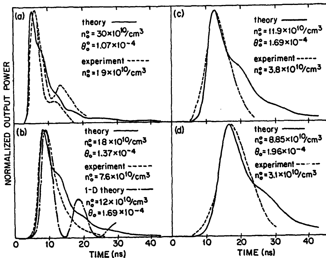
Figure 1. Theoretical fits to Cs data of Ref. 8a. The two experimental curves in (a) indicate typical shot-to-shot variations. The 1-D curve in (b) is the fit of Ref. 8b to the one-dimensional theory. F = \pi r^2 / \lambda L = 1 , L = 2 cm, T_1 = 70 ns, T_2' = 80 nsec, \lambda = 2.931\mu , \tau_0 = 551 ns, \theta_0 uniform Gaussian, inversion n_0(r) = n_0^0 \exp[-\ln 2 (r/r_p)^2] .
