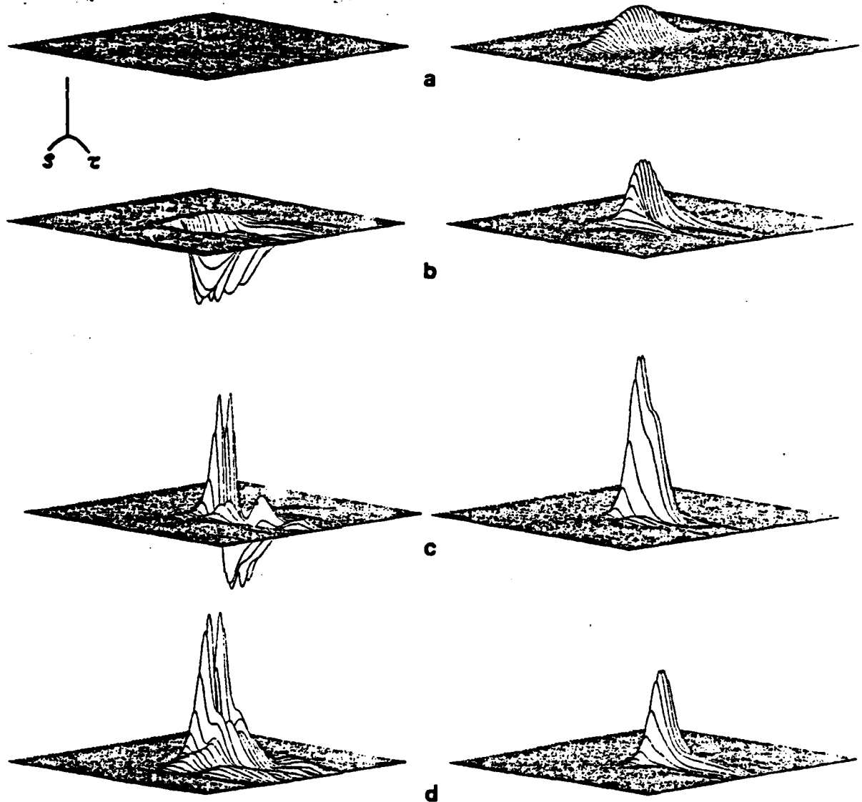
Fig. 13. Isometric plots of the absorber field energy and transverse energy flow, against the retarded time for various transverse coordinates at four regions: (a) reshaping, (b) build-up region, (c) focal region, (d) post-focal region.
