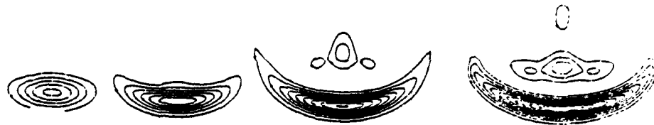
Fig. 19. Amplifier field energy contour plots for the four propagation regions of interest. Note the temporal advance associated with coherent exchange of energy between light and matter (the smaller area propagates more slowly than the larger one), as well as beam cross-section expansion.
