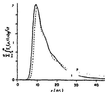
FIG. 3. Effect of fluctuations on the average pulse shape. Average over 17 trajectories with fluctuations (solid curve) has a slightly shorter delay and a smaller tail than the dashed curve with no fluctuations and a uniform \theta_0 . Here, n_0^0 = 18.2 \times 10^{10} \text{ cm}^{-3} , (\theta_0^2)^{1/2} = 1.37 \times 10^{-4} rad, and F = 0.32 .
