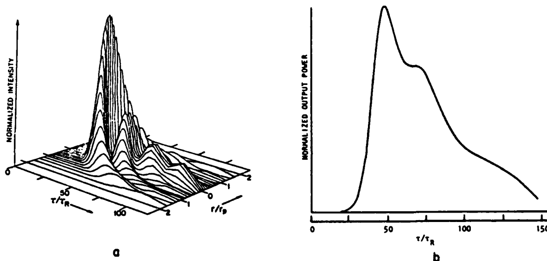
Figure 3. Energy as a function of (a) transverse coordinate \rho = r/r_0 and time and (b) only time after integration over \rho . Notice that strong ringing is predicted for a small-aperture detector in the center of the beam although very little ringing is in evidence after radial averaging. \theta_0 = 2.38 \times 10^{-4} \exp(-\rho^2/2) , \tau_R = 4.9 \text{ ns} , F = 1 , L = 22.4 \text{ cm} , and transverse Gaussian inversion profile. As F is decreased, ringing is washed out into smaller and smaller \rho .
