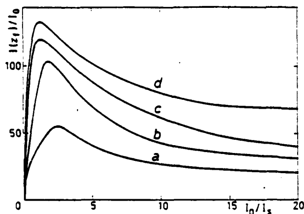
Figure 7. On-axis intensity at the focus as a function of I_0/I_s for same parameters as in Fig. 6.
