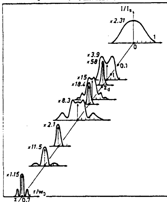
Figure 5. Intensity profile. I_0/I_s = 2.31 \alpha_1 = 2 , \delta T_2 = -60 , z_d = 0.22 cm, F = 2.9 , l^2 = 0.15 cm.
