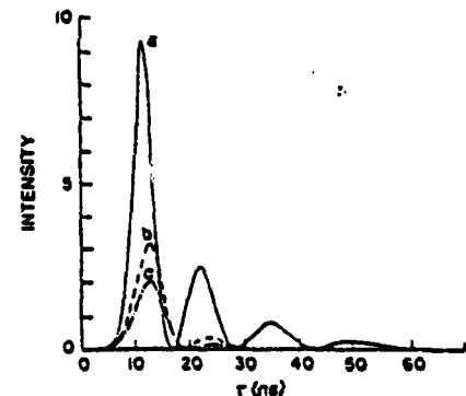
FIG. 11. Removal of ringing by inhomogeneous broadening. Parameters: Same as Fig. 10 with T_2^* = 0.67 \text{ ns} .
