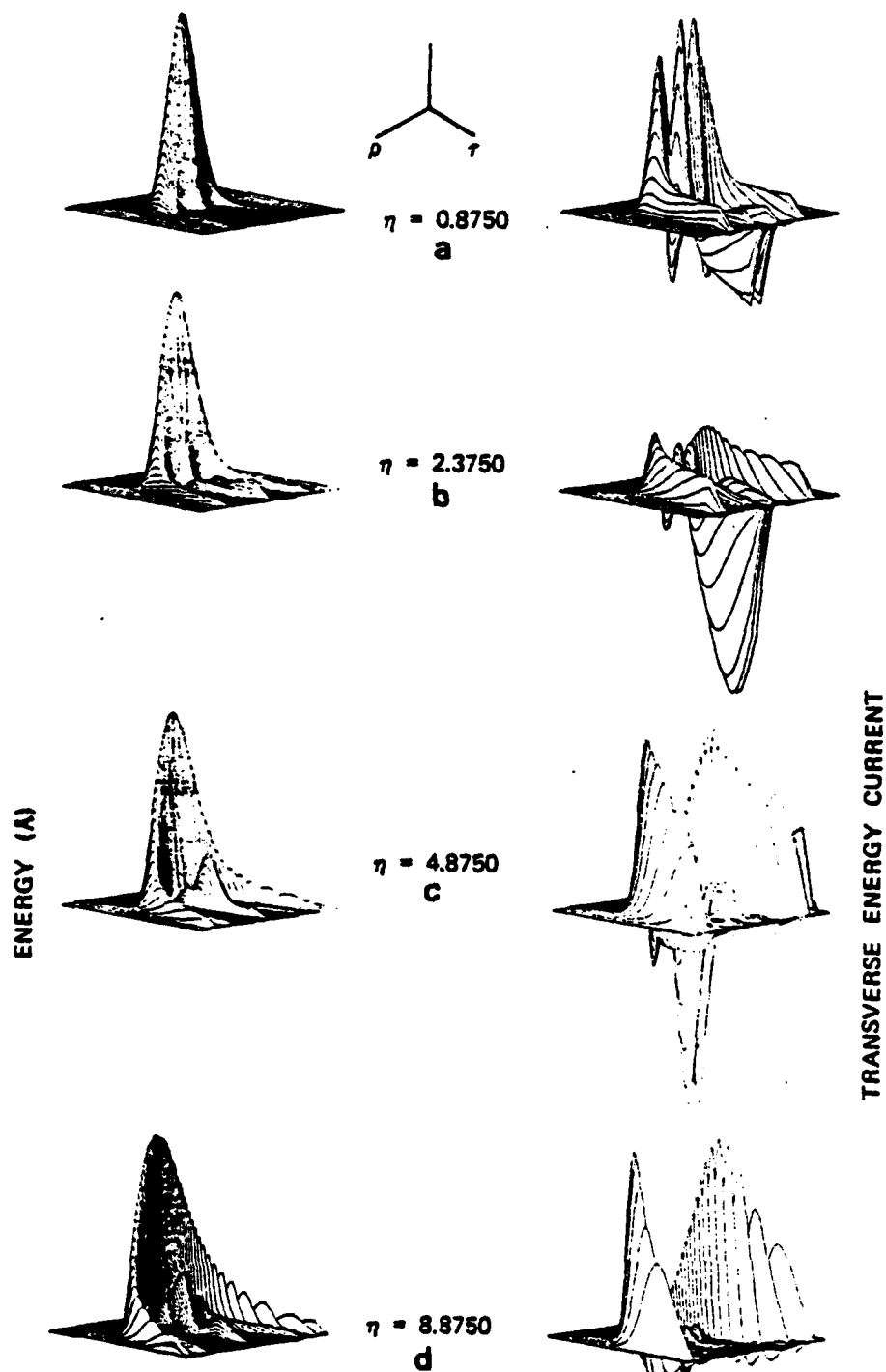
Fig. 18. Isometric plots of the amplifier field energy and transverse energy flow, against the retarded time for various transverse coordinates at four regions: (a) reshaping, (b) build-up region, (c) focal region, (d) post-focal region, with stretched radial coordinate for proper accounting of the transverse boundary condition.
