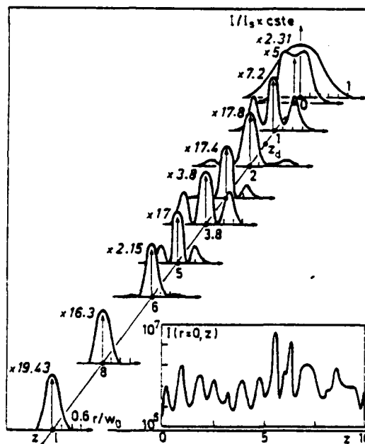
Figure 9. Transverse reshaping and on-axis intensity. I_0/I_s = 2.31 , \alpha_2 = 1 , \delta T = -1200 , z_d = 1.26 cm, F = 0.14 , z = 10 cm.
