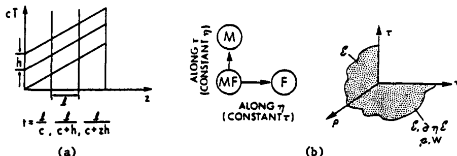
Fig. 6. Graph (a) displays the retarded time concept. Graph (b) outlines the numerical approach: a marching problem along \eta for the field simultaneously with a temporal upgrading of the material variables along \tau .
