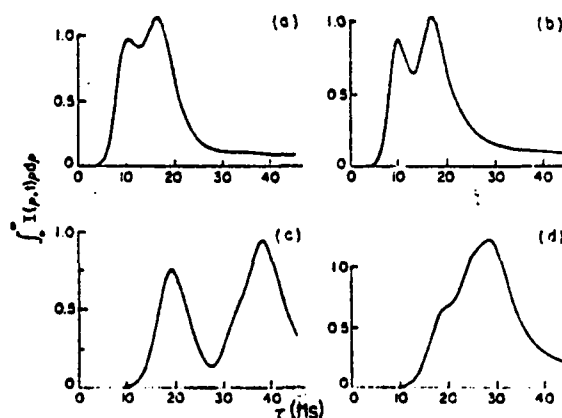
FIG. 7. Phase waves. Fluctuations can result in the second peak exceeding the first. n_0 = 9.5 \times 10^{10} \text{ cm}^{-1} . (a) F=1.49 , \langle \theta_0^2 \rangle^{1/2} = 1.21 \times 10^{-4} \text{ rad} ; (b) F=1.49 , \langle \theta_0^2 \rangle^{1/2} = 1.24 \times 10^{-4} \text{ rad} ; (c) F=0.165 , \langle \theta_0^2 \rangle^{1/2} = 2.22 \times 10^{-4} \text{ rad} ; (d) F=0.165 , \langle \theta_0^2 \rangle^{1/2} = 1.79 \times 10^{-4} \text{ rad} .
