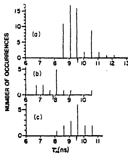
FIG. 5. Histogram showing the number of occurrences of a particular delay time. Points do not occur at integral values of \tau_D because of the nonlinear time mesh. (a) Plane-wave case for n_0^0 = 11.8 \times 10^{10} \text{ cm}^{-3} and \langle \theta_0^2 \rangle^{1/2} = 1.69 \times 10^{-4} rad. (b) and (c) Cylindrical-symmetric transverse case for n_0^0 = 18.2 \times 10^{10} \text{ cm}^{-3} , and \langle \theta_0^2 \rangle^{1/2} = 1.37 \times 10^{-4} rad. (b) F=1 . (c) F=\pi^{-1} . Each arrow denotes \tau_D .
