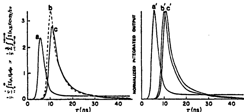
FIG. 8. Effect of Cartesian vs cylindrical geometry for the sum over shots of the transversely integrated intensity for quantum-fluctuation calculations. Curve a holds for F=1.37 for a Cartesian geometry. F=0.11 for both curves b and c; curve b involves cylindrical geometry while curve c is Cartesian (parallelepiped). Note that the delay with F=1.37 (curve a) is shorter than the delay with F=0.11 (curve c), just as it was for cylindrical geometry and no fluctuations (Ref. 16). Strong diffraction increases the delay because of energy lost transversely, but the tail is greatly reduced because the diffraction makes the sample superfluoresce as a unit. Curves a'—c' show the same curves normalized for pulse-shape comparisons. n_0 = 18.2 \times 10^{10} \text{ cm}^{-1} and \langle \theta_0^2 \rangle^{1/2} is about 1.56 \times 10^{-4} \text{ rad} .
