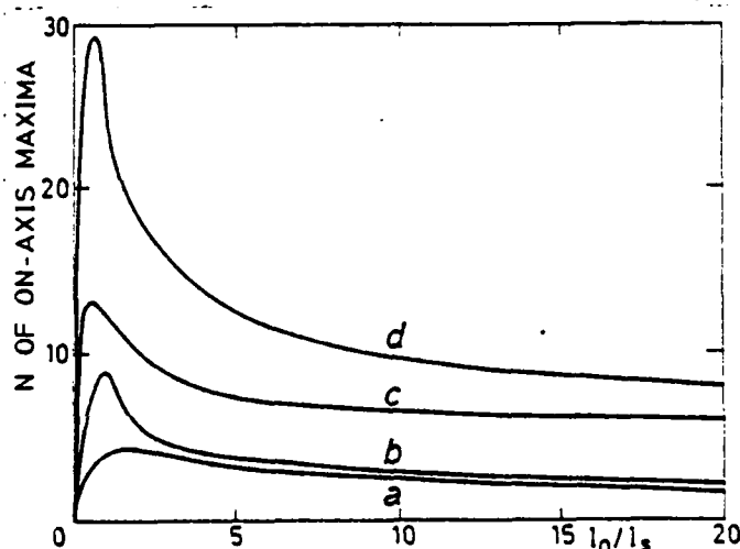
Figure 6. Number of on-axis maxima as a function of I_0/I_s , for same parameters as in Fig. 5, and for different T_2 : a) -60, b) -120, c) -250, d) -500.
