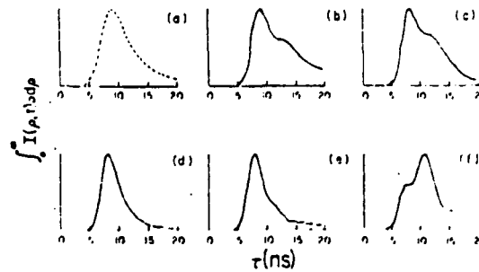
FIG. 2. Intensity integrated over the transverse cylindrical coordinate as a function of time for single trajectories. (a) Cs data for n_0^0 \approx 7.6 \times 10^{10} \text{ cm}^{-3} . (b) Simulation with transverse effects, but no fluctuations: n_0^0 = 18.2 \times 10^{10} \text{ cm}^{-3} , \theta_0 = 1.37 \times 10^{-4} rad, and Fresnel number F=1 . (c)-(f) Simulations with transverse effects and fluctuations for n_0^0 = 18.2 \times 10^{10} \text{ cm}^{-3} , \langle \theta_0^2 \rangle^{1/2} = 1.37 \times 10^{-4} rad, and F=1 .
