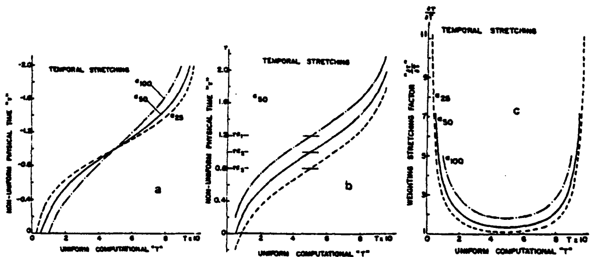
Fig. 9. Dependence of prescribed stretching and its derivatives on the point densities and the centre of transformation.
