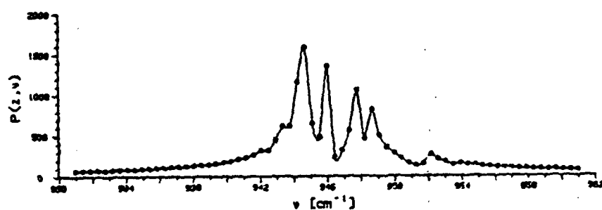
Figure 3: Power spectrum of the field shown in Fig. 2. The units of the vertical axis are (\text{sV cm}^{-1})^2 , and the resolution of the numerical Fourier transform is 0.44 \text{ cm}^{-1} . The initial time t_0 was taken as zero in Eq. (48).
