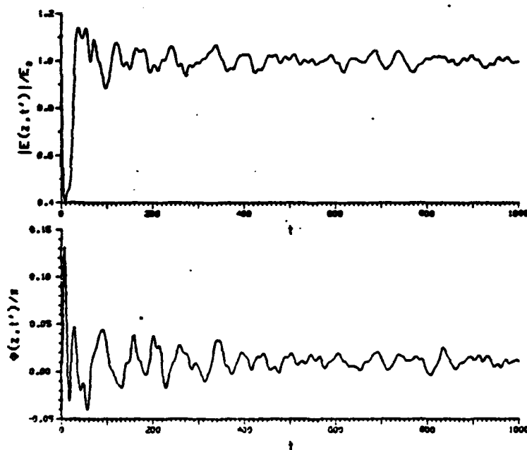
Figure 2: The normalized amplitude and phase of \tilde{E}(z, t') for z = 50 cm, and for the ten-level system shown in [8(a)], Fig. 1. Parameters are: \langle \mu_{01} \rangle = 0.388 D, N = 3.54 \times 10^{15} \text{ cm}^{-3} , E_0 = 10^3 \text{ sV cm}^{-1} ( 3.1 \times 10^3 \text{ V cm}^{-1} ), X_{33} = -2.54 \text{ cm}^{-1} , G_{33} = 0.303 \text{ cm}^{-1} , T_{33} = 0 , J_0 = 68 , v_g/c \approx \omega/2\pi c = 946 \text{ cm}^{-1} .
