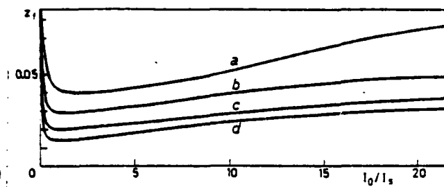
Figure 8. First focus as a function of I_0/I_s for same parameters as in Figs. 6 and 7.
