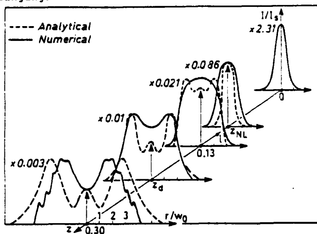
Figure 2. Transverse reshaping; same parameters as in Fig. 1, except F = 8.8 , l = 0.1 cm, z_{NL} = 0.08 cm/
