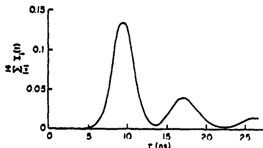
FIG. 1. Intensity as a function of time for the average of 14 output pulses in the plane-wave case with quantum fluctuations such that (\theta_0^2)^{1/2} = 1.69 \times 10^{-4} rad and n_0^0 = 11.8 \times 10^{10} \text{ cm}^{-3} .
