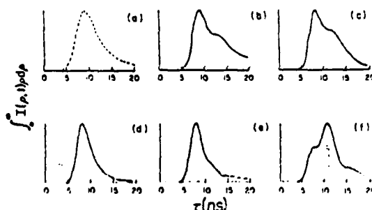
FIG. 2. Intensity integrated over the transverse cylindrical coordinate as a function of time for single trajectories. (a) Cs data for n_0^0 = 7.6 \times 10^{10} \text{ cm}^{-3} . (b) Simulation with transverse effects, but no fluctuations: n_0^0 = 18.2 \times 10^{10} \text{ cm}^{-3} , \theta_0 = 1.37 \times 10^{-4} rad, and Fresnel number F = 1 . (c)-(f) Simulations with transverse effects and fluctuations for n_0^0 = 18.2 \times 10^{10} \text{ cm}^{-3} , (\theta_0^2)^{1/2} = 1.37 \times 10^{-4} rad, and F = 1 .
