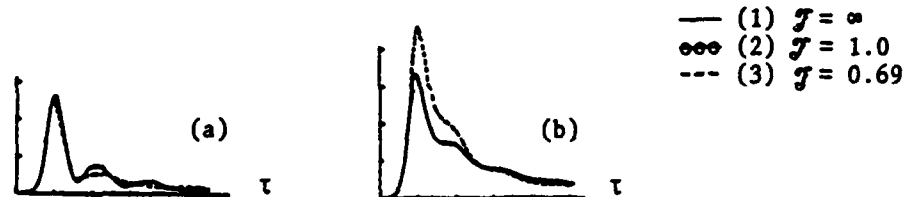
Fig. 24. (a) Propagation of small-area Gaussian profile pulse through uniform cylinders ( \tau_R = 0.046 ns, L/L_c = 1.35 and \theta_R = 3 \times 10^{-3} on-axis). (b) Superfluorescence with Gaussian radial gain ( \tau_R = 0.046 ns, L/L_c = 1.35 and \theta_R = 3 \times 10^{-3} on-axis).
