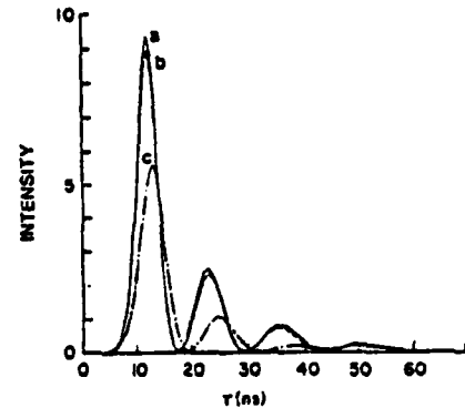
FIG. 10. Effects of inhomogeneous broadening in the uniform plane-wave case with homogeneous initial tipping angle. a: T_2^* = \infty . b and c: T_2^* = 32 \text{ ns} in the formulas (for b) g(\Delta\omega) = (T_2^*/\pi) \exp[-(T_2^*(\Delta\omega)/\sqrt{\pi})^2] and (for c) g(\Delta\omega) = (T_2^*/\pi^{3/2}) \{1 + [T_2^*(\Delta\omega)/\sqrt{\pi}]^2\}^{-1} corresponding closely to the value in the Cs experiment. Notice that including T_2^* damps the field energy amplitude and reduces the tail. Delay is also affected slightly. n_0^0 = 9.5 \times 10^{10} \text{ cm}^{-3} and \theta_0 = 1.89 \times 10^{-4} \text{ rad} .
