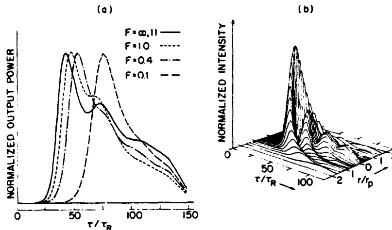
FIG. 2. Influence of diffraction on SF pulse shapes. Parameters are the same as in Fig. 1(a), with n_0 Gaussian and \theta_0 uniform. (a) Emitted power; (b) isometric graph of intensity for the F = 1 case of (a).
