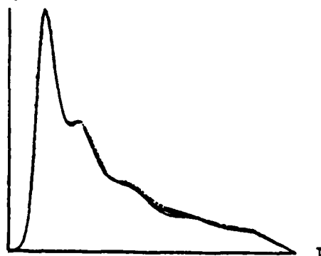
Fig. 31. Display of small-ripple effects in the Gaussian inversion of the cylinder on the total energy per unit atom (versus time) for \mathcal{F} = 0.7 , \tau_R = 0.46 ns, and L/L_c = 1.95 .
