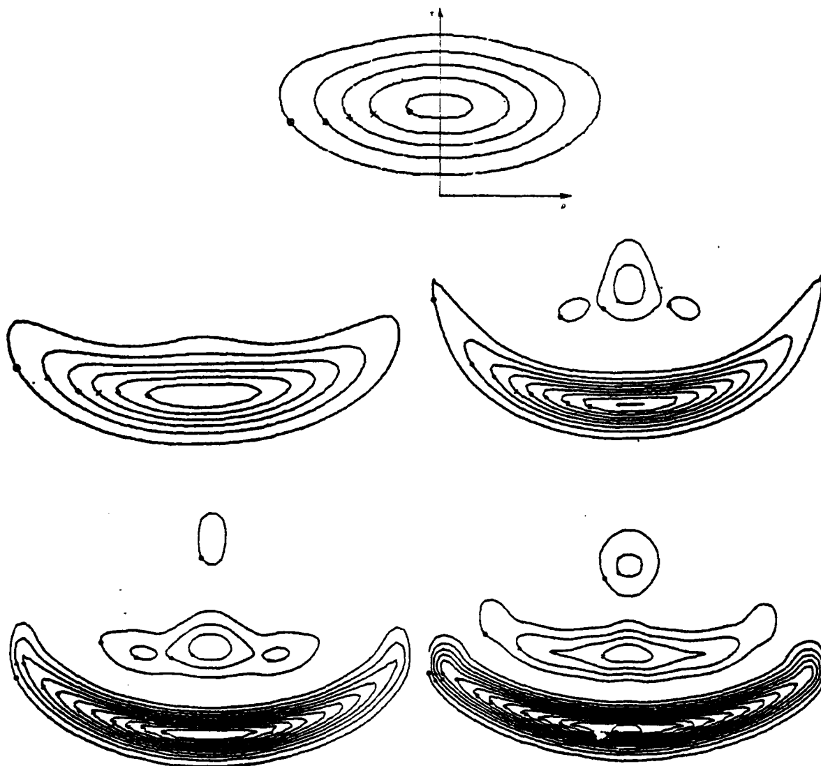
Fig. 17. Amplifier field energy contour plots for the four propagation regions of interest. Notice the temporal advance associated with the coherent exchange of energy between light and matter, as well as the beam cross-section narrowing.
