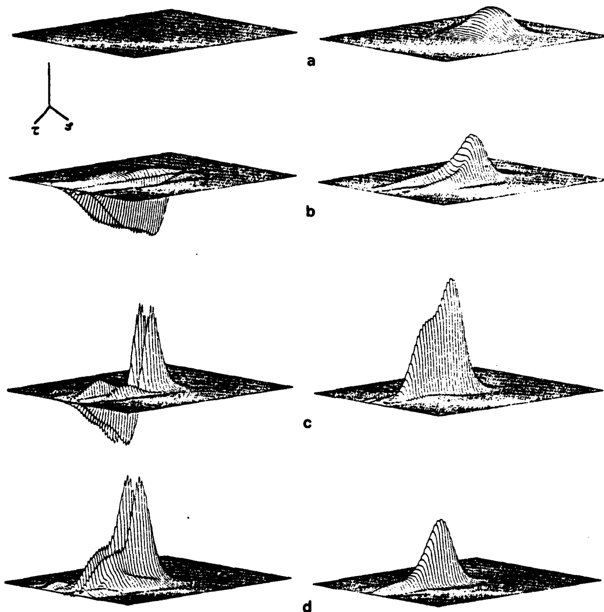
Fig. 14. Isometric plots of the absorber field energy and transverse energy flow profile for various time slices at the four regions of interest.
