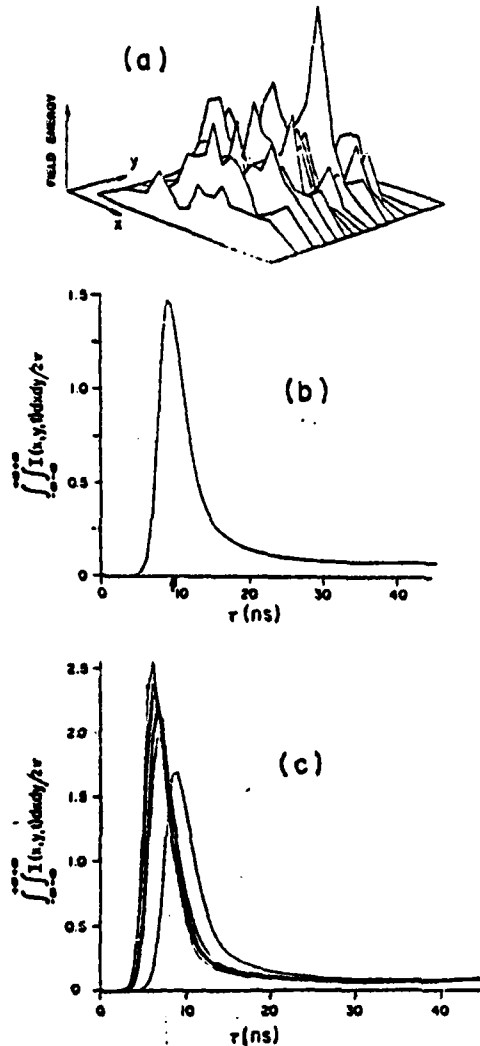
FIG. 9. Transverse fluctuations for a full three-spatial-dimension calculation with quantum initiation. (a) Field energy is displayed isometrically at a time near the peak of the pulse [see arrow, Fig. 9(b)]. In (b) the transversely integrated energy is displayed. (c) Comparison of seven output energy profiles. F=1.37 , n_0^0=18.2 \times 10^{10} \text{ cm}^{-3} , and (\theta_0^0)^{1/2}=1.56 \times 10^{-4} \text{ rad} . Actually (a) and (b) were calculated for L=1.86 \text{ cm} and (c) for L=2 \text{ cm} .
