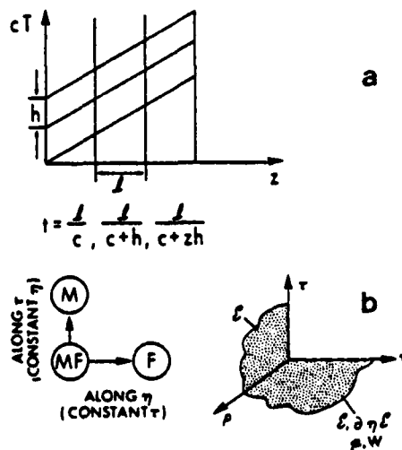
Fig. 5. Graph (a) displays the retarded time concept; (b) outlines the numerical approach: a marching problem along \eta for the field simultaneously with a temporal up-grading of the material variables along \tau .
