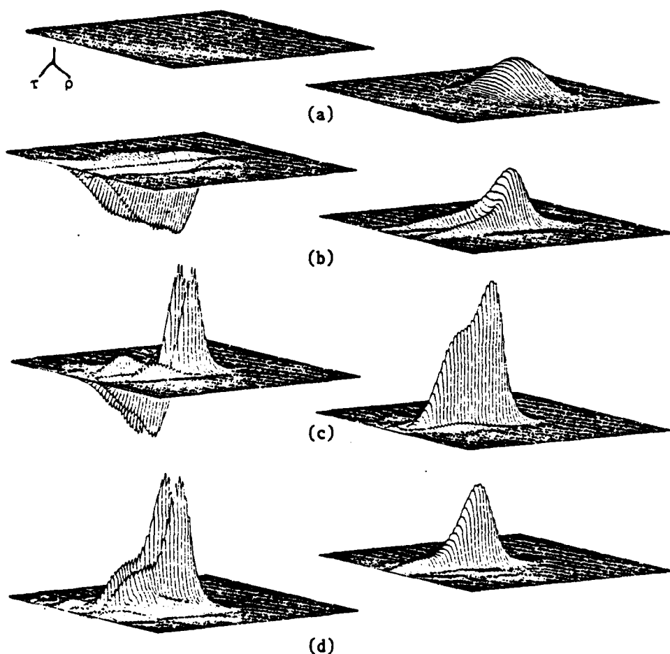
Fig. 16 Isometric plots of the absorber field energy and transverse energy flow profile for various time slices at the four regions of interest.
