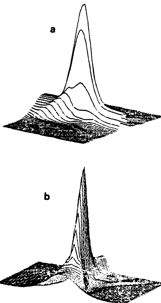
Fig. 12. The energy per unit area \{\int \delta |e(\rho, \eta, r)|^2 dr\} the fluency is displayed as a function of the distance in the direction of propagation for various values of the coordinates transverse to the direction of propagation. To illustrate the gradual inward energy flow the \pi/2 reorientation is also displayed. The longitudinal orientation illustrates the gradual boosting mechanism that the field energy experiences as it flows radially towards the beam axis (while \eta increases). The second angle displays the severe beam distortion in its cross-section as a function of \eta .
