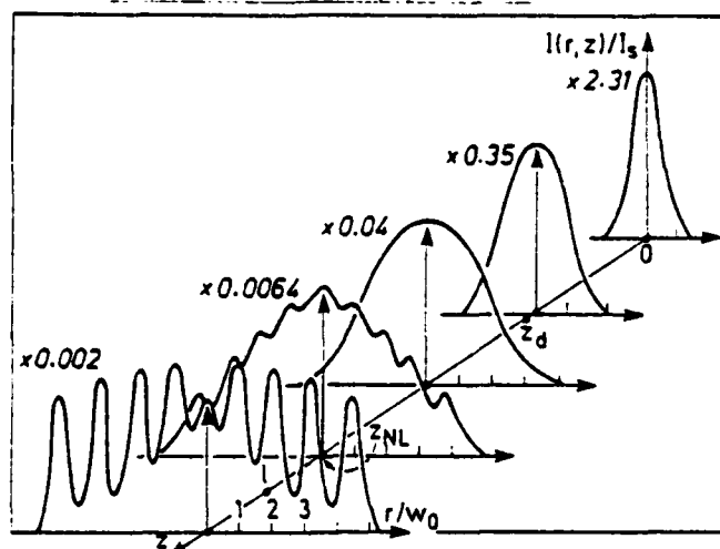
Figure 4. Transverse reshaping, same parameters as in Figs. 1 and 2, except F = 1.25 , l = 0.7 cm, z_{NL} = 0.6 cm.
