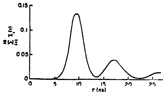
FIG. 1. Intensity as a function of time for the average of 14 output pulses in the plane-wave case with quantum fluctuations such that \langle \theta_0^2 \rangle^{1/2} = 1.69 \times 10^{-4} rad and n_0^0 = 11.8 \times 10^{10} \text{ cm}^{-3} .
