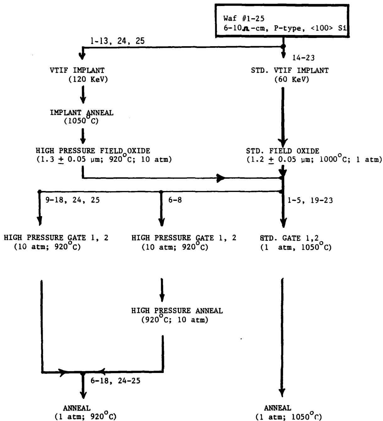
FIGURE 20: Process matrix for Batch JE08B
