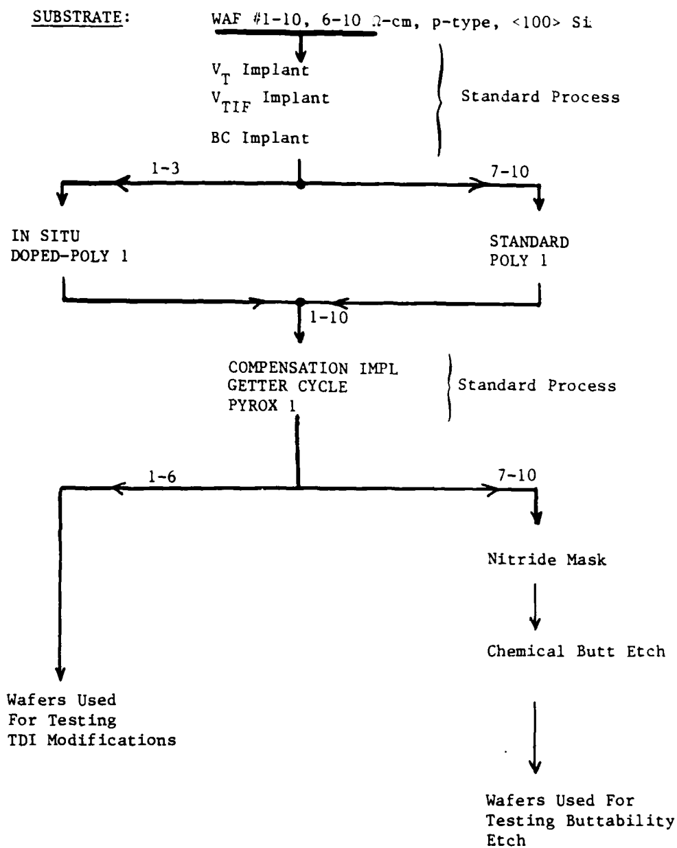
FIGURE 4: Salient features of process matrix for Batch 1 (JE07A)
