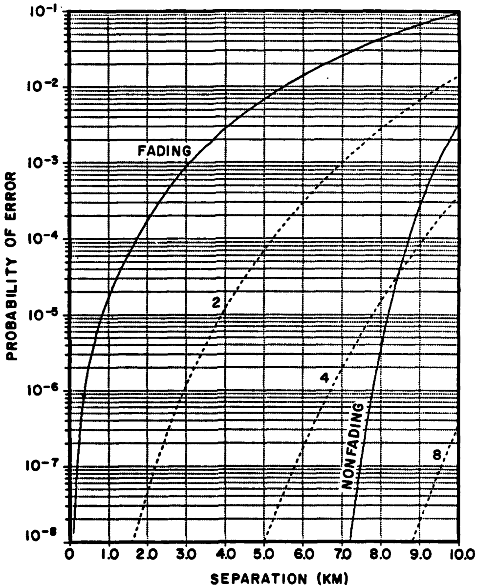
Figure 23 Coherent MSK (with maximal ratio combining) probability of error as a function of range for a 0.5 watt link composed of a directional transmitter (15 cm maximum) and an omni-directional receiver operating at optimum frequency. The effects of fading and diversity are illustrated.
