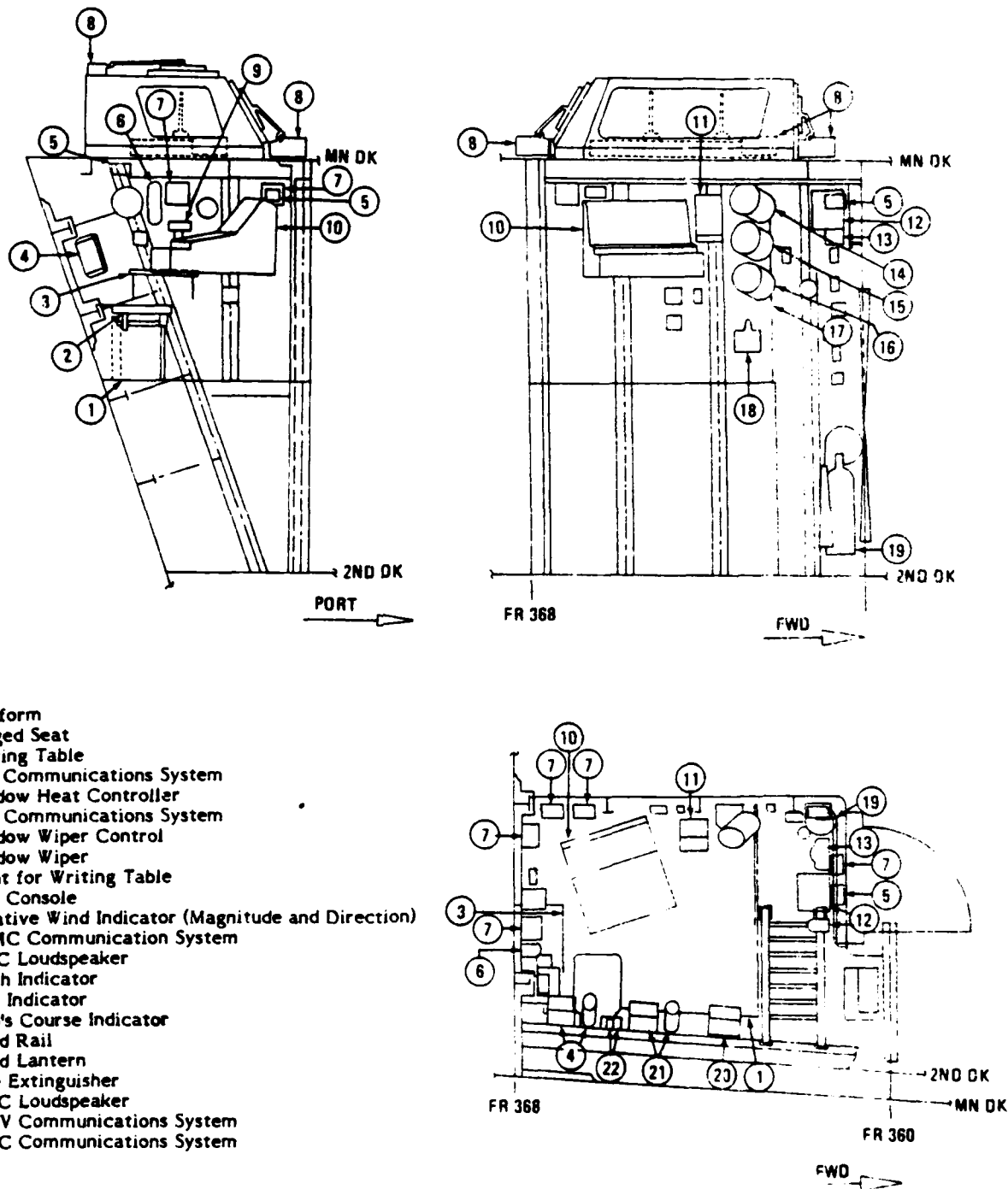
Figure 6 LSO Station Layout on the FFG-8 (Obtained from Redesign Agency, GIBBS&COX INC., NEW YORK, N.Y.)
