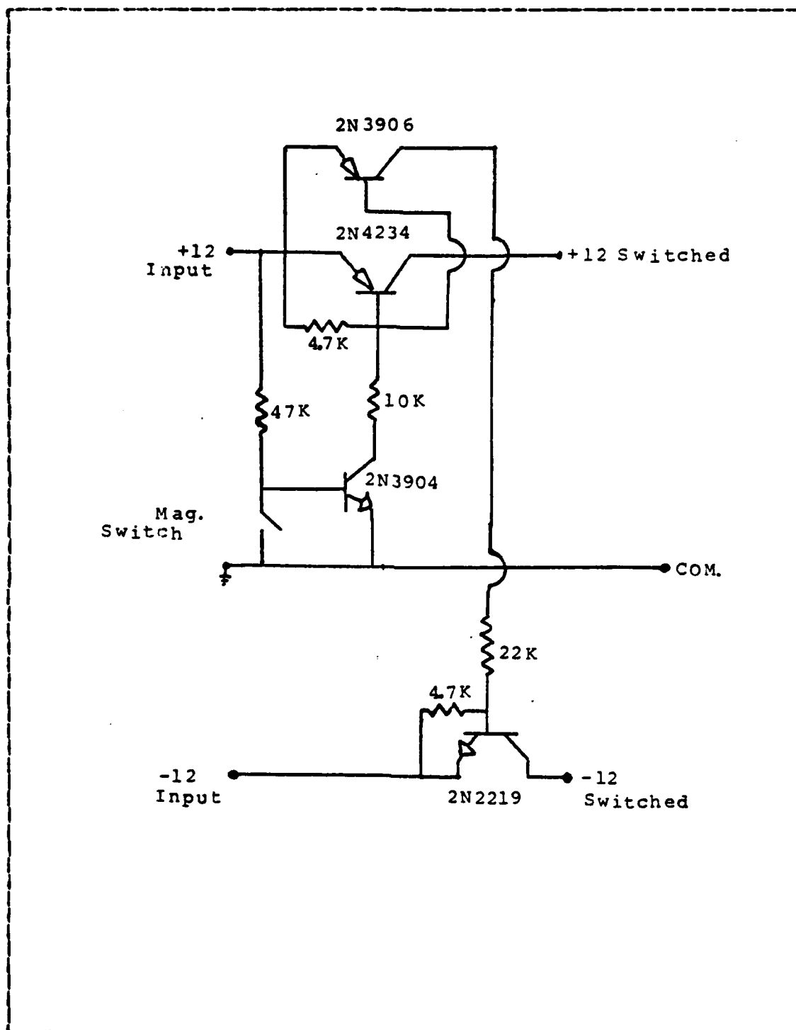
Figure A.2 Magnetic Activation Circuit
