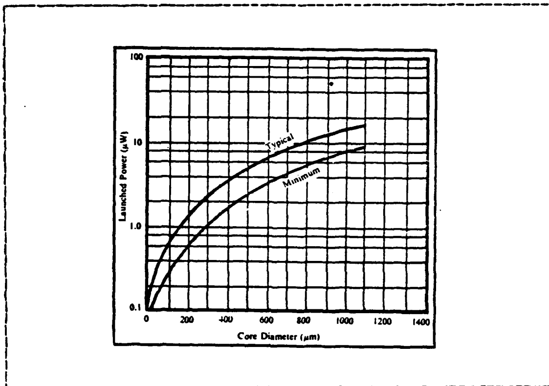
Figure 3.4 Launched Power vs. Core Diameter
