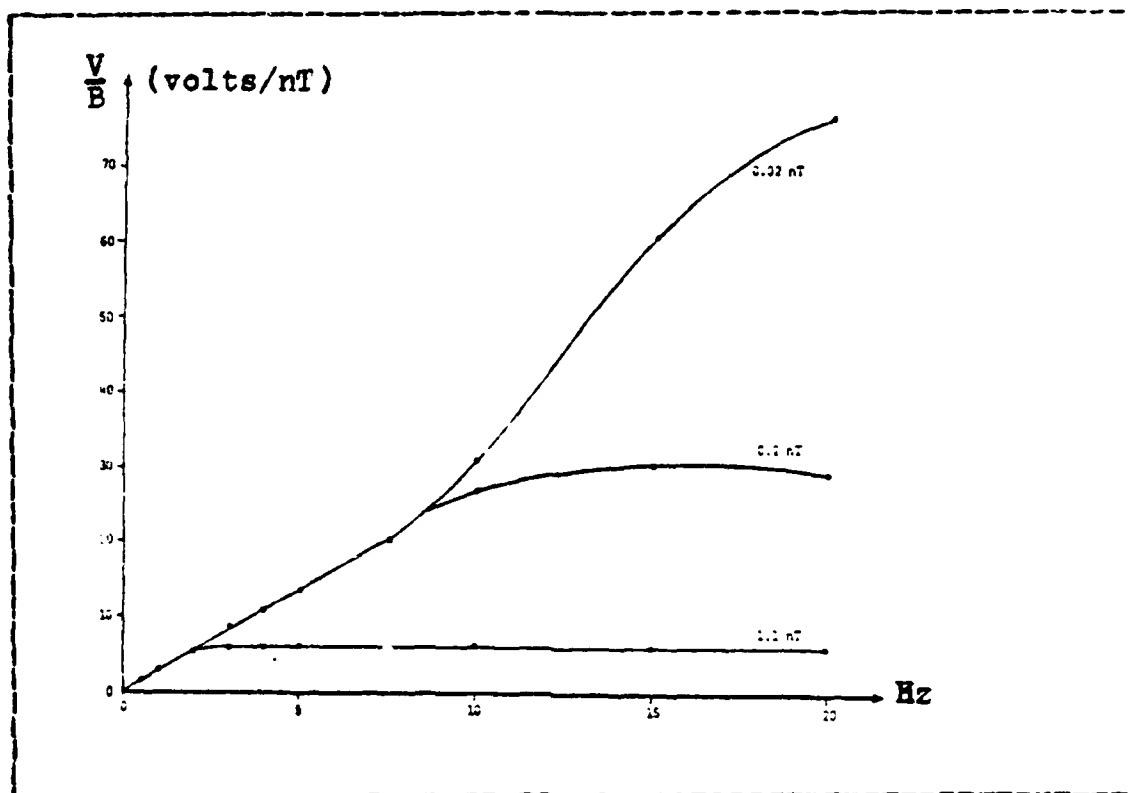
Figure C.16 Ocean System Y-Coil Calibration
