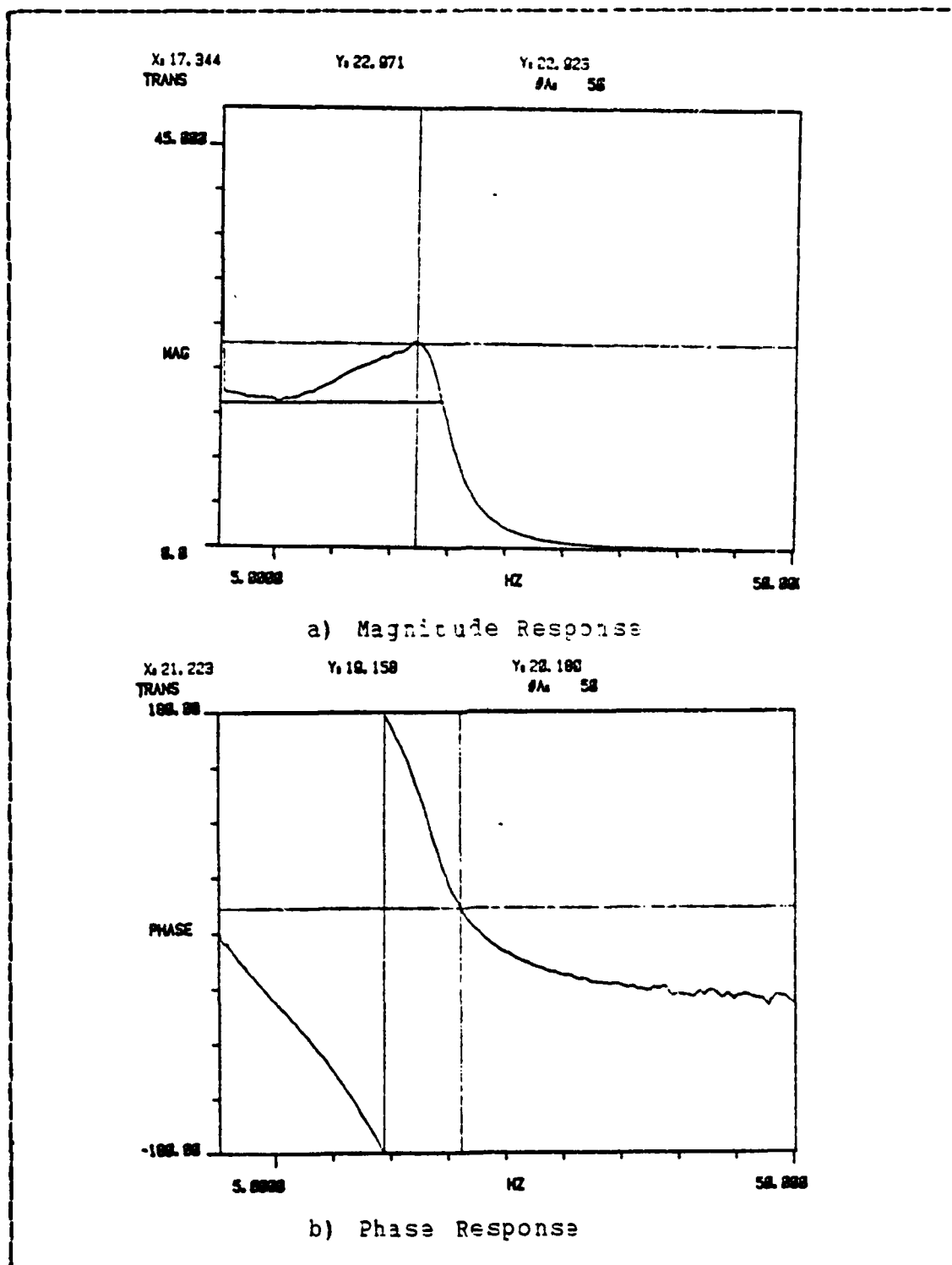
Figure C.6 Response of the Ocean X System
