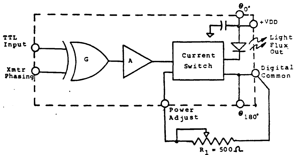
a) Optical Transmitter Block Diagram
