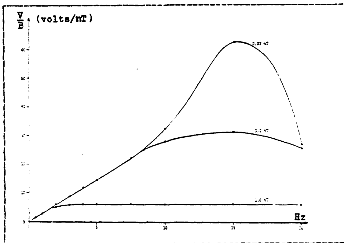
Figure C.14 Land System Z-Coil Calibration
