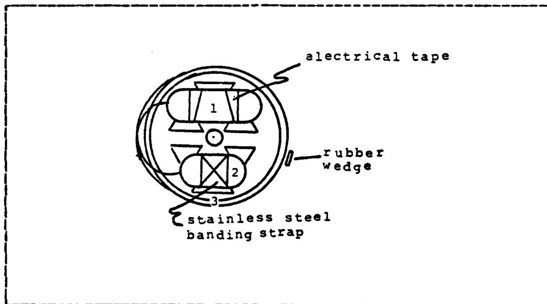
Figure B.2 Fiber Optic Enclosures (1) and (2), and storage reel (3).
