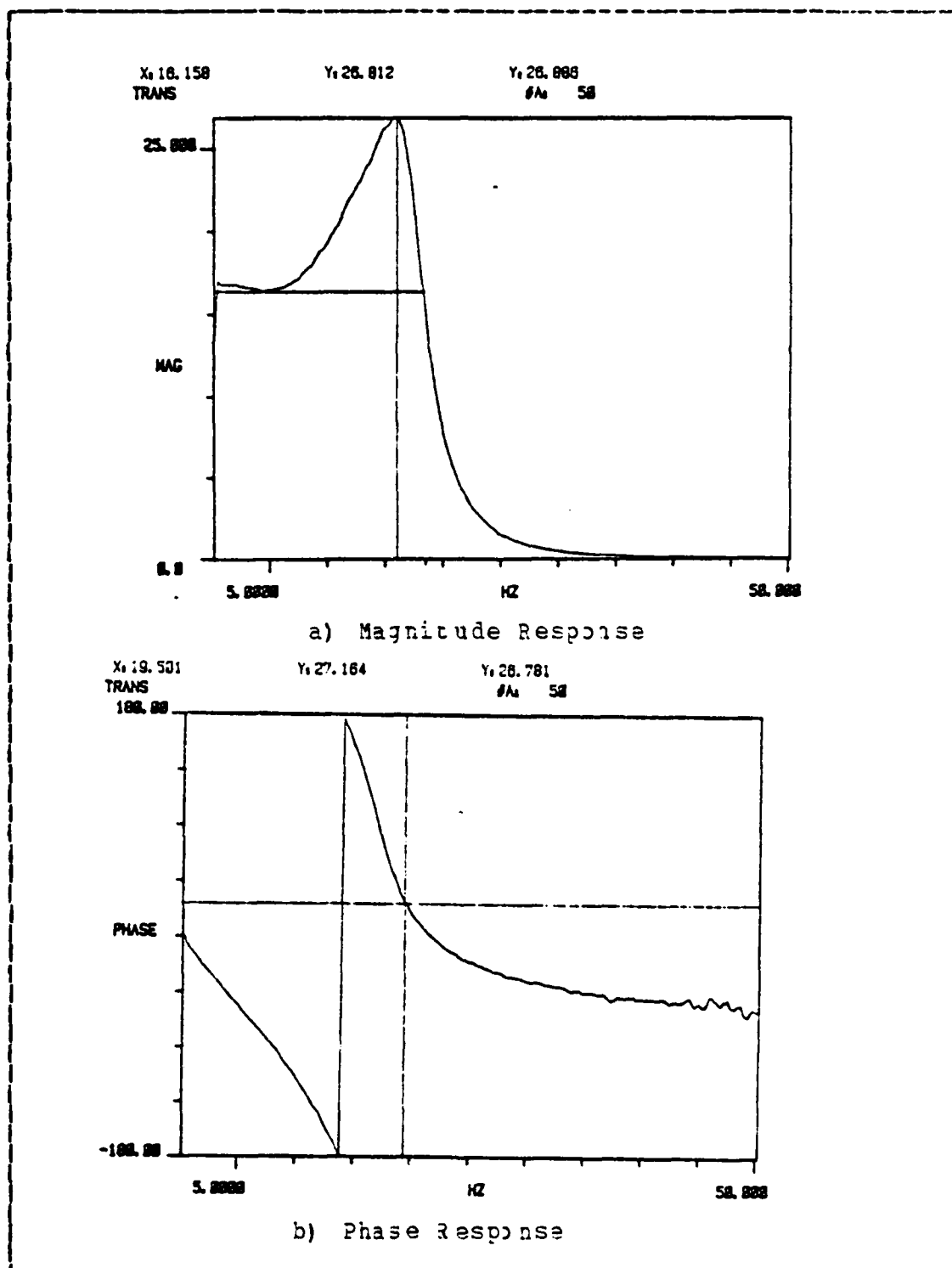
Figure C.4 Response of the Land Y System
