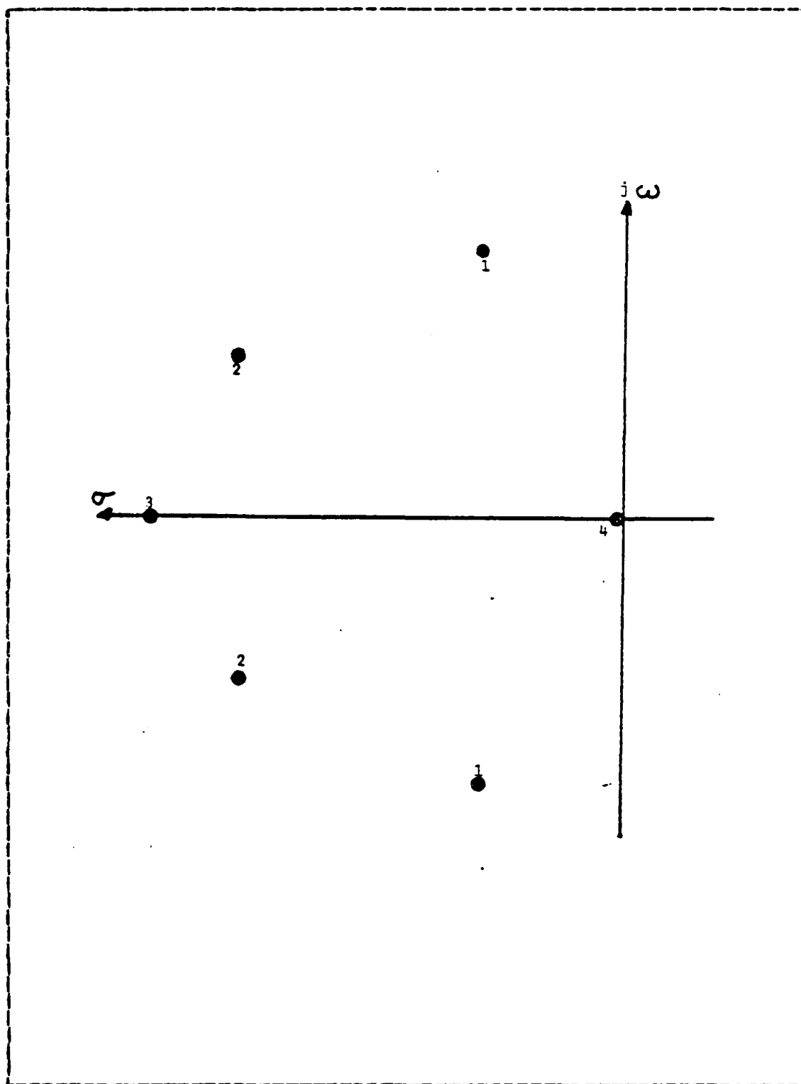
Figure C.2 Pole-Zero Diagram for Model 13-10A Amplifier
