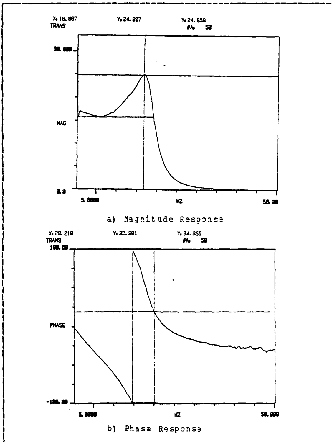
Figure C.3 Response of the Land X System
