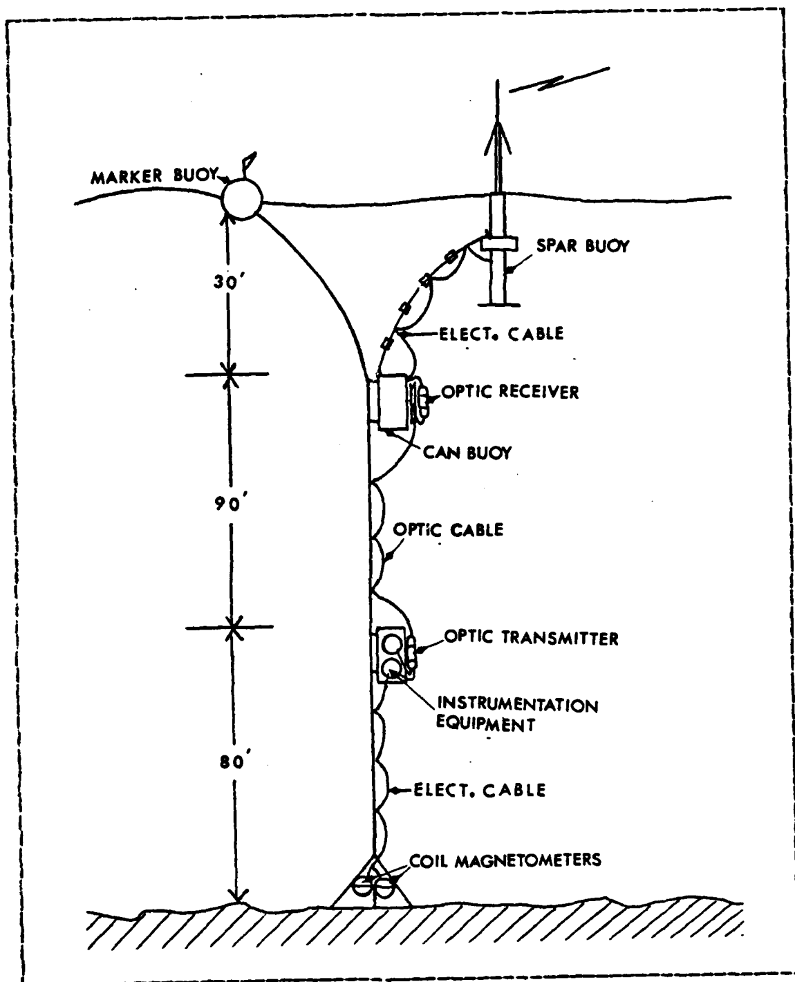
Figure 2.1 Diagram of Deployed Generation II System
