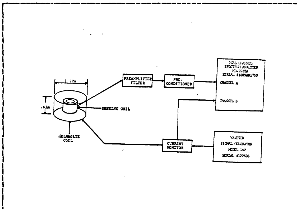
Figure C. 10 System Calibration Experiment
