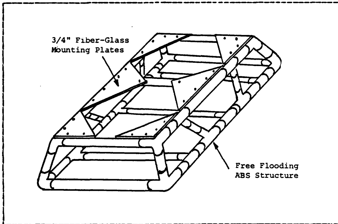
Figure 2.3 Sensor Subsystem Equipment Mounting Assembly
