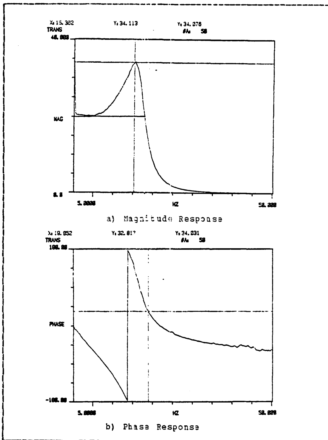
Figure C.8 Response of the Ocean Z System
