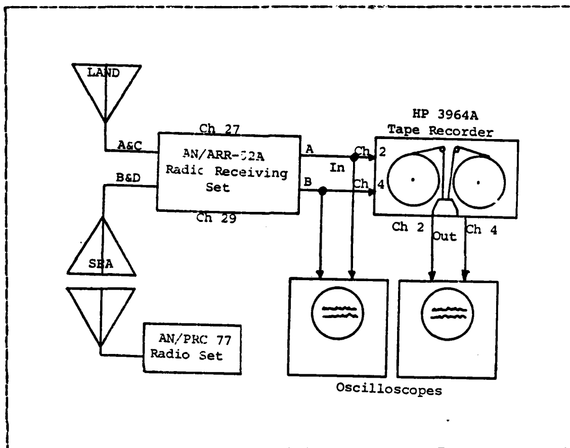
Figure 2.13 Receiving Station Equipment Configuration
