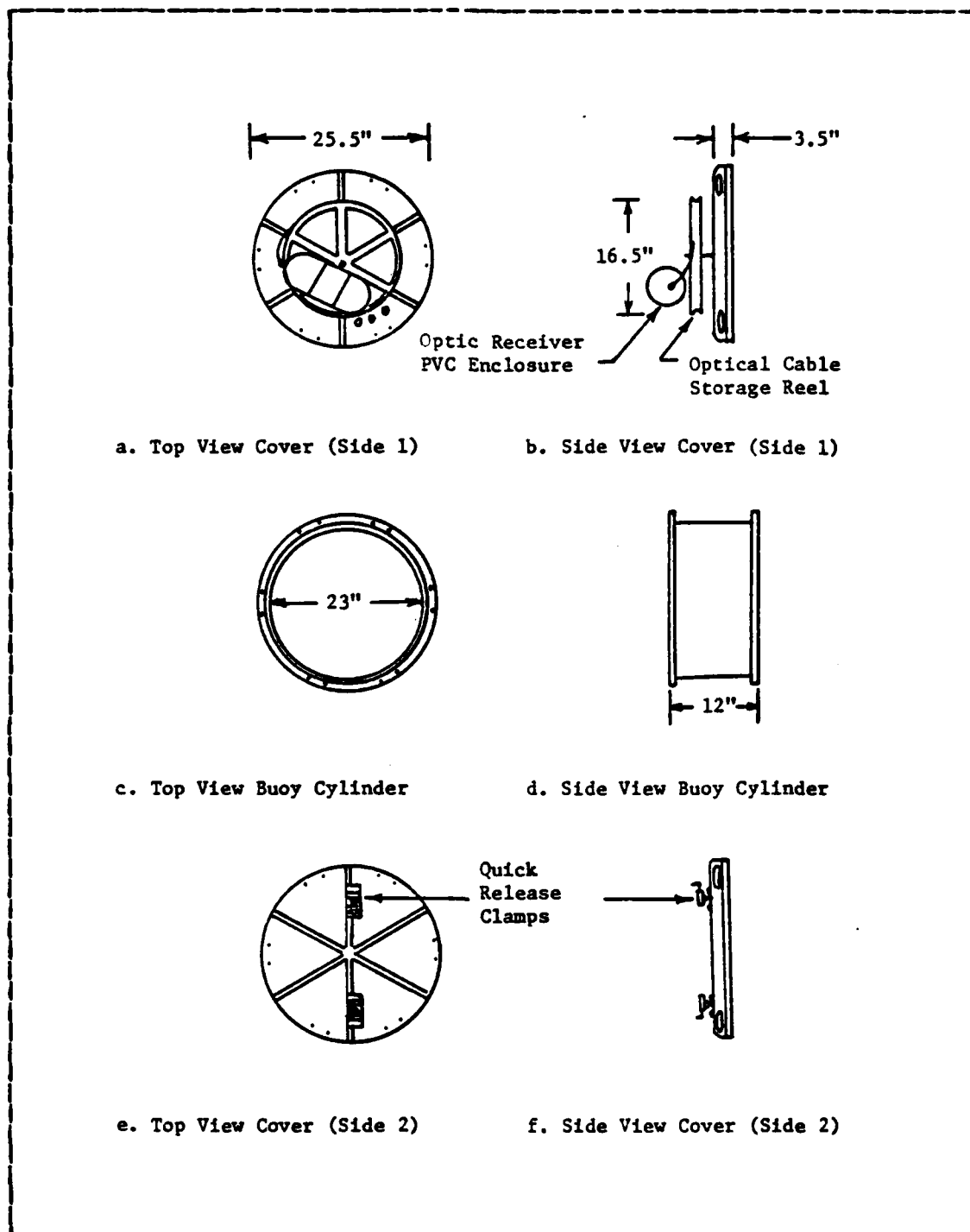
Figure 2.7 Diagram of Can Buoy and Optic Receiver Assembly
