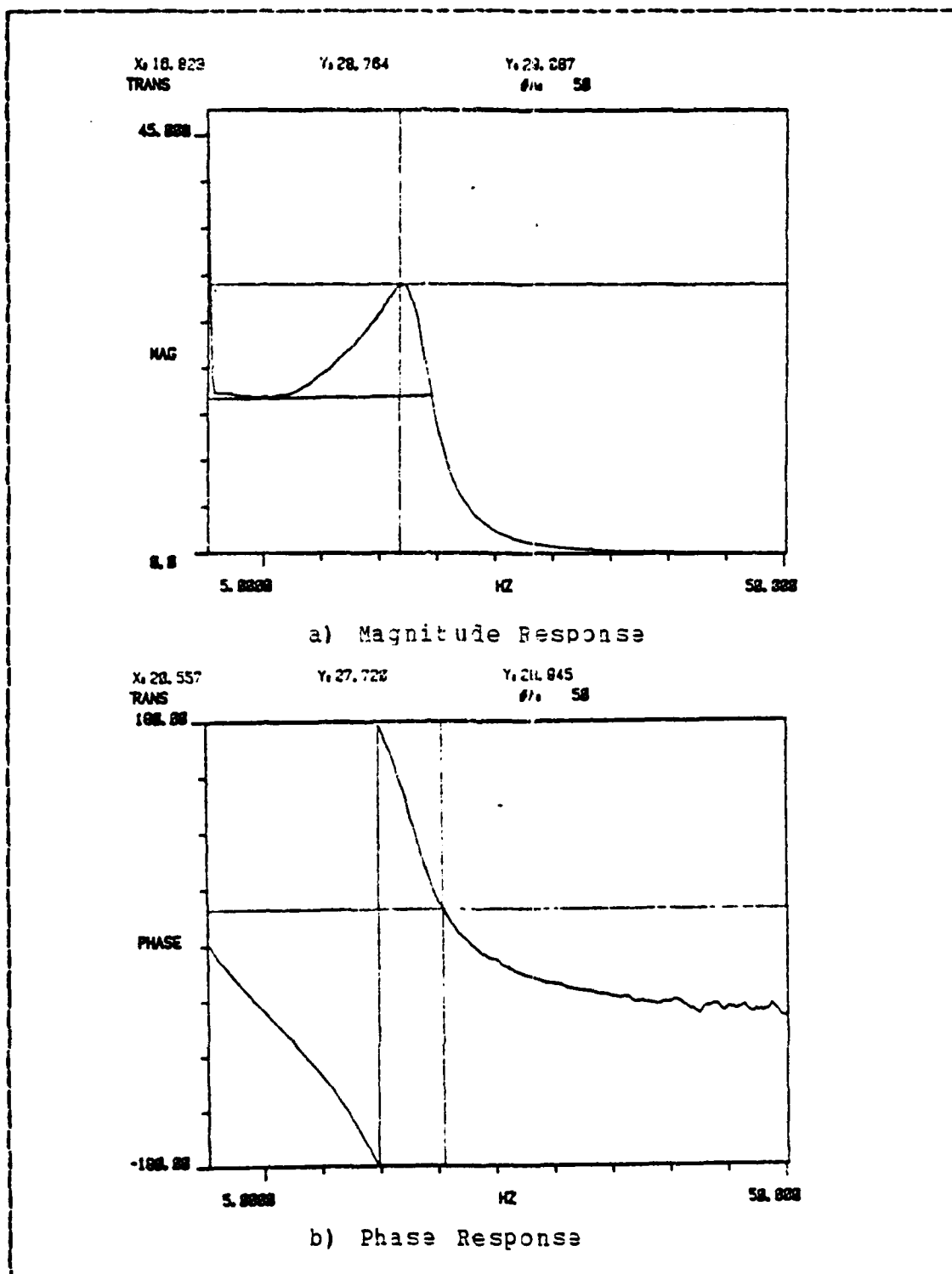
Figure C.7 Response of the Ocean Y System
