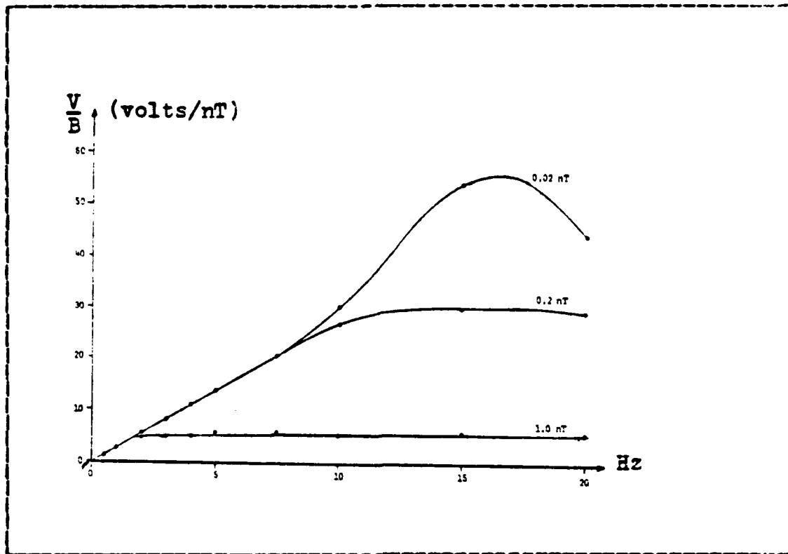
Figure C.15 Ocean System X-Coil Calibration
