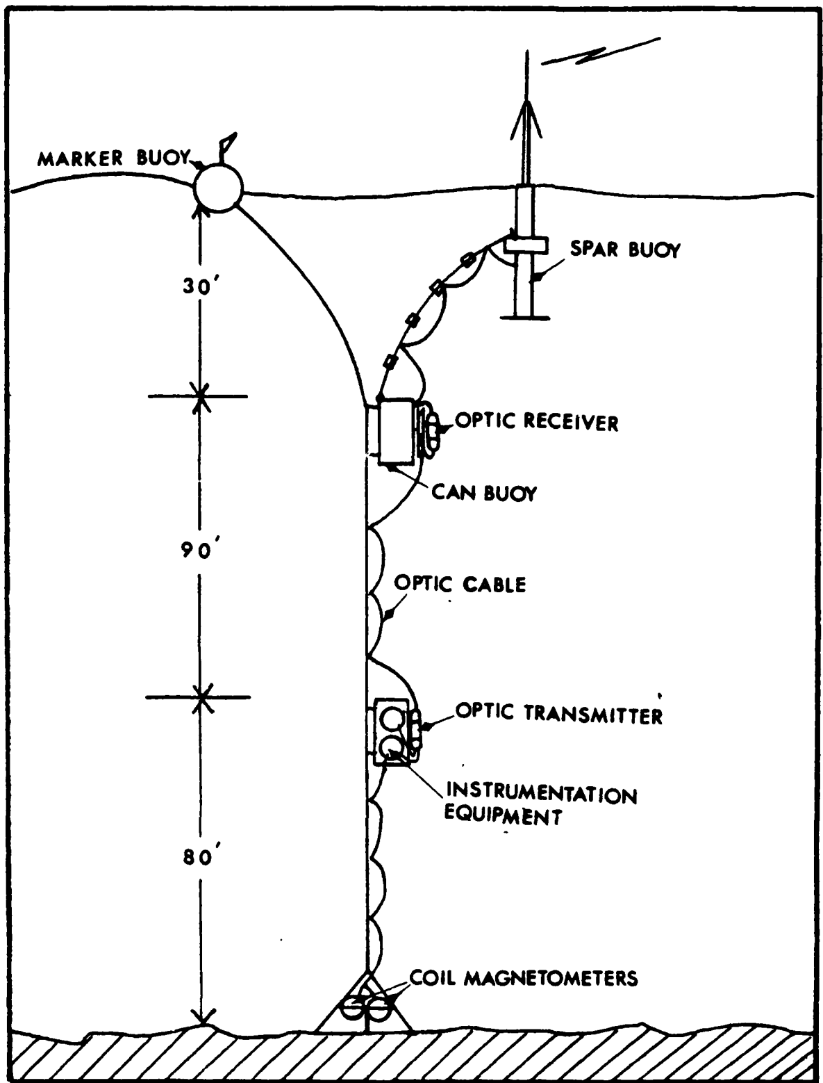
Figure 3.2 Ocean Data Collection System
