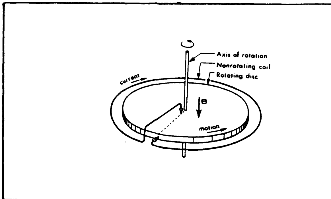
Figure 2.2 Simple Disk Dynamo
