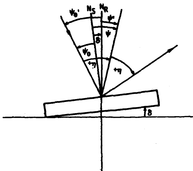
Figure 1. Schematic drawing of X-ray diffraction geometry for the Rigaku Strainflex system.
