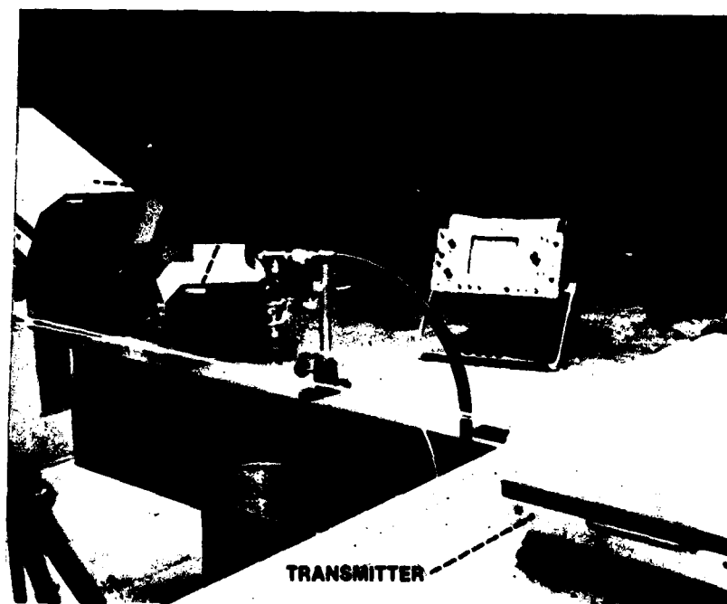
Figure 7. - Photograph of components of Droplet Sizing Interferometer instrument with Lexel HVPS in place.
