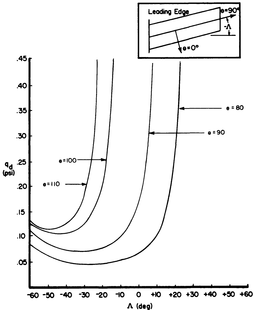
Figure 10. Design Curves; q_d as a Function of Sweep for Fiber Orientations of 80°, 90°, 100°, and 110°
