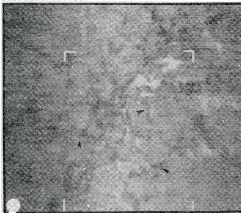
Figure 4. Areas of rafted thin ice show higher T_B than unrafted areas.
