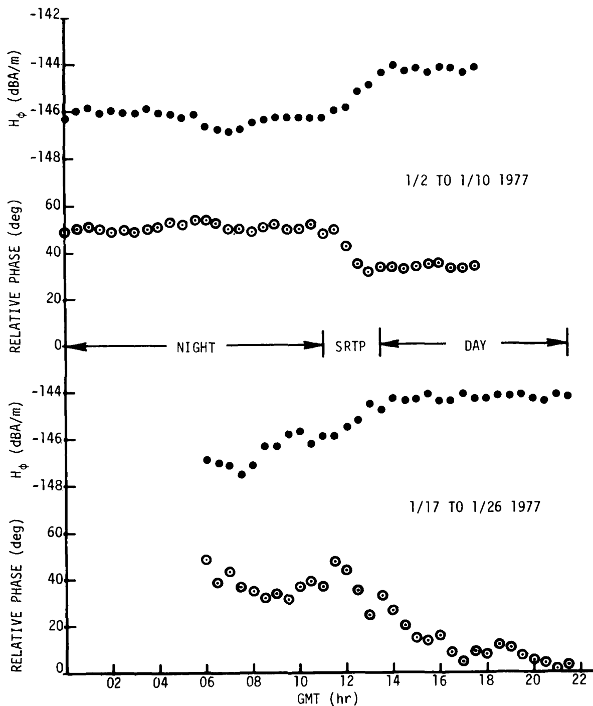
Figure 11. Connecticut Field-Strength Averages Versus GMT, 2 to 10 and 17 to 26 January 1977
