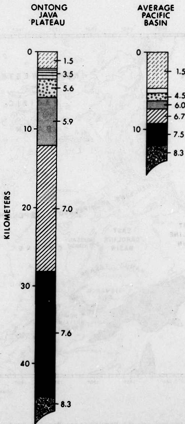
Fig. 7. Section profiles for the Ontong-Java Plateau and Pacific Basin (from Hussong et al. 1979).
