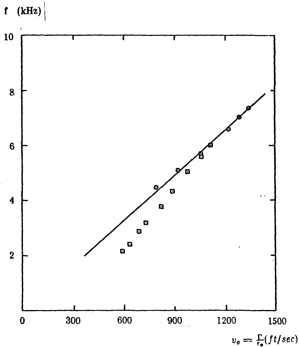
Figure 1. Fundamental frequency for solid main tube. ————calculated; \square , L = 1.65 \text{ in.} ; \circ , L = 0.5 \text{ in.} (Taken from Figure 6, Ref. 6, Section 6.)
