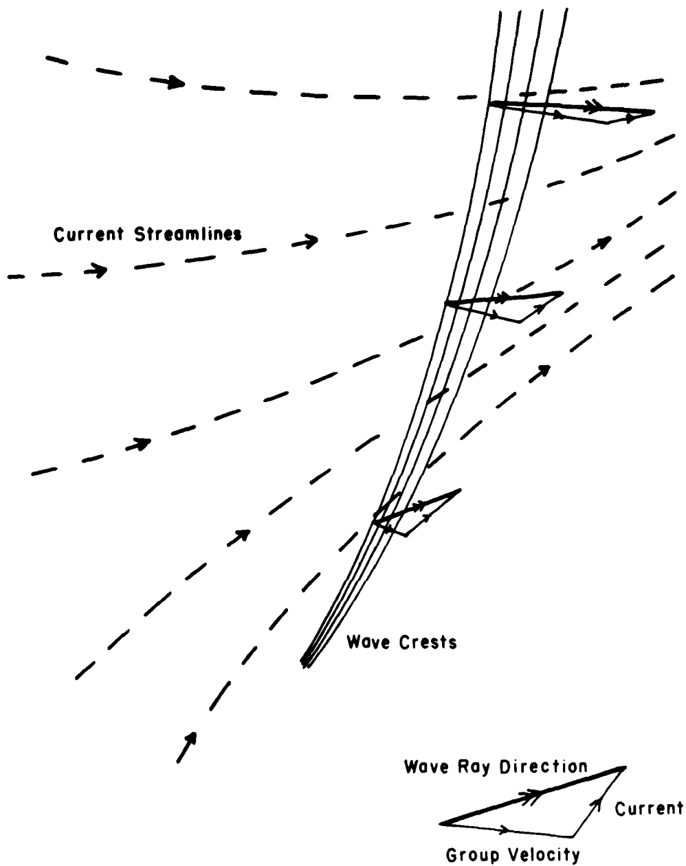
Figure 5. Direction of rays as vector sum of current plus group velocity. Drawing shows sea surface viewed from above.
