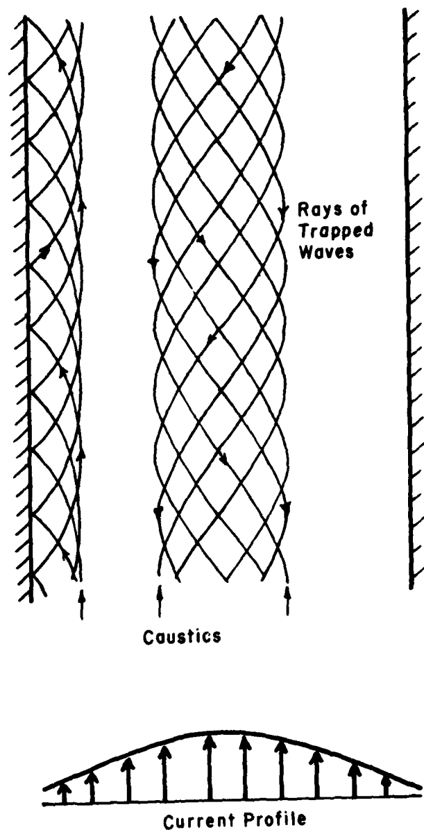
Figure 7. Rays in a nonuniform stream in a channel, showing two sets of trapped waves and their corresponding caustics.
