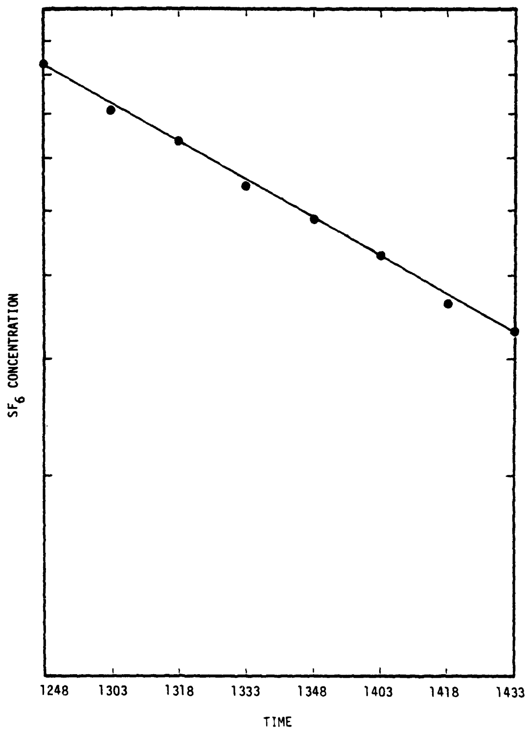
Figure B.5b Tracer Concentration Decay versus Time on 12/4/79 (P.M.) for Apartment No. 8121.
