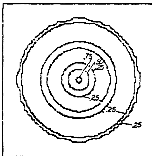
Figure 3.4 CONTOUR II Plot of a Single Sonobuoy Detection Probability
