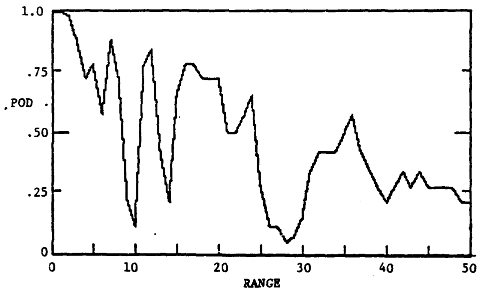
Figure 4.12. Probability of Detection IOC050DDS FOM: 85 Sigma: 5
