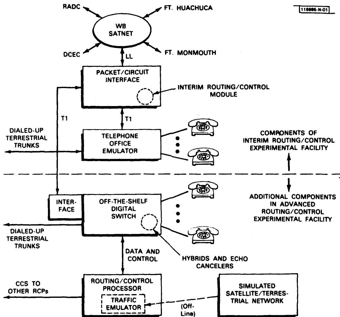
Fig. 17. Planned EISN site equipment configurations.
