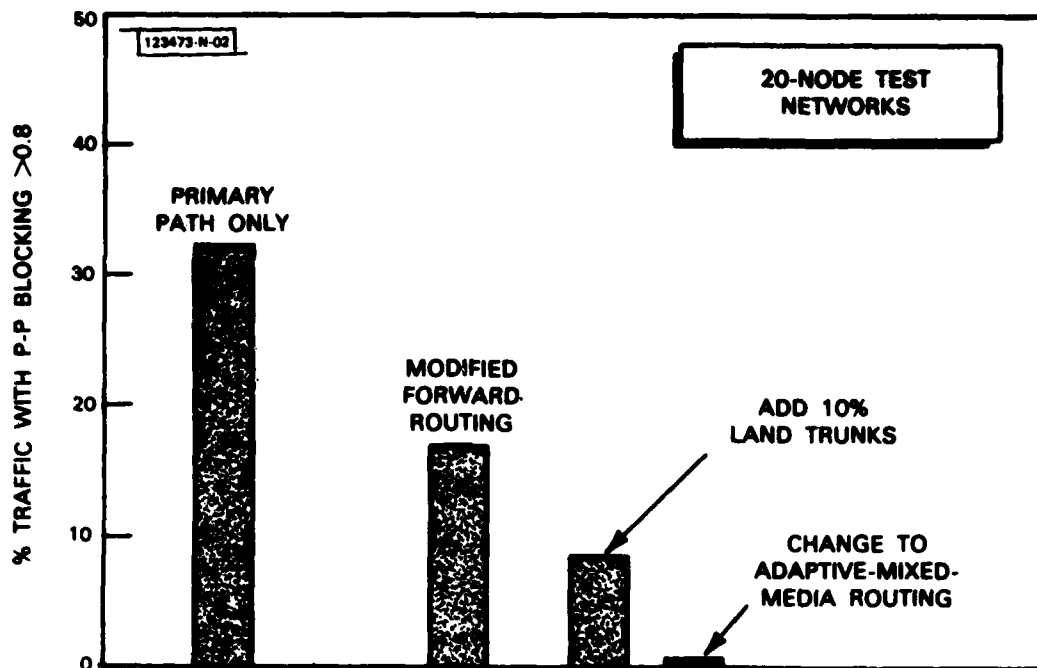
Fig. 9. Percentage offered traffic that experiences a point-to-point blocking probability > 0.8 when the satellite is destroyed (1) in network DSN1 with primary-path-only routing, (2) in network DSN1 with modified forward routing, (3) in network DSN3 which has 10-percent more land trunks than in DSN1 but still with modified forward routing, and (4) in network DSN1 with adaptive-mixed-media routing.
