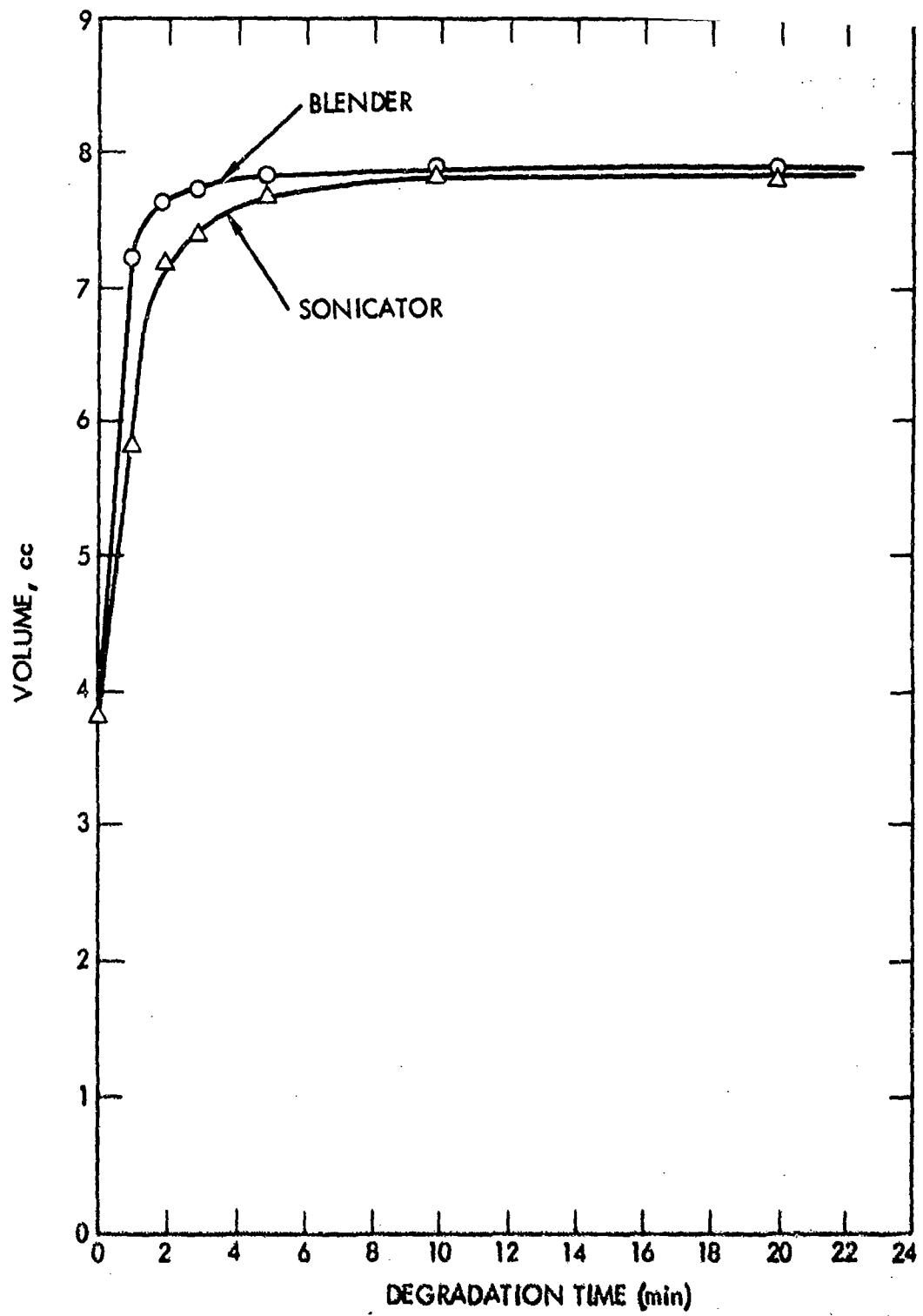
FIGURE 19 MONITORING OF DEGRADATION BY CUP TEST
