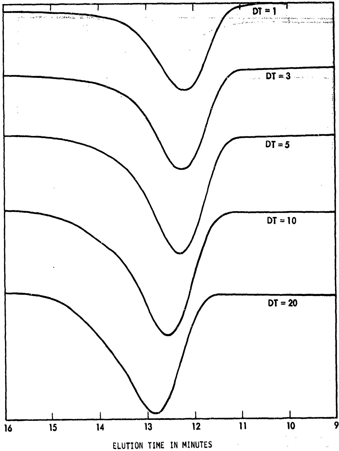
FIGURE 13 GEL PERMEATION CHROMATOGRAPHY (GPC) ULTRASONIC DEGRADATION, STYRAGEL COLUMNS 10^5 , 10^4 , 10^3 , 500A. DT-DEGRADATION TIME IN MINUTES.
