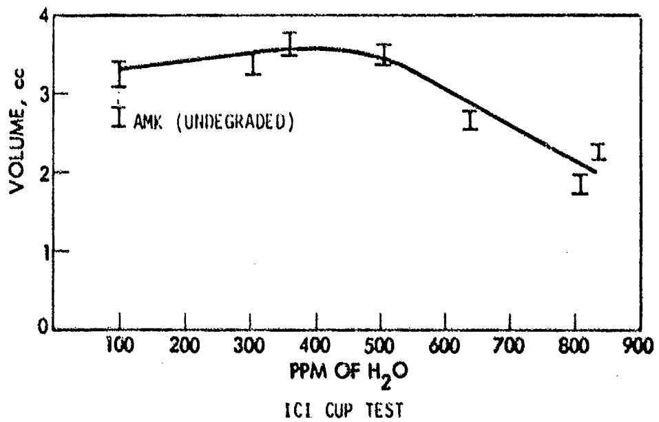
FIGURE 17 INFLUENCE OF WATER ON FILTER AND CUP TESTS
