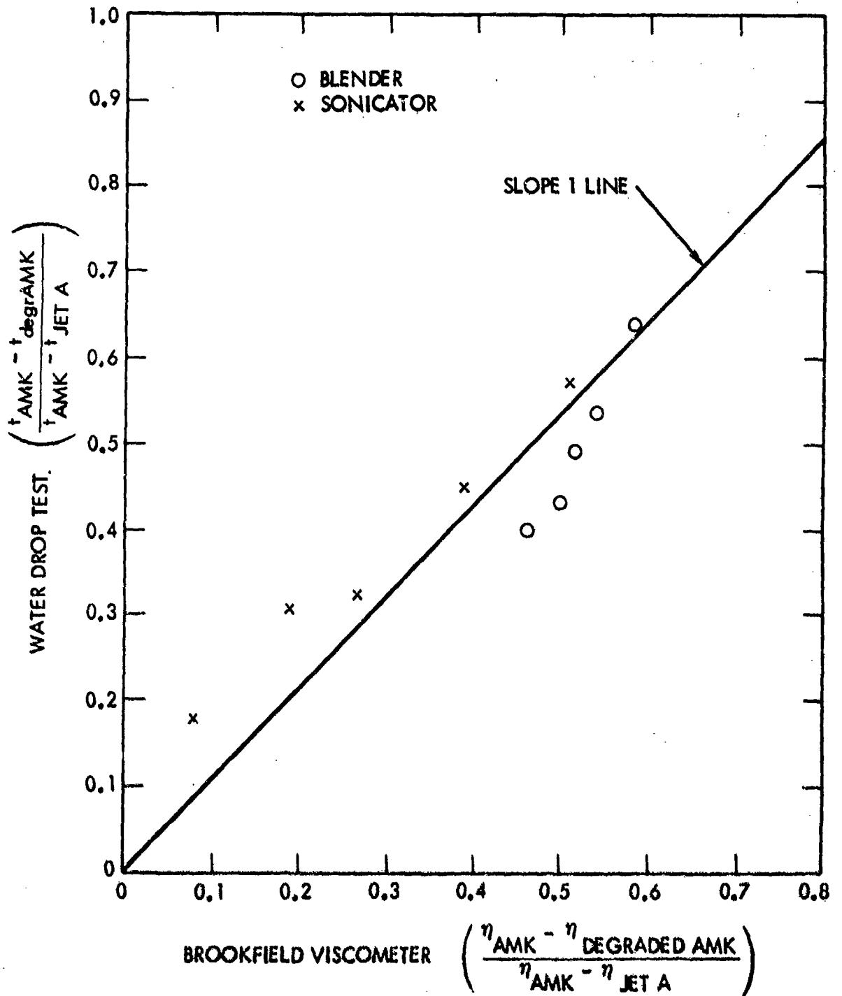
FIGURE 22 CORRELATION BETWEEN WATER-DROPLET TEST AND VISCOMETRY
