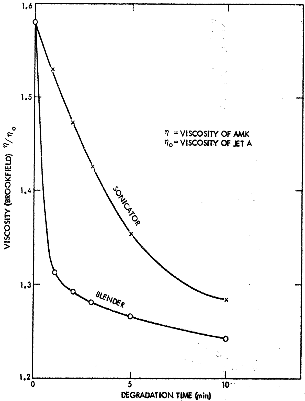
FIGURE 20 MONITORING OF DEGRADATION BY BROOKFIELD VISCOMETER
