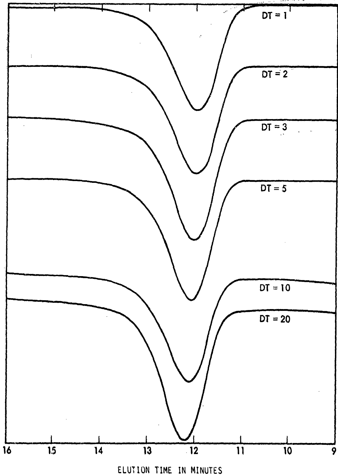
FIGURE 14. GEL PERMEATION CHROMATOGRAPHY DEGRADATION IN BLENDER. STYRAGEL COLUMNS 10^5 , 10^4 , 10^3 , 500Å. DT - DEGRADATION TIME IN MINUTES.
