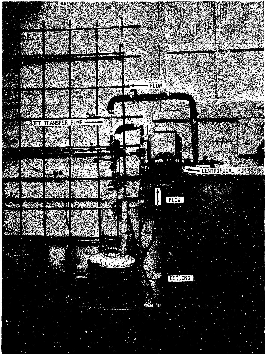
FIGURE 11 FUEL SYSTEM SETUP
