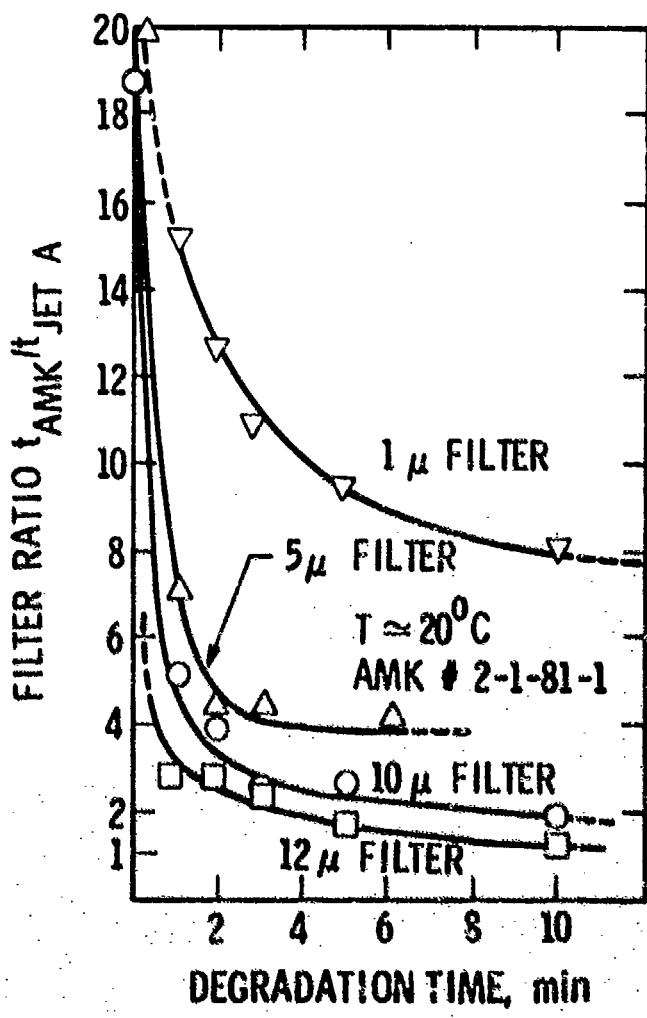
FIGURE 25 EFFECTIVENESS OF DEGRADATION MONITORING OF VARIOUS PORE SIZE FILTERS
