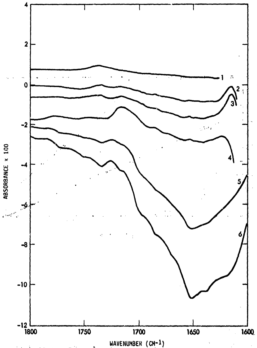
FIGURE 3 SPECTRA OF WATER-TREATED AMK WITH THE REFERENCE SPECTRUM OF UNTREATED AMK SUBTRACTED (WATER DATA) THE NUMBERS 1 THROUGH 6 REPRESENT THE SAMPLE NUMBERS CITED IN TABLE 1
