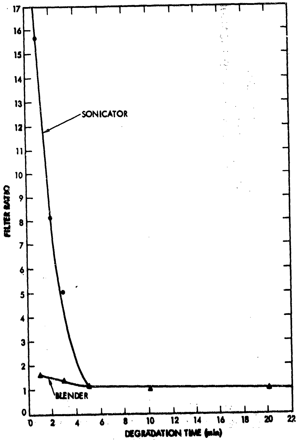
FIGURE 15 MONITORING OF DEGRADATION BY FILTER TEST USING 16-18 \mu STAINLESS STEEL FILTER
