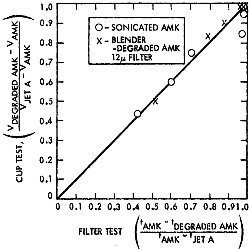
FIGURE 24 CORRELATION BETWEEN THE CUP AND FILTER TESTS FOR DEGRADED AMK
