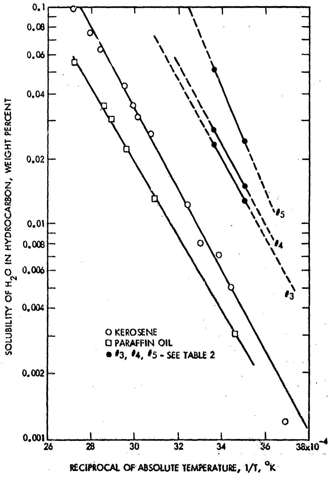
FIGURE 6 SOLUBILITY OF WATER IN PETROLEUM FRACTIONS AS A FUNCTION OF TEMPERATURE (REFERENCE 5)
