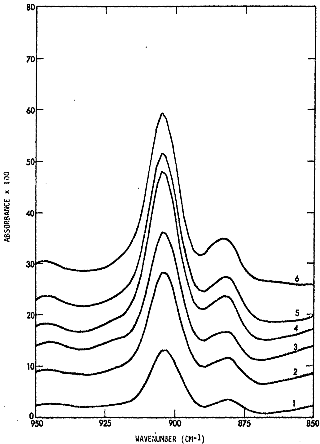
FIGURE 2 SPECTRA OF WATER-TREATED AMK WITH THE REFERENCE SPECTRUM OF UNTREATED AMK SUBTRACTED (GLYCOL DATA) THE NUMBERS 1 THROUGH 6 REPRESENT THE SAMPLE NUMBERS CITED IN TABLE 1
