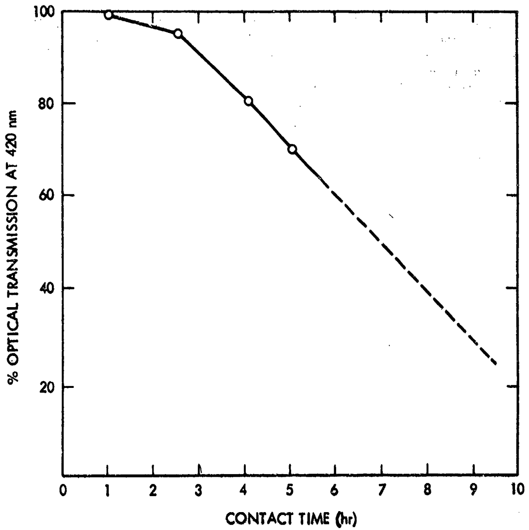
FIGURE 10 OPTICAL TRANSMISSION VS. WATER/FUEL CONTACT TIME
