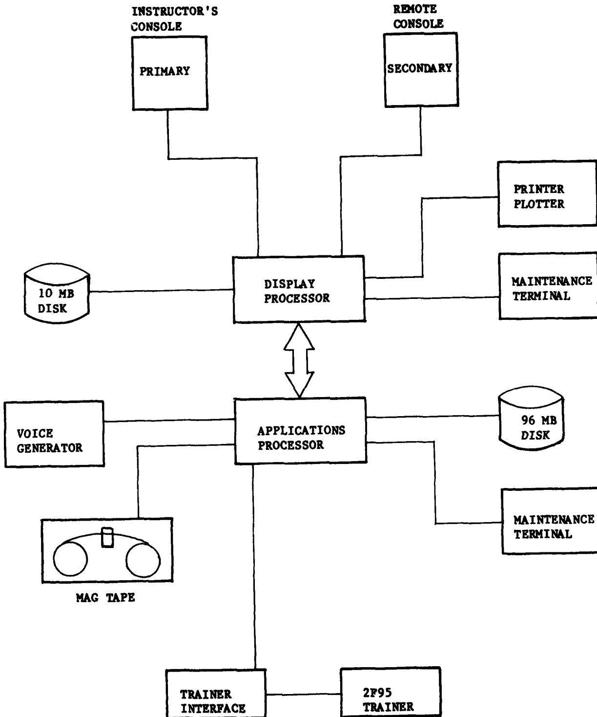
Figure 1. ISS System Block Diagram.
